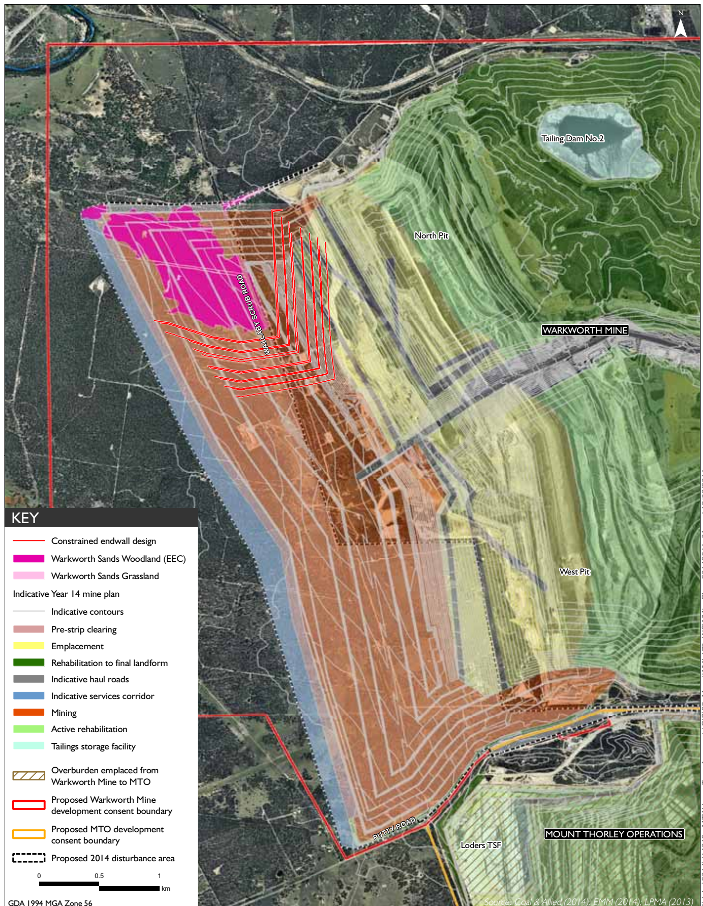
Constrained endwall design and reduced strike length Warkworth Continuation 2014 Environmental Impact Statement Figure 23.1
