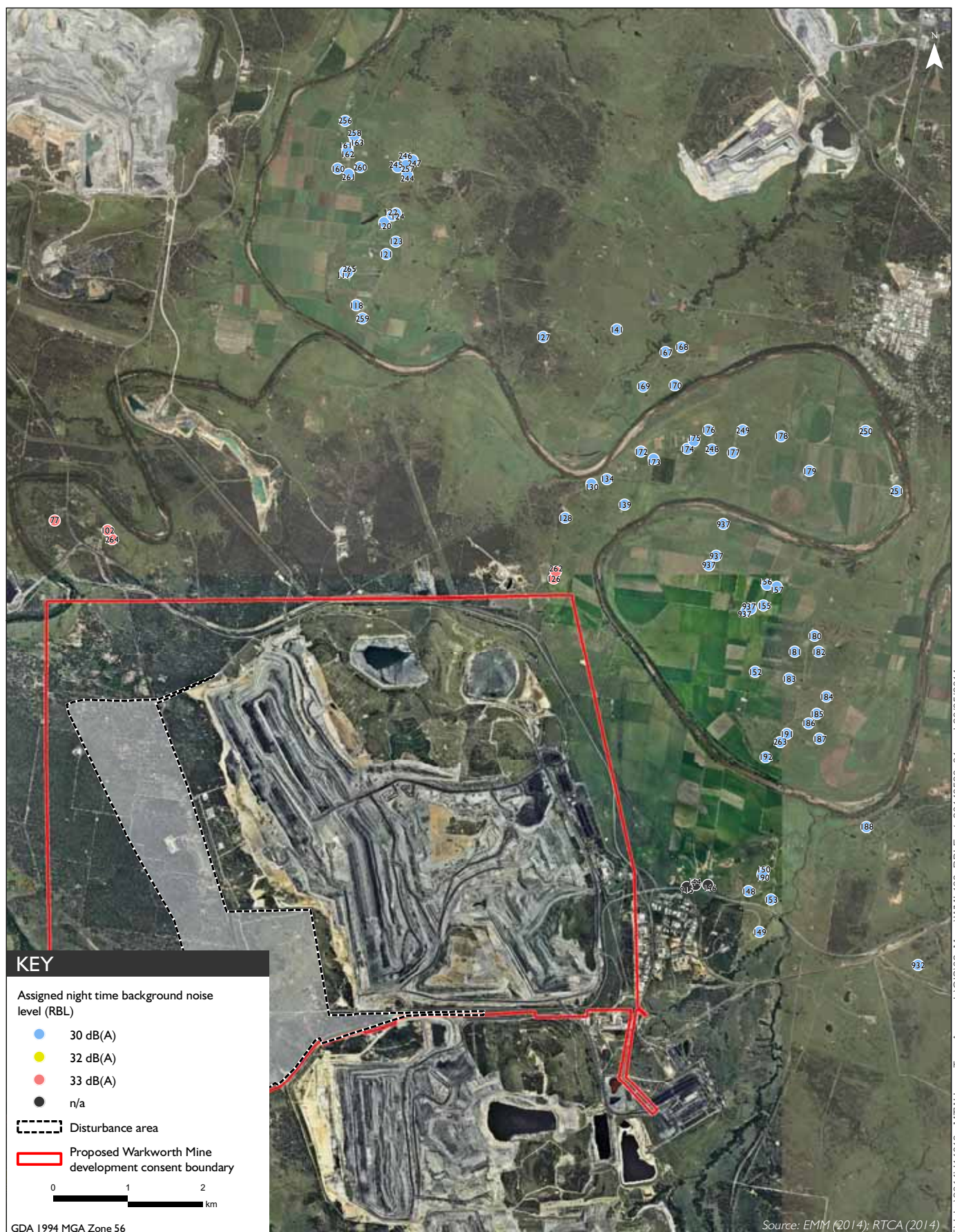
Assigned night time background noise levels - Eastern and northern assessment locations Warkworth Continuation 2014 Environmental Impact Statement Figure 10.4
