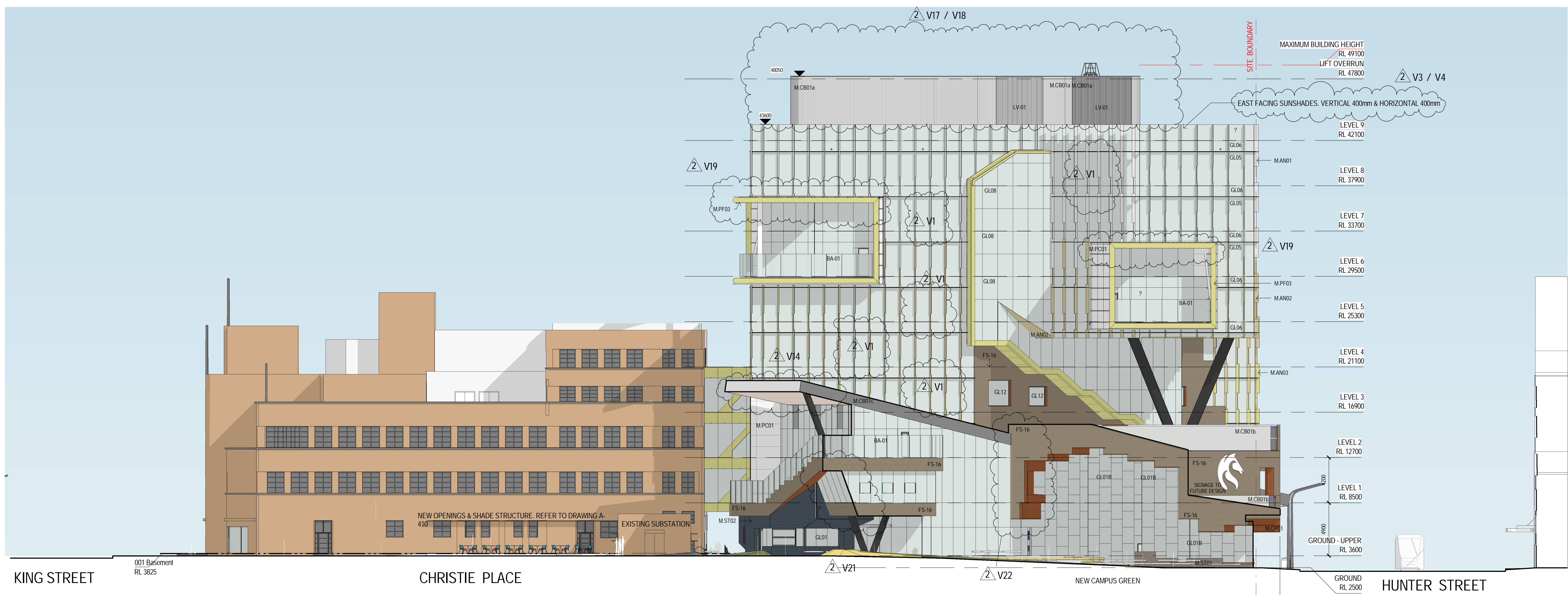
2 ELEVATION - EAST (CHRISTIE PLACE) Scale: 1: 200
