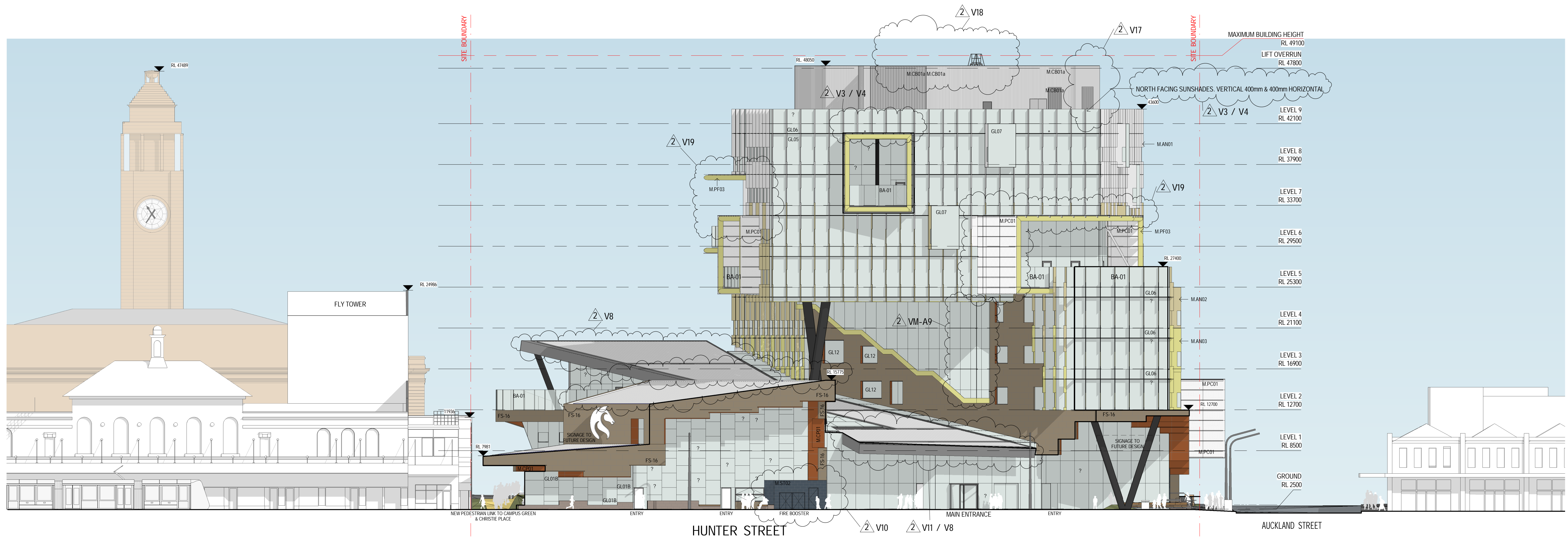
1 ELEVATION - NORTH (HUNTER STREET) Scale: 1 : 200
