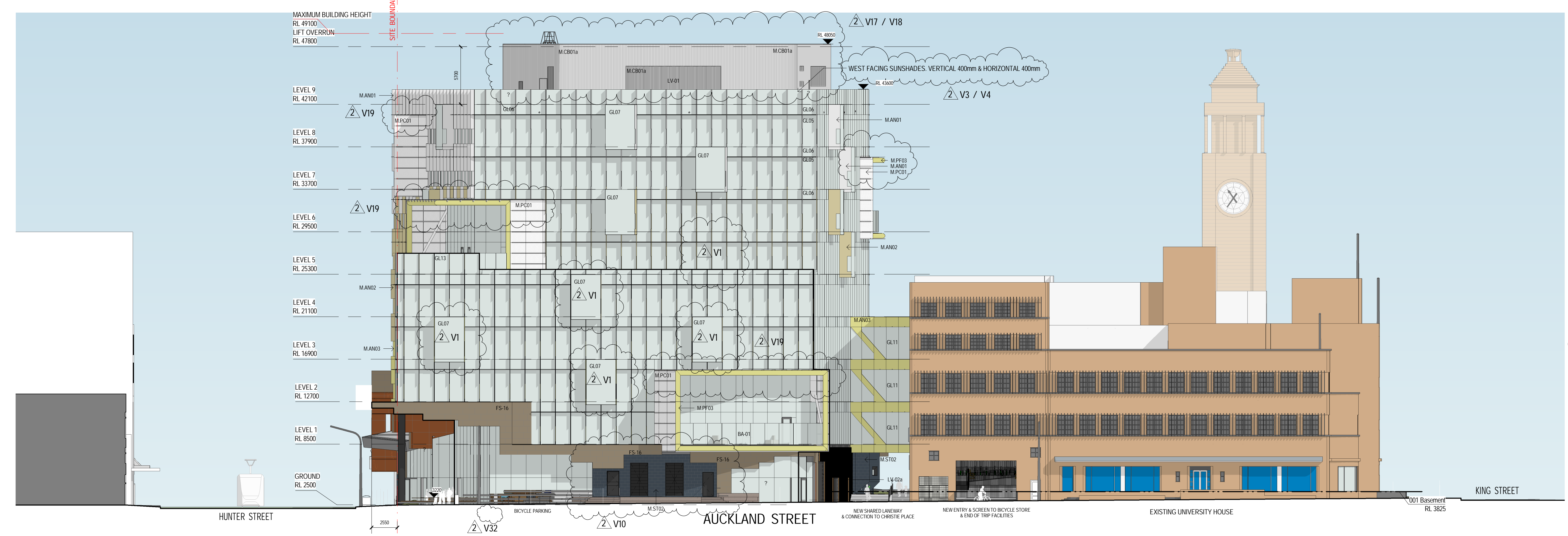
2 ELEVATION - WEST (AUCKLAND STREET) Scale: 1 : 200
