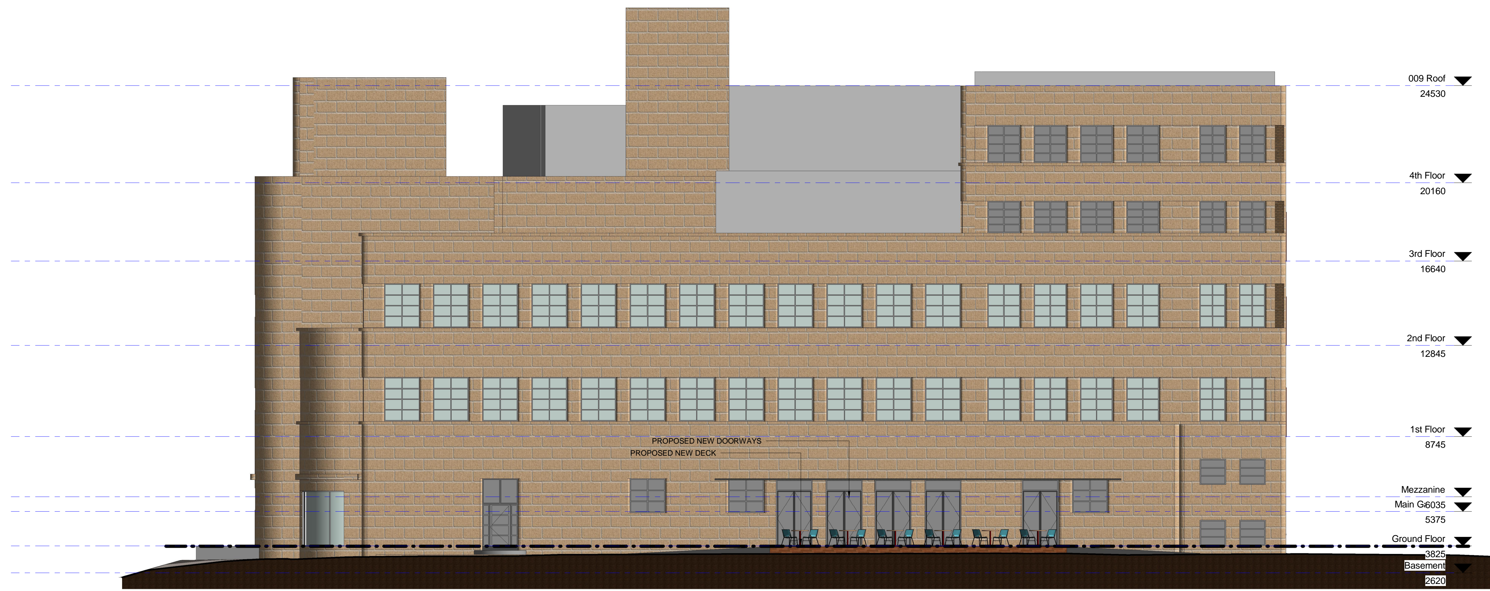
East Elevation 1 : 100
