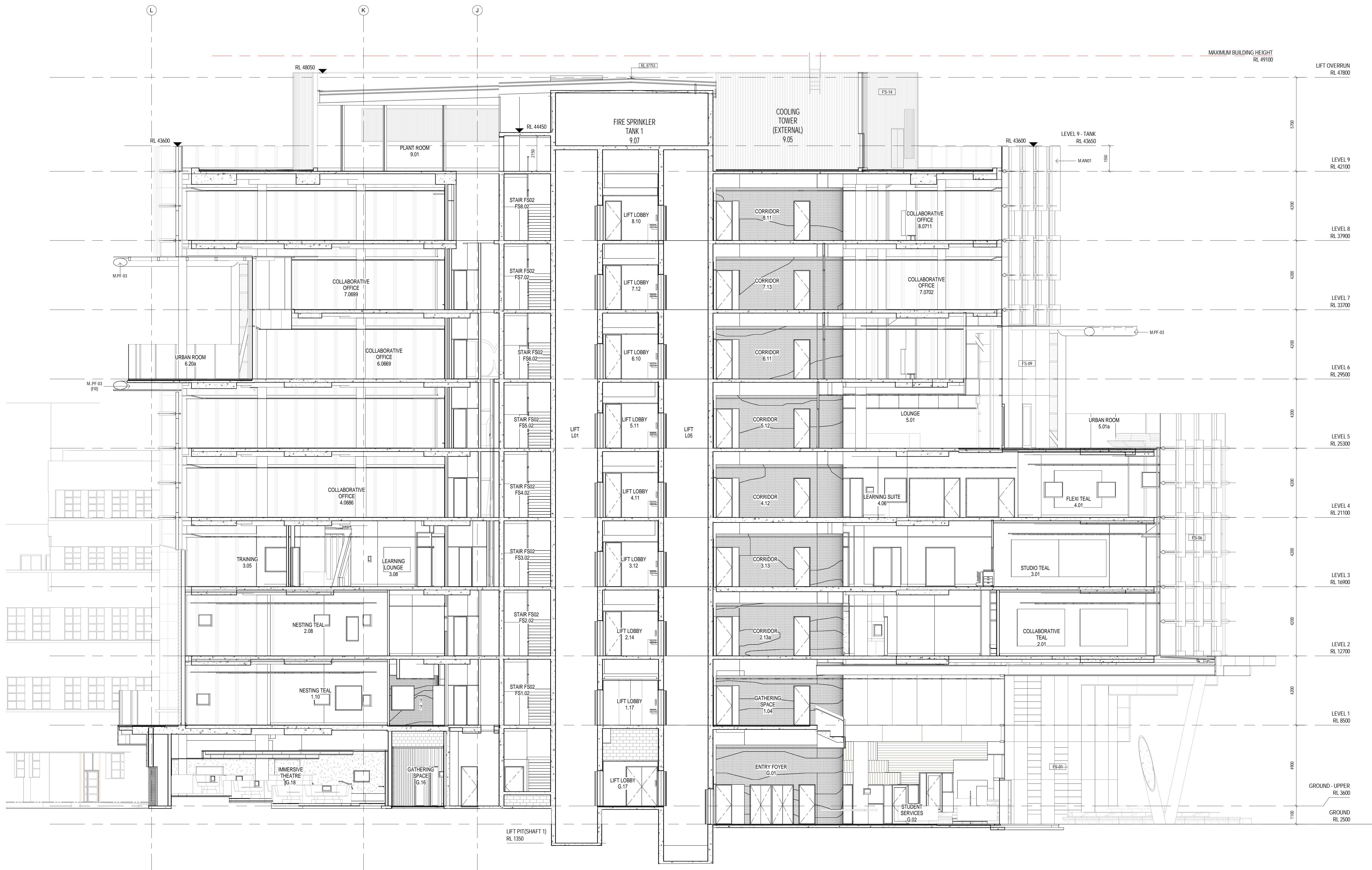
C SECTION CC A 300 Scale 1: 100
