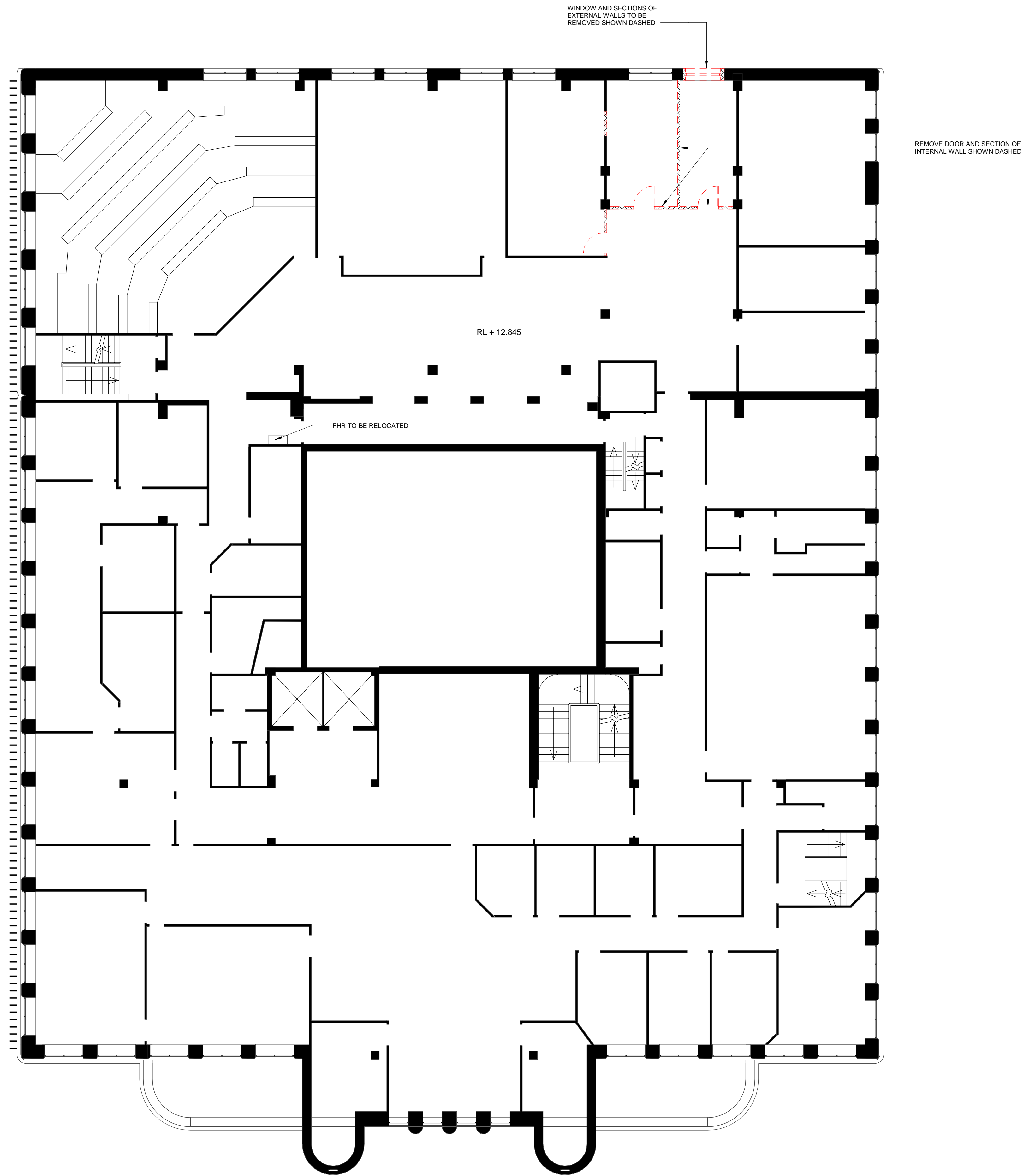
1 Demolition Plan - 2nd Floor 1 : 100
