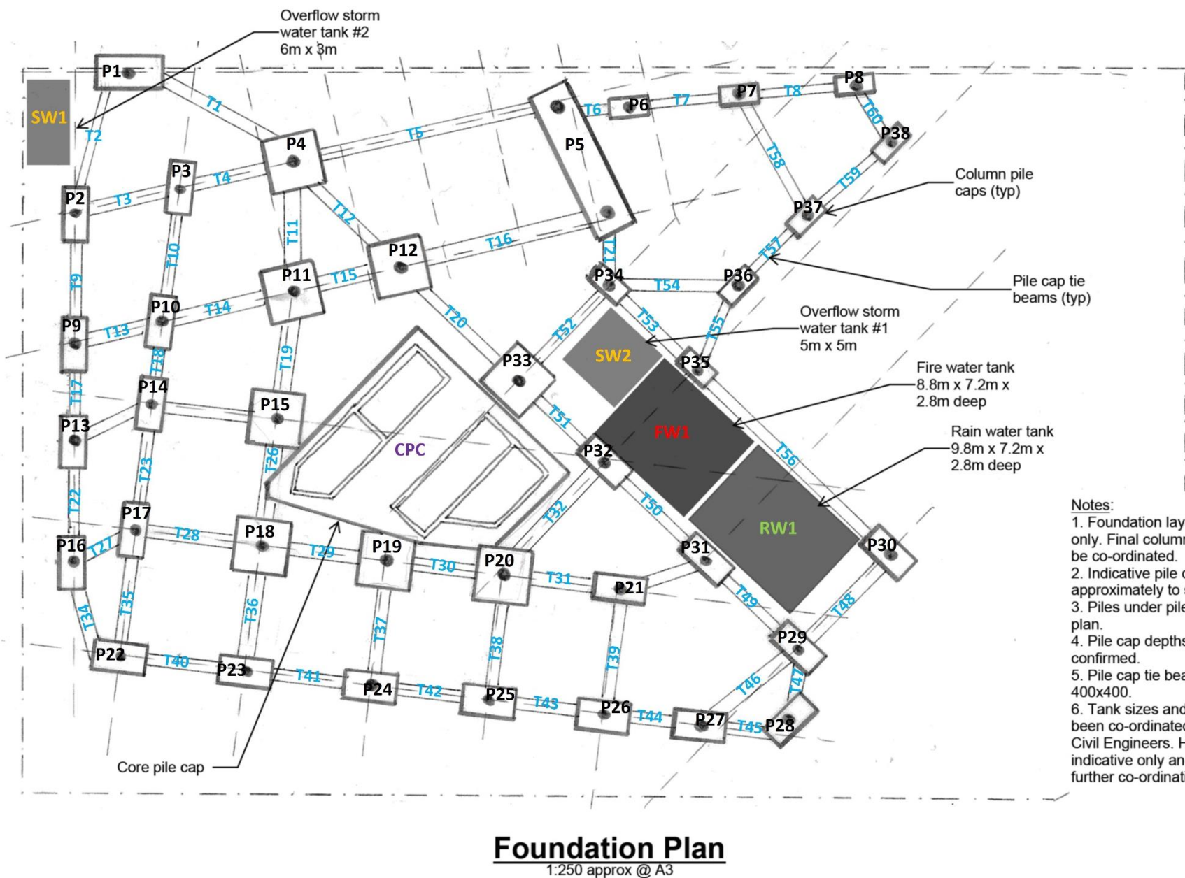
Figure 1 Foundation plan, showing the numbering system for each impact feature.
