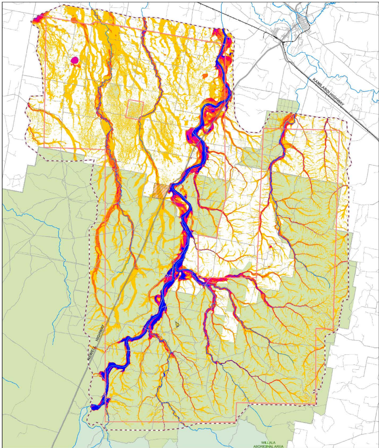
Figure 10: Flooding 1% AEP Event
