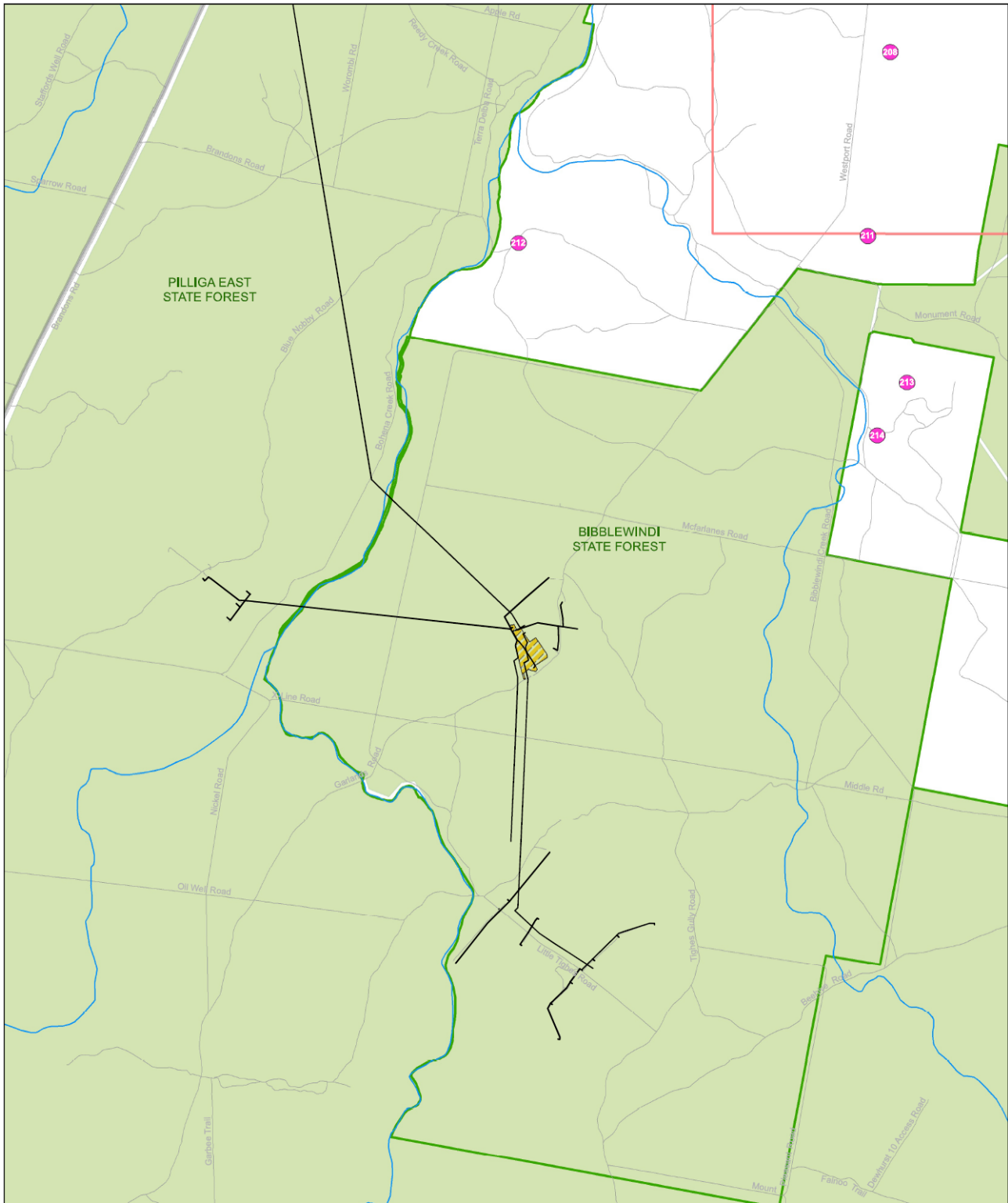
Figure 7: Receiver Locations – Bibblewindi
