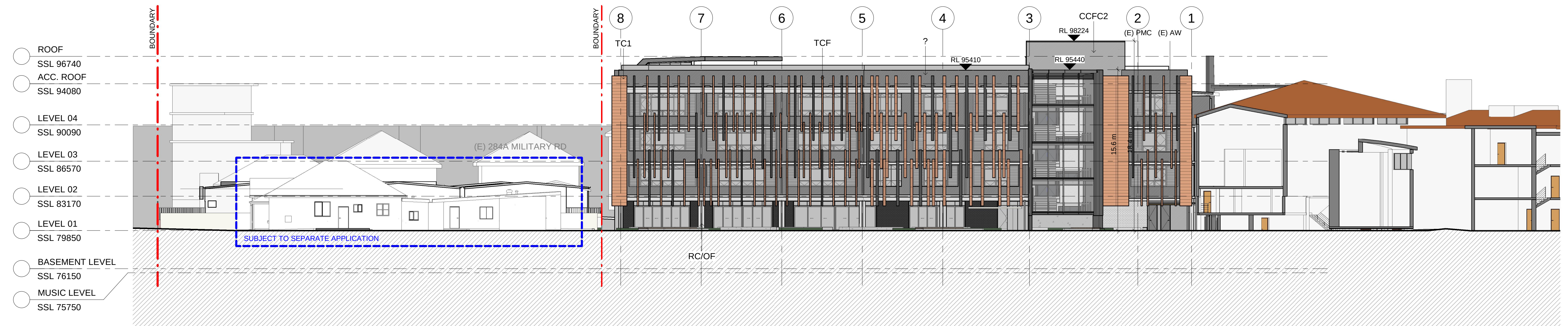
2 NORTH ELEVATION 1 : 200
