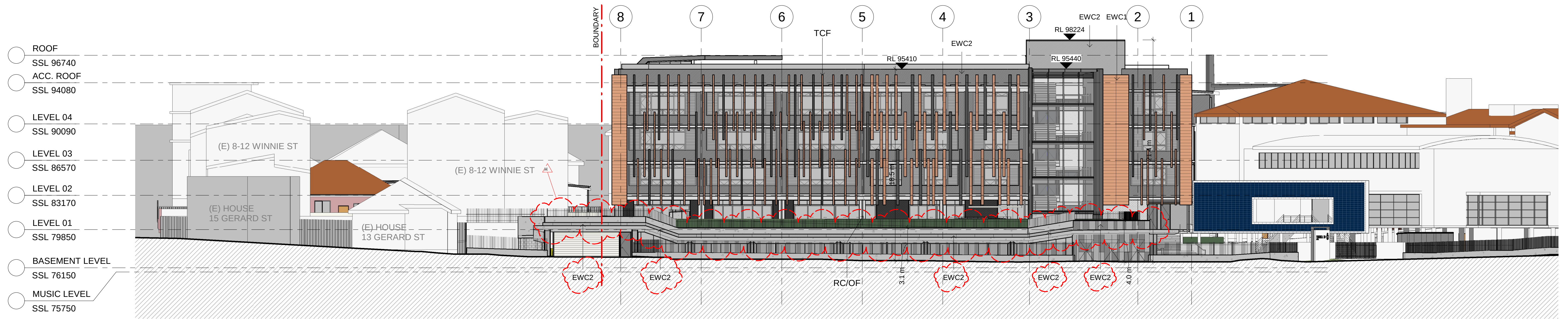
1 NORTH ELEVATION - GERARD STREET 1 : 200
