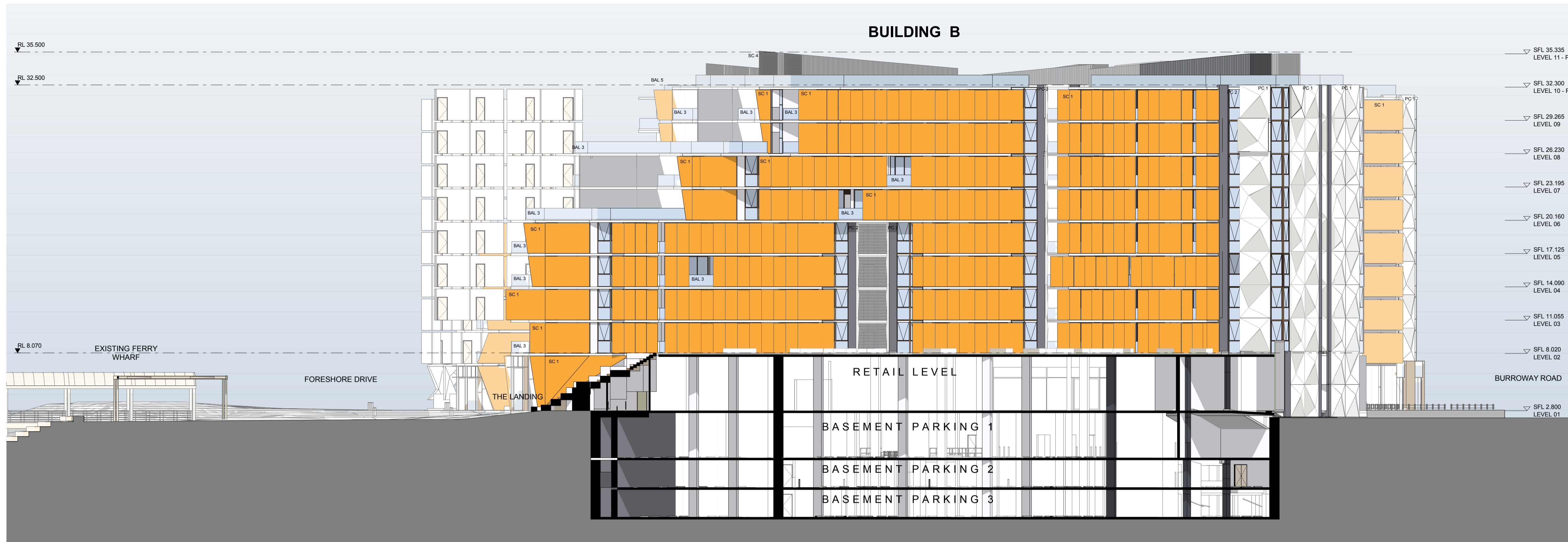
1 ELEVATION B-B WEST ELEVATION 1:200
