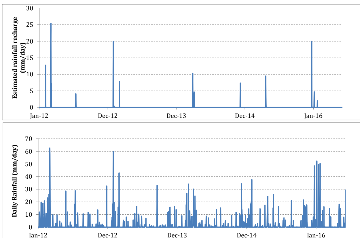
Figure 5-7 Daily rainfall and estimated rainfall recharge events
