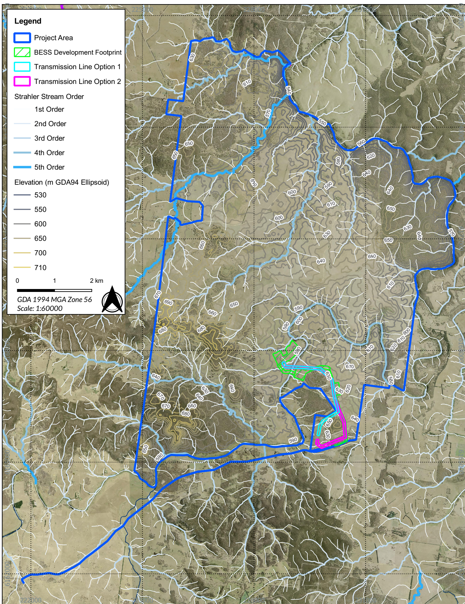
Figure 3.2 - Hydrology and topography of the Project Area
