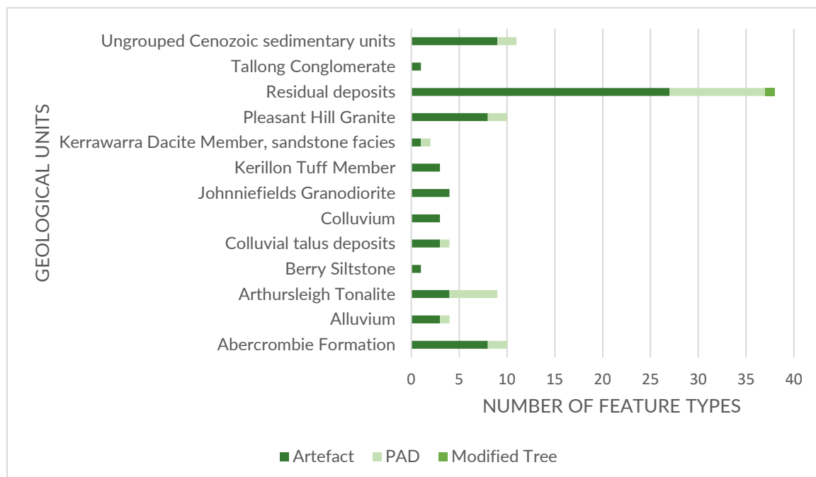
Figure 5.3 Recorded feature types and distribution by geological unit
