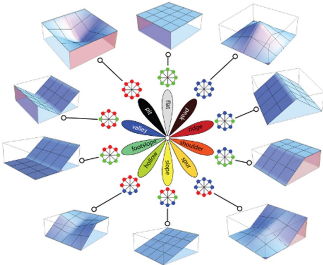
Figure 5.7 Examples of landform definitions by geomorphons
