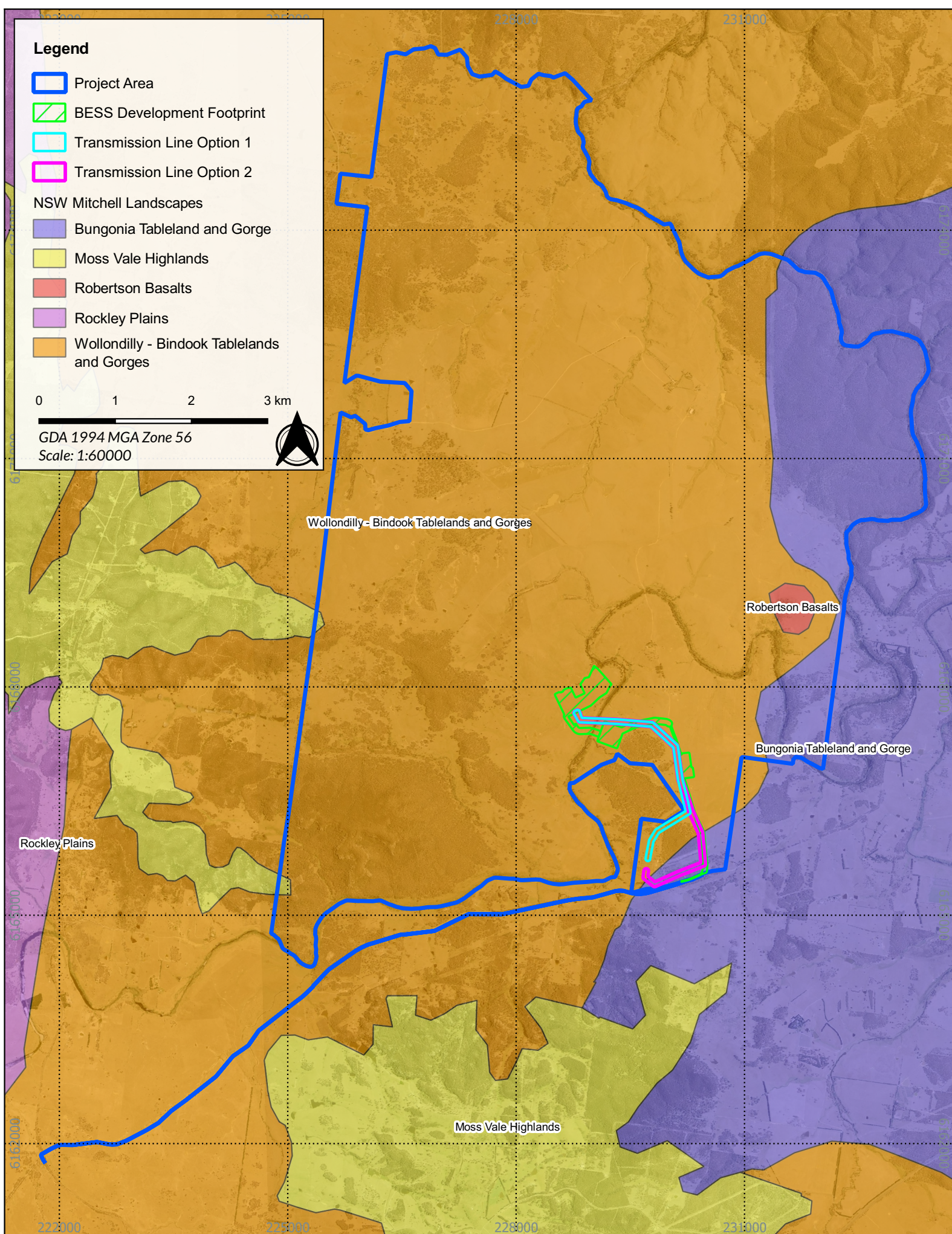
Figure 3.4 - Mitchell Landscapes identified within the Project Area and surrounding landscape
