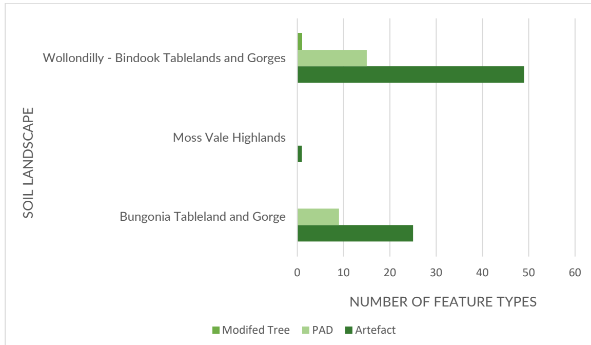
Figure 5.1 Recorded feature type distribution by soil landscape
