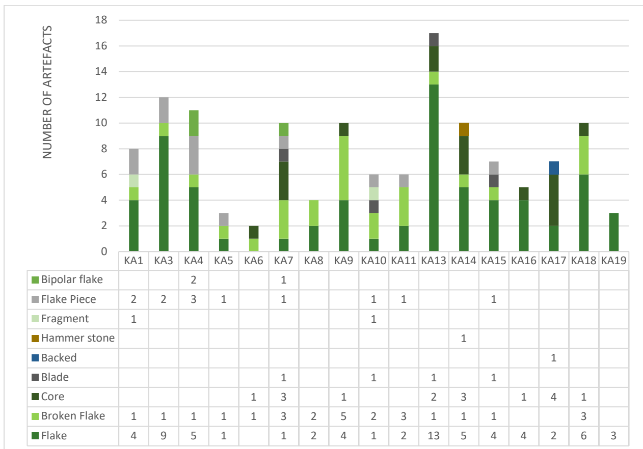
Figure 5.9 Artefact types from the Navin Officer assemblage
