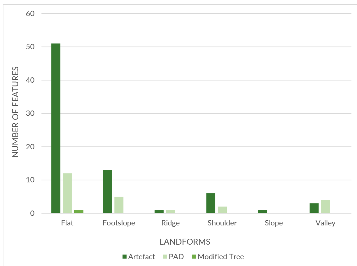
Figure 5.8 Number of feature types by landform
