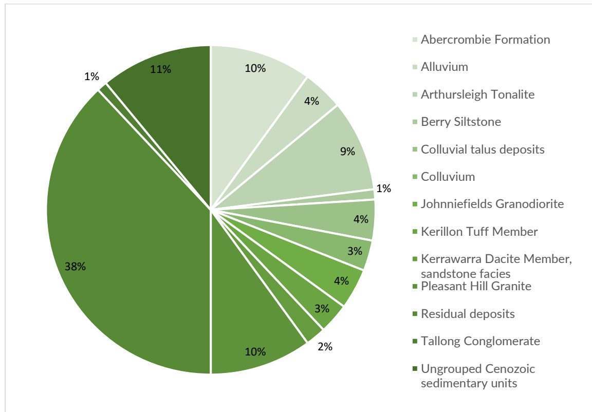
Figure 5.4 Frequency of recorded feature types by geological unit
