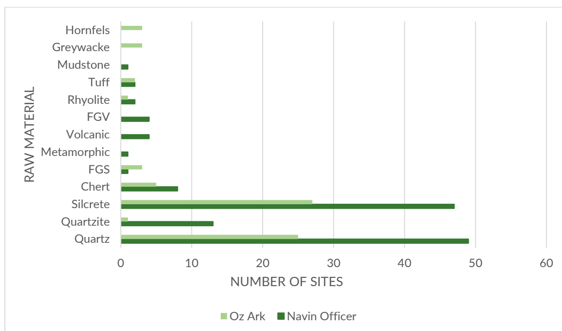
Figure 5.12 Raw material types from locally excavated assemblages
