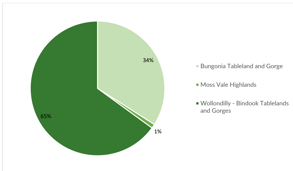
Figure 5.2 Frequency of recorded feature type by soil landscape
