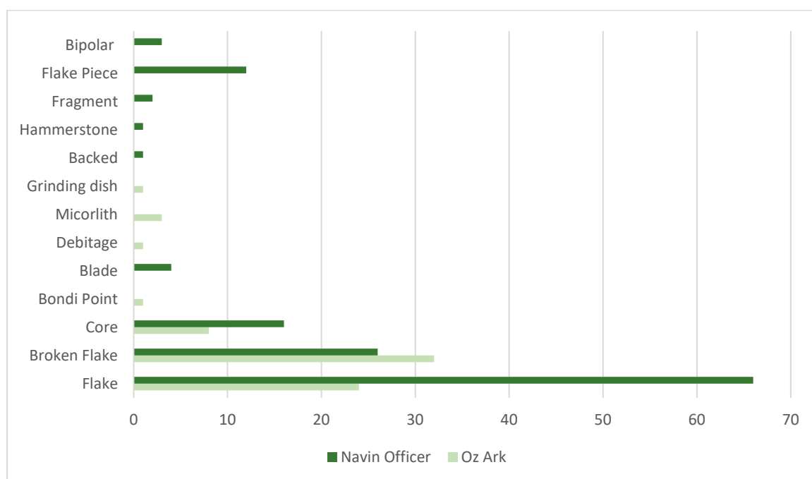
Figure 5.10 Artefact types combined OzArk and Navin Officer assemblages
