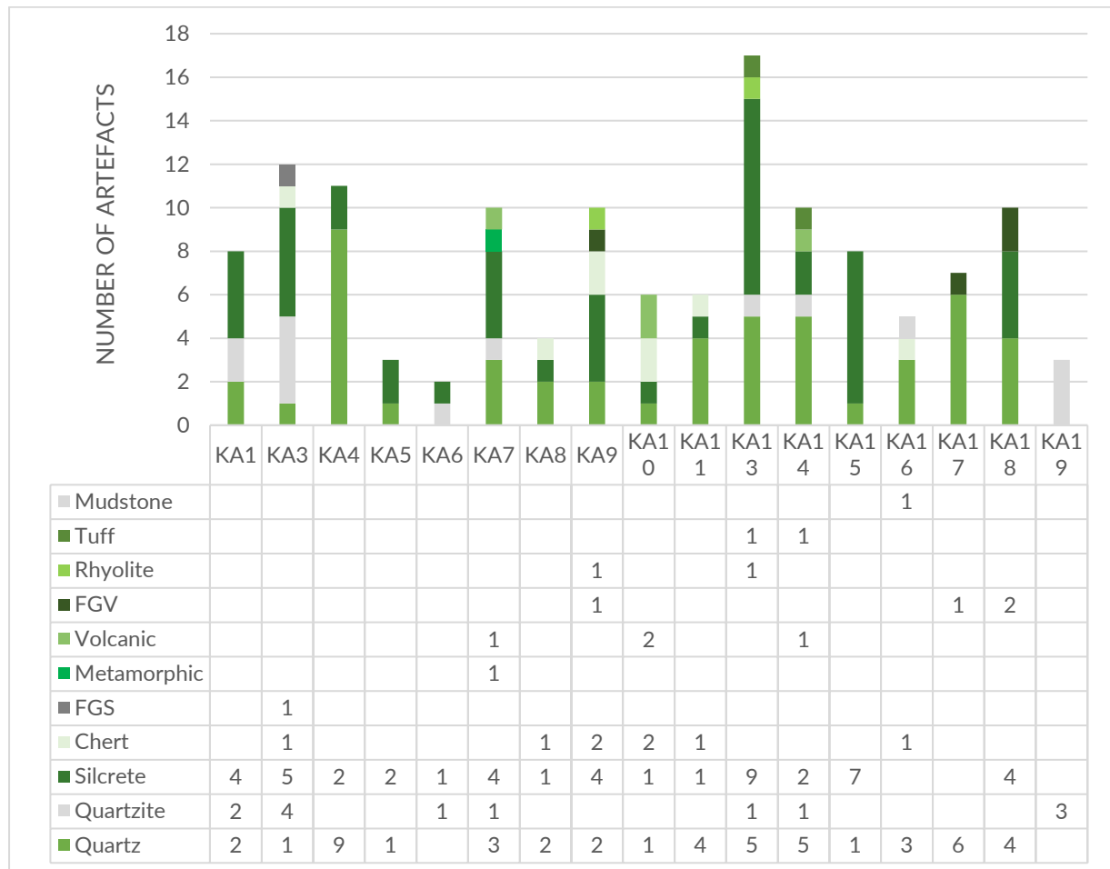
Figure 5.11 Raw material types from Navin Officer assemblage
