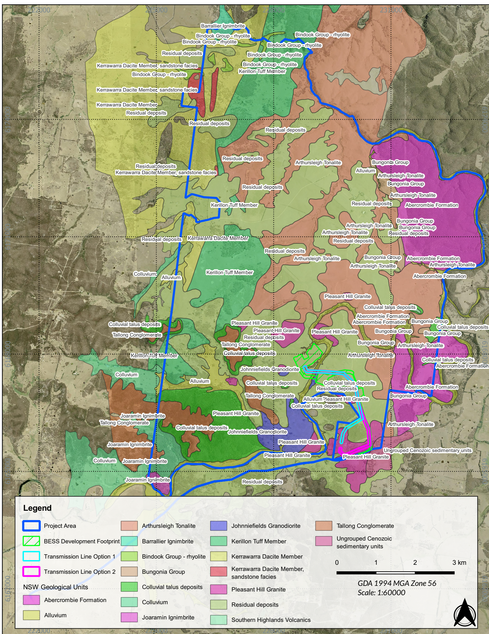
Figure 3.3 - Geology of the Project Area
