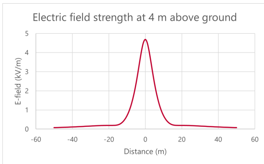
Figure 11: Electric Field strength of 330 kV Overhead Transmission lines with a ground clearance of 8.5 m
