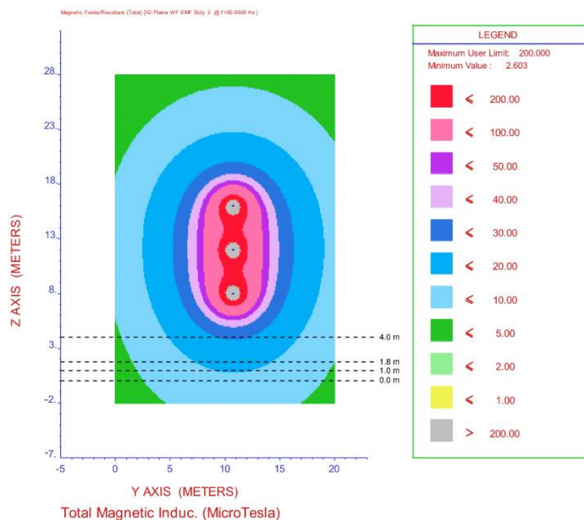
Figure 9: Magnetic Field strength of 330 kV overhead transmission lines carrying 658.4 A
