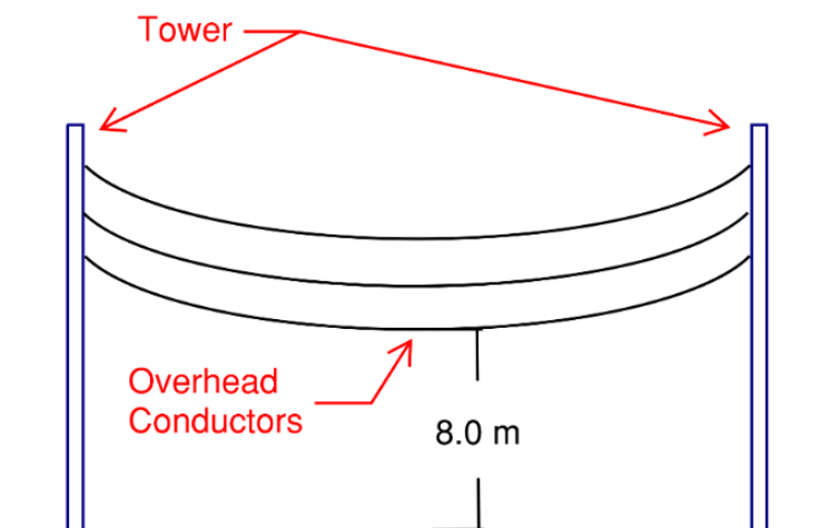
Figure 7: 330 kV Transmission Lines
