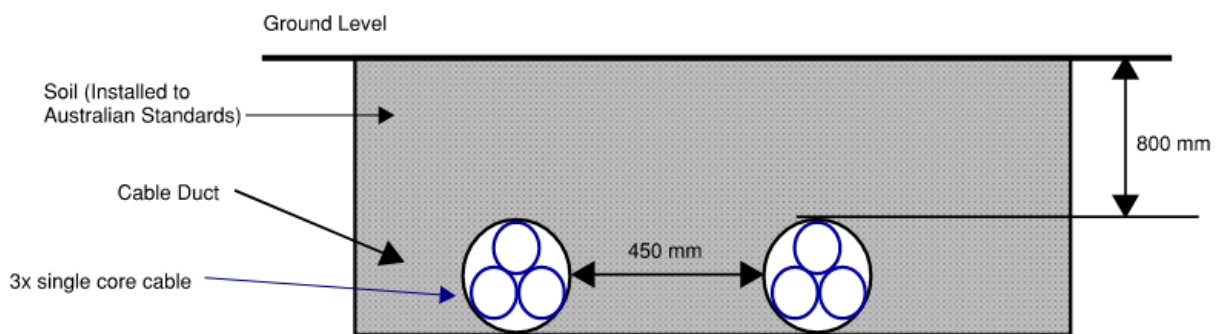
Figure 5: Underground Cable Installation Concept Design
