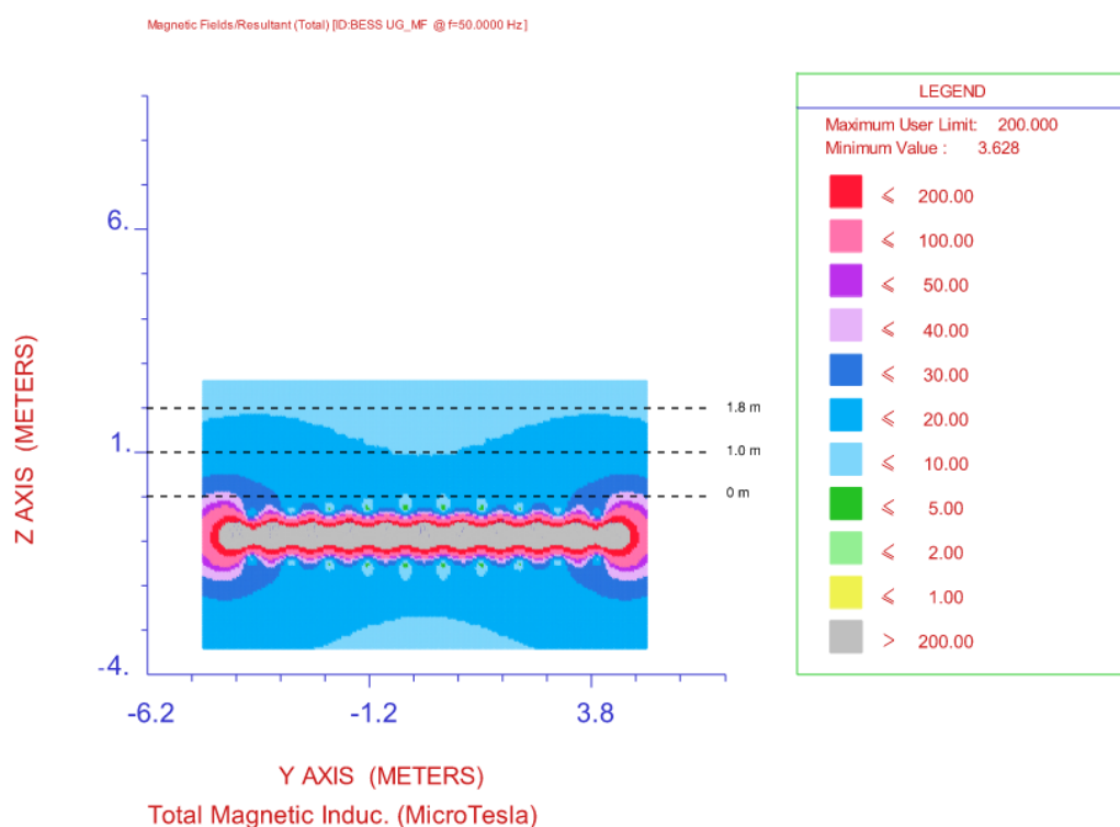
Figure 8: Magnetic Field Strength of 33 kV Underground Cables Carrying 598.5 A
