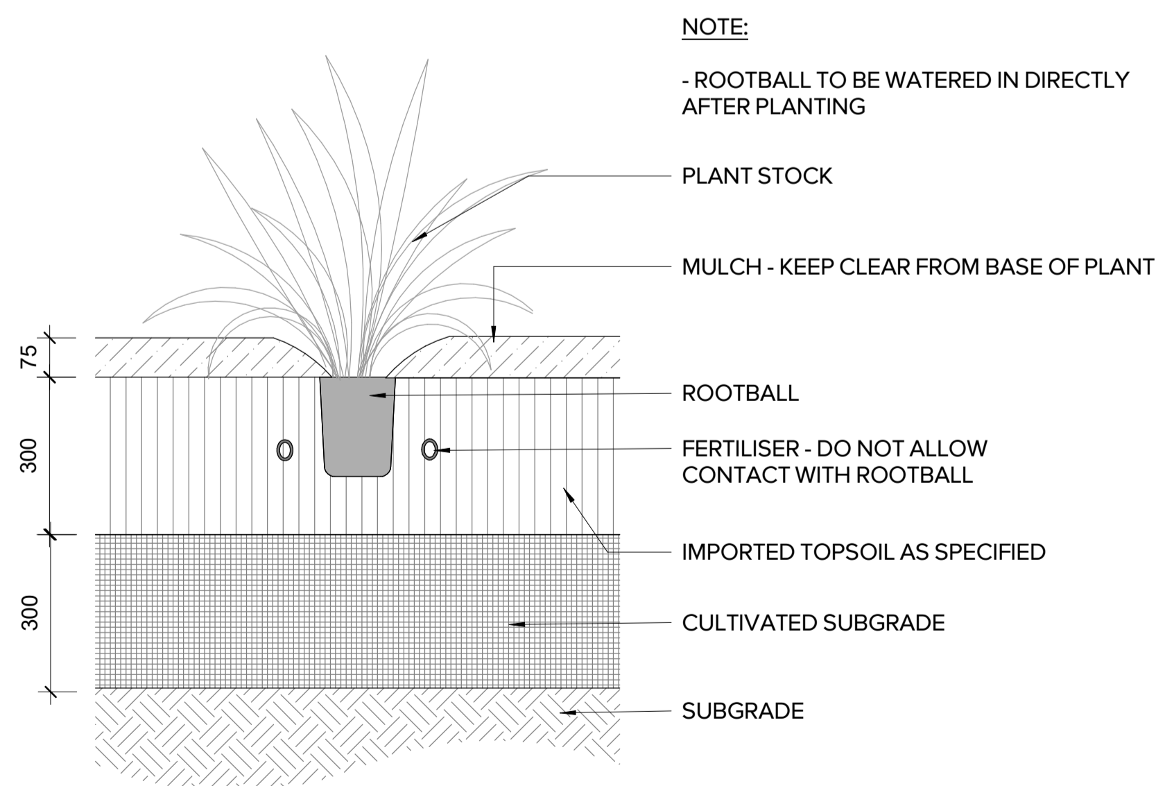
3 PLANTING - SHRUB 1 : 10
