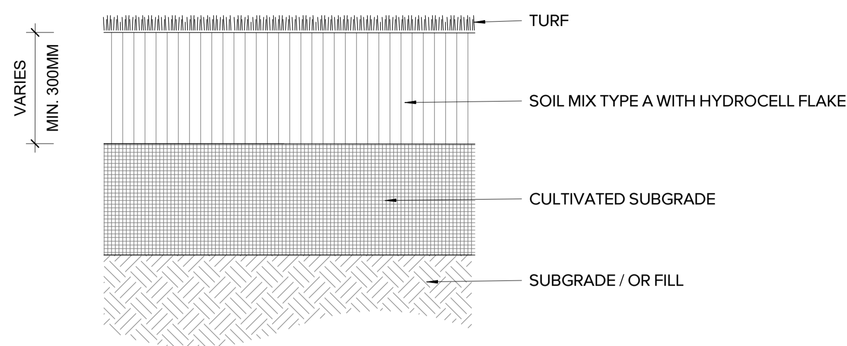
1 TURF - ON GRADE 1 : 10
