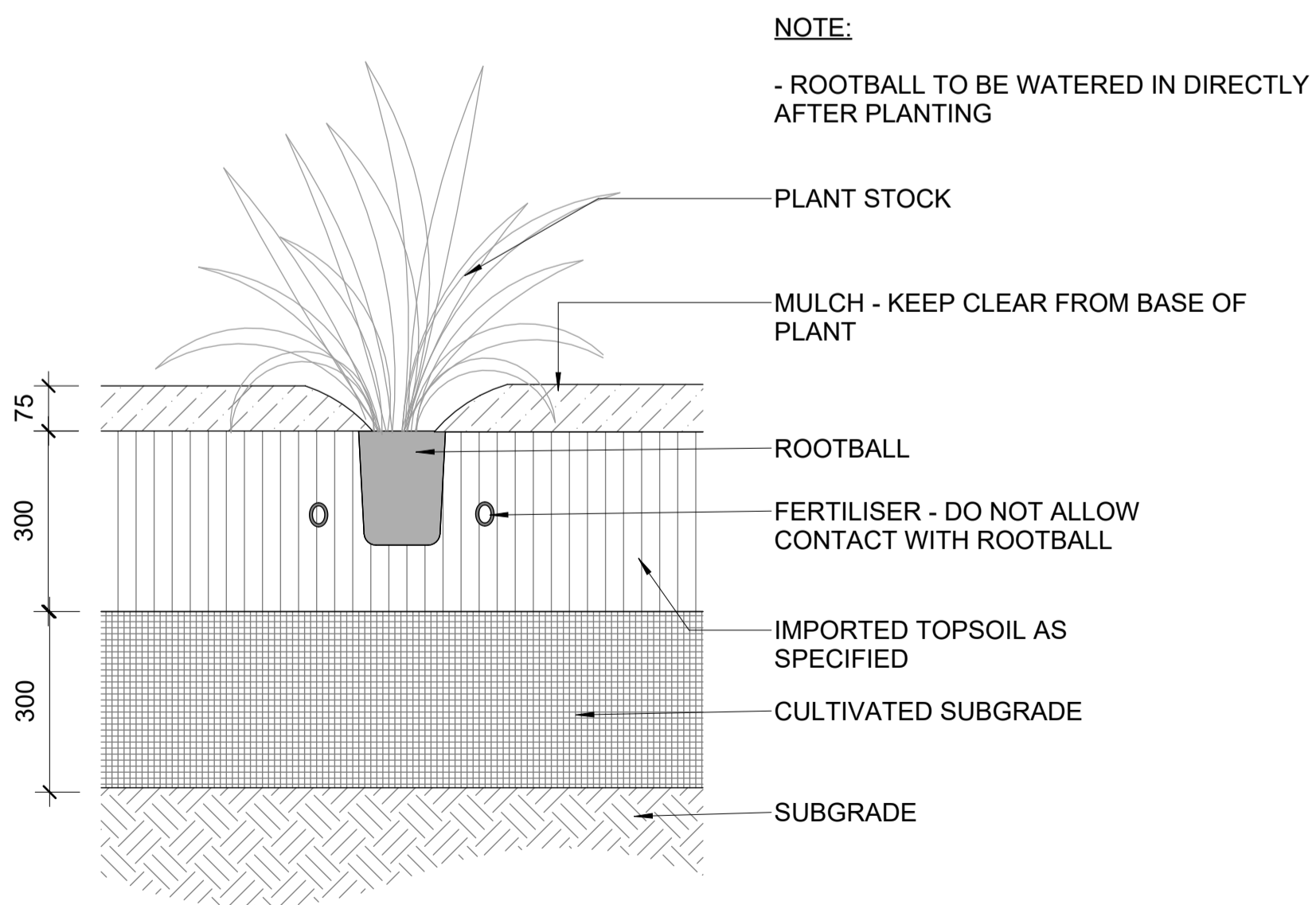
3 PLANTING - SHRUB 1 : 10
