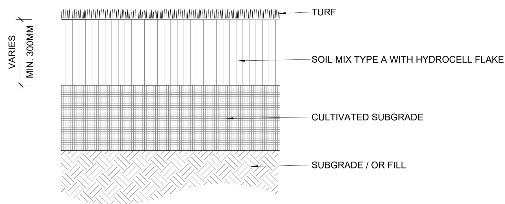
1 TURF - ON GRADE 1 : 10
