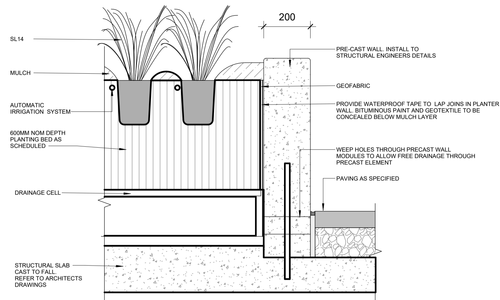
4 PLANTING - INSITU CONCRETE WALL 1 : 10
