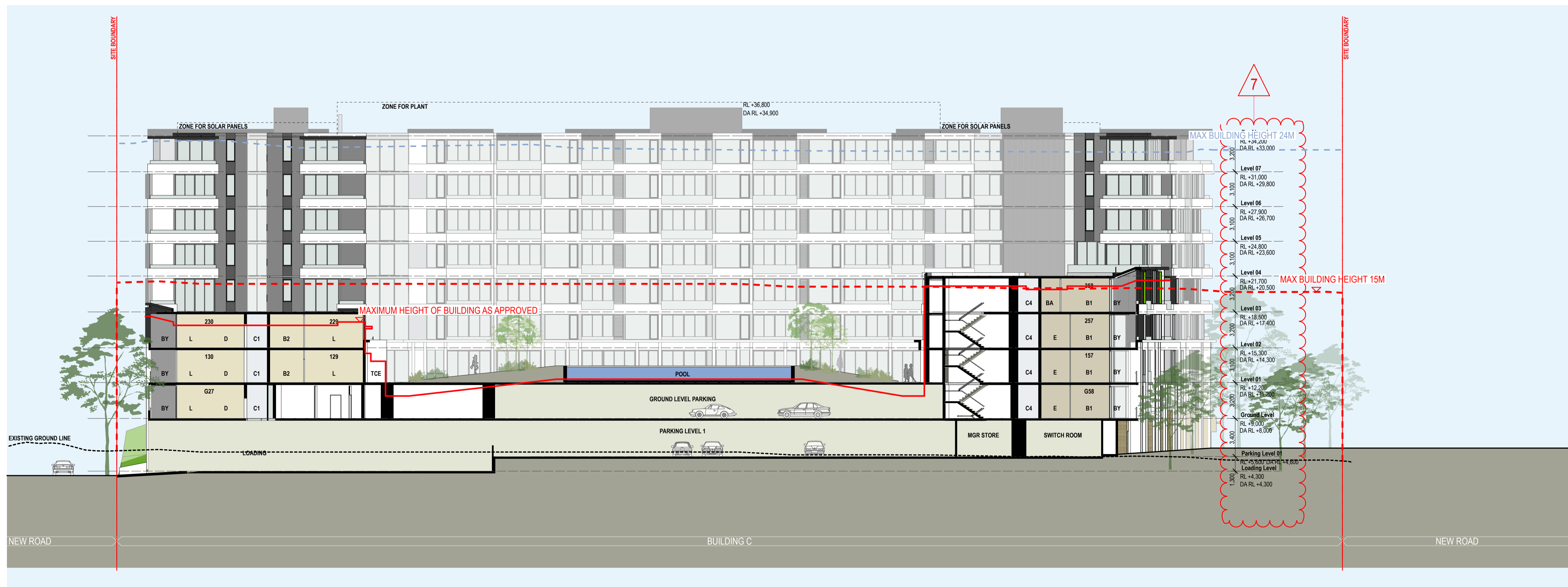
2 Section B 1:200
