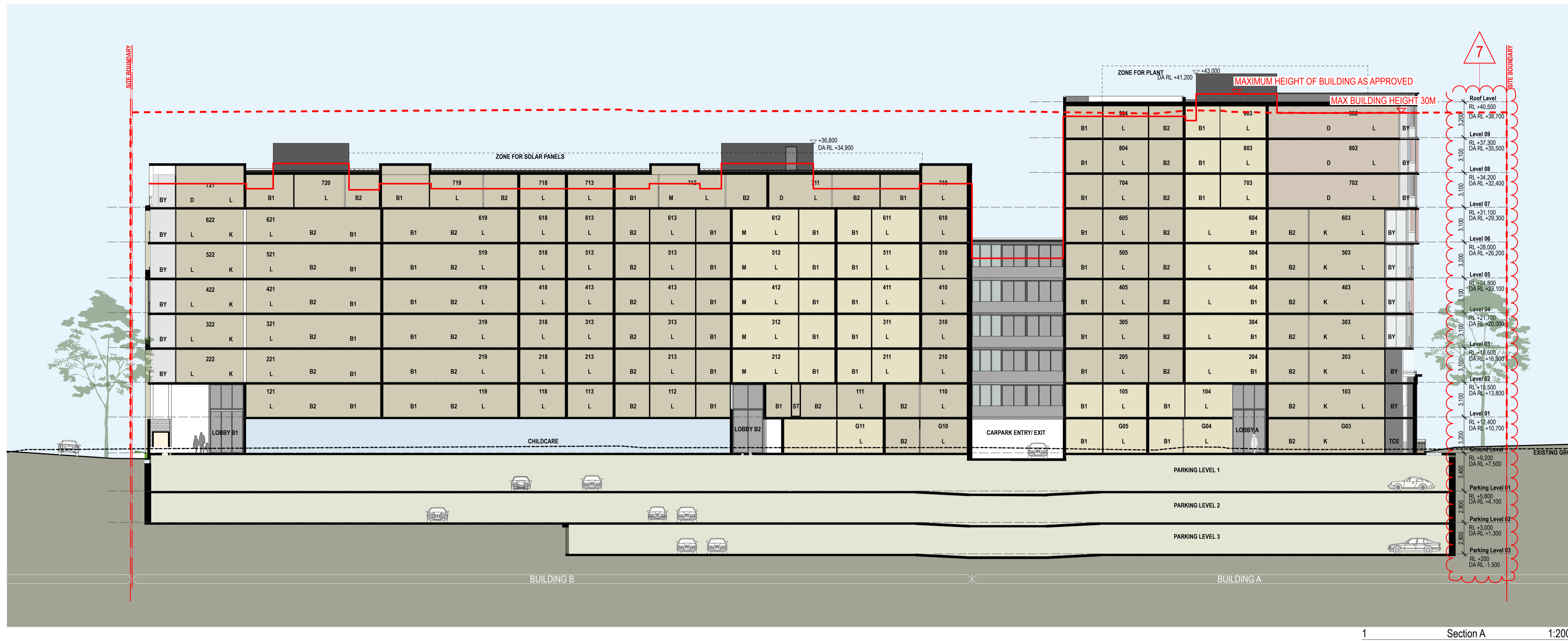
1 Section A 1:200
