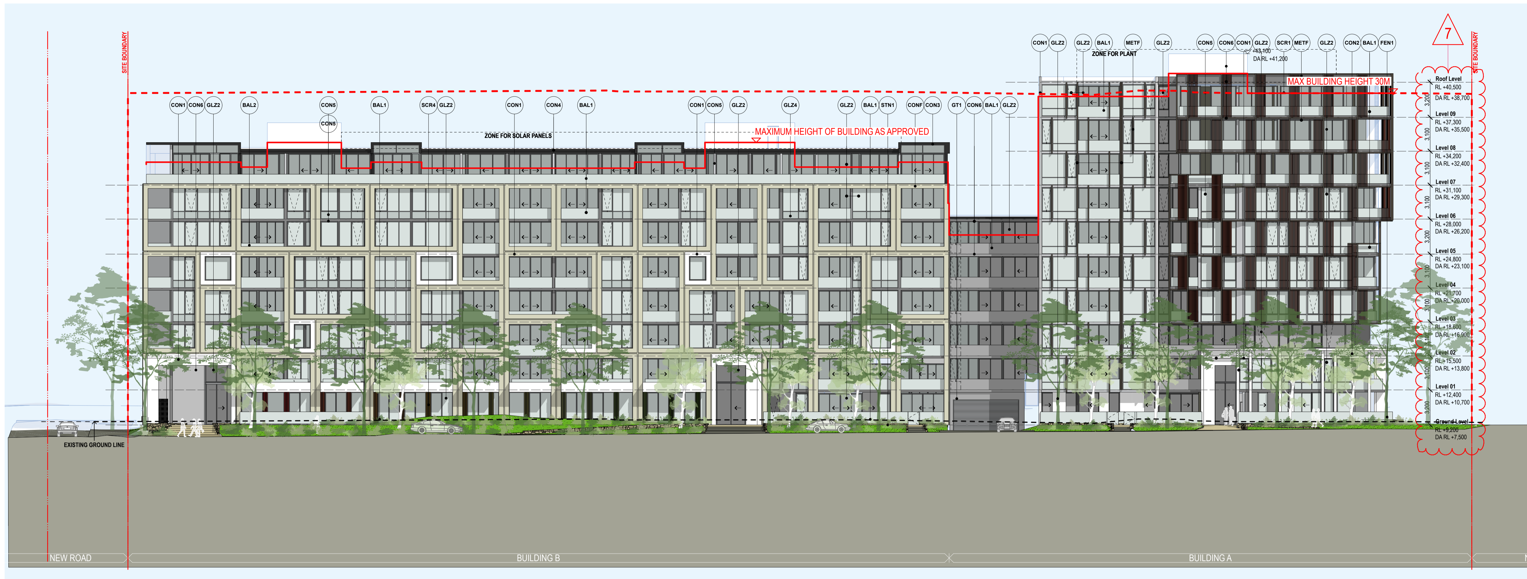
1 Building A & B East Elevation 1:200
