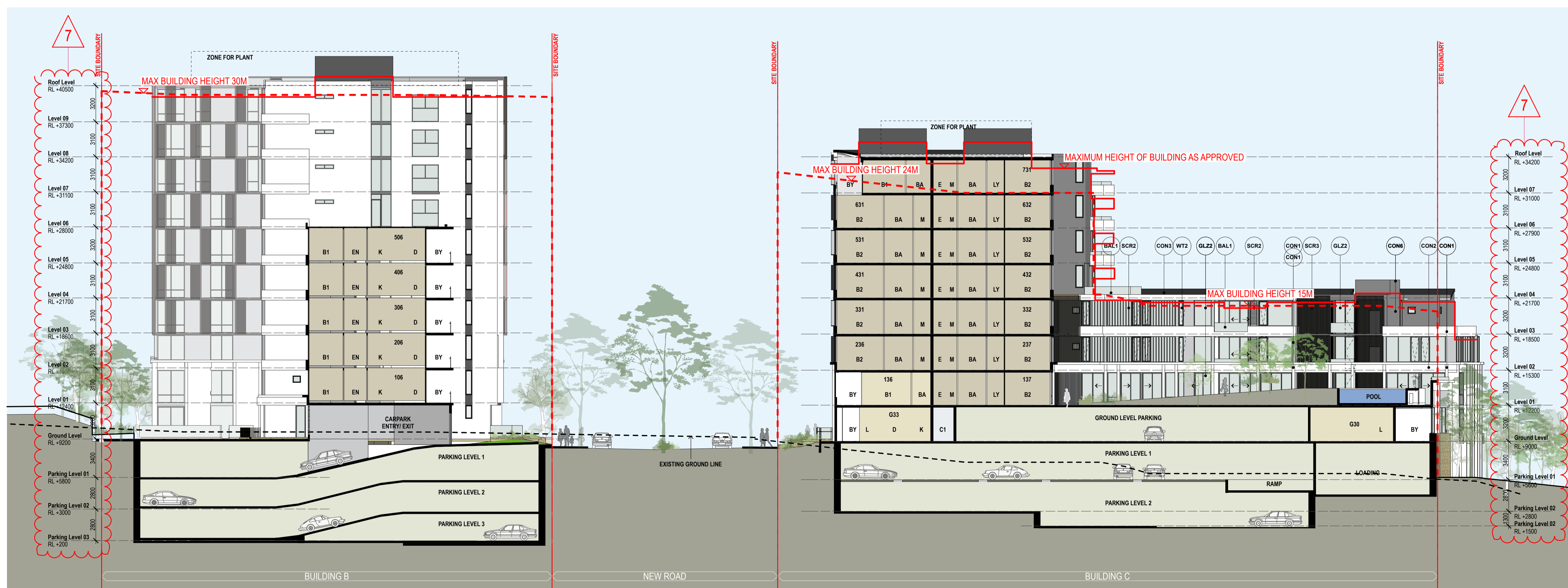
3 Section C 1:200
