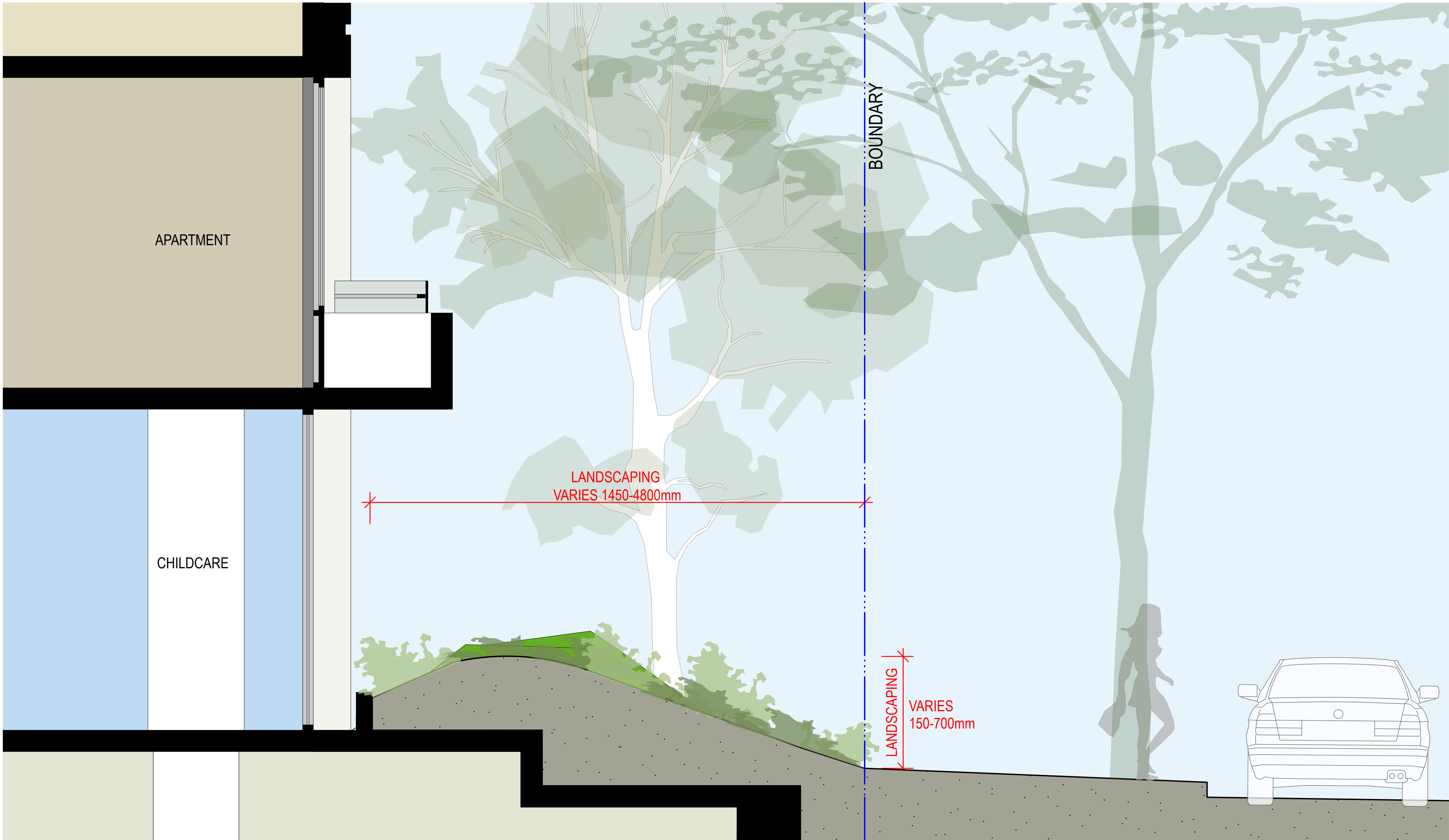
2 Section E 1:25
