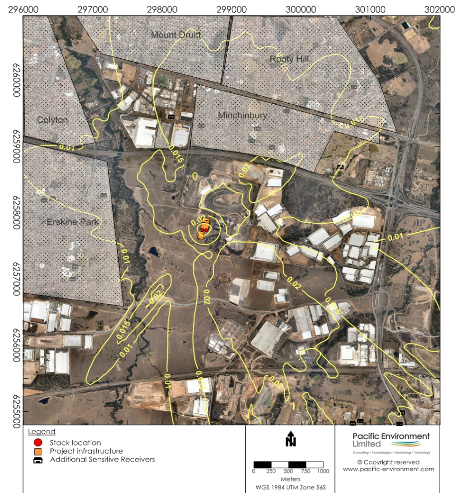
Figure 9-6: Maximum Predicted Ground Level CO Concentration – mg/m³
