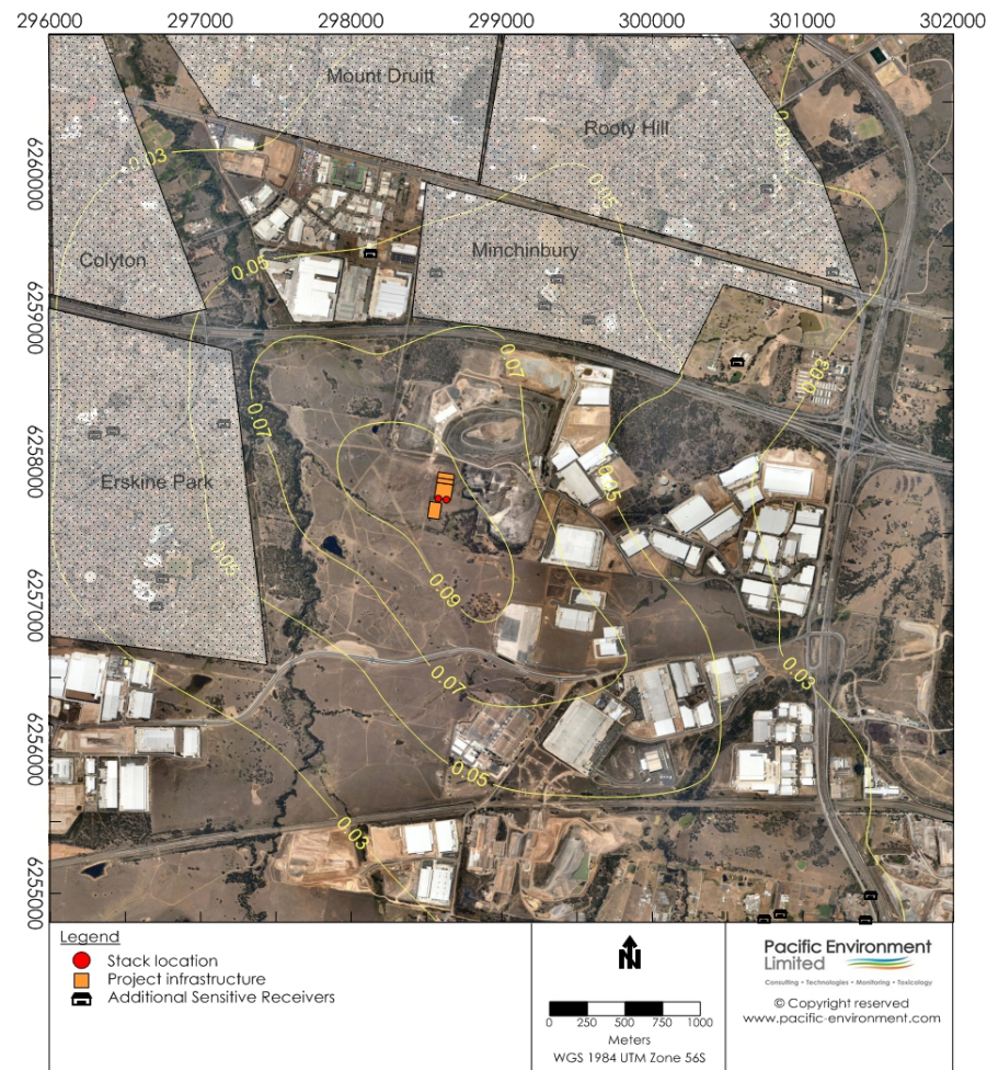
Figure 9-8: Maximum Predicted Ground Level HF Concentration
