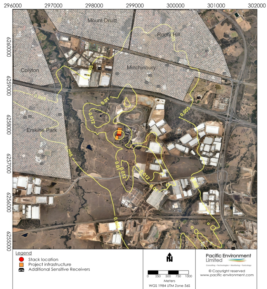
Figure 9-7: Maximum Predicted Ground Level CO Concentration – mg/m³
