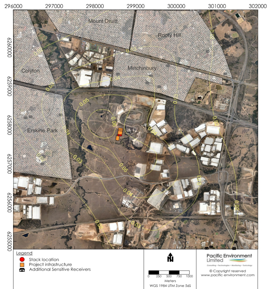
Figure 9-9: Maximum Predicted Ground Level HF Concentration
