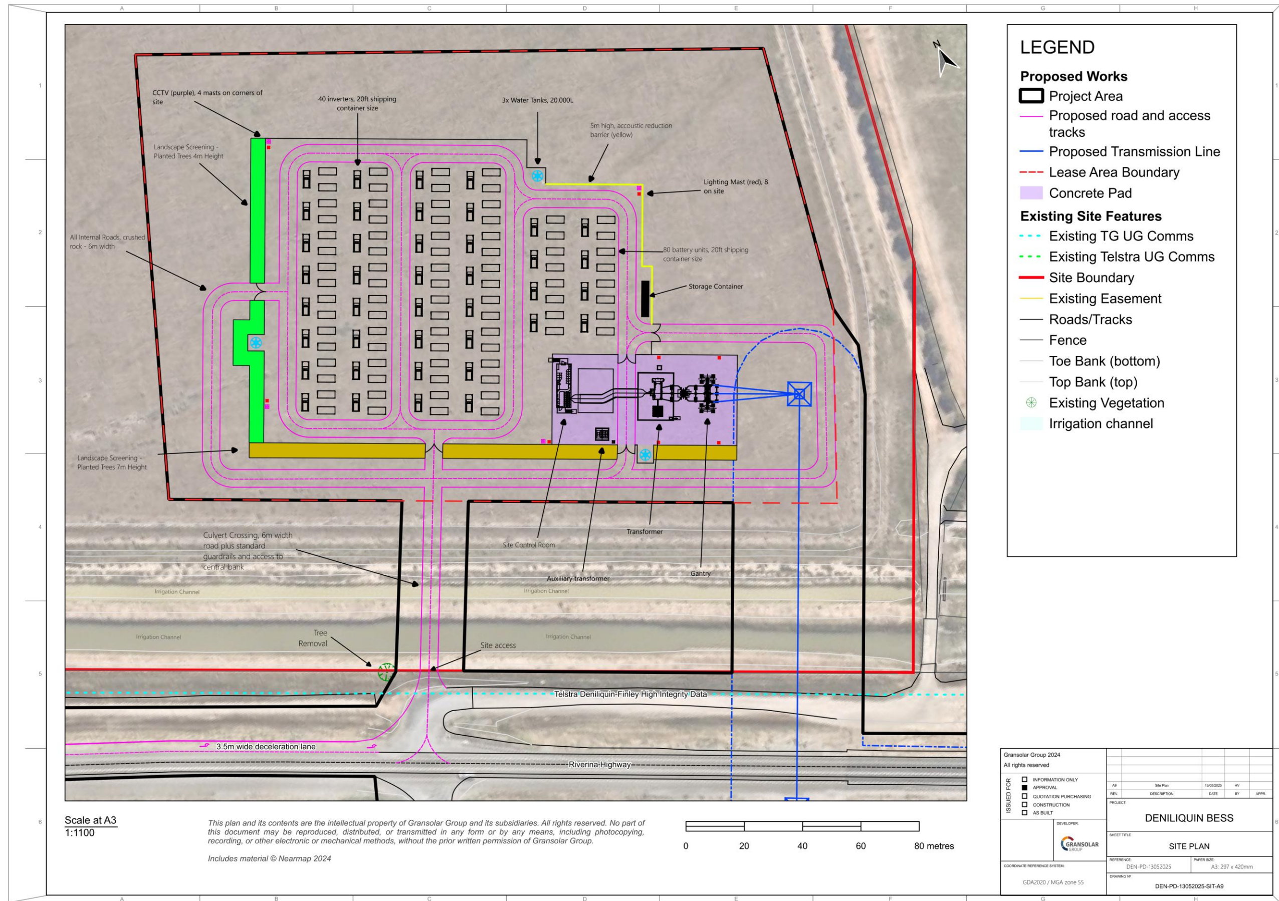
Figure 3-3: Conceptual BESS Layout
