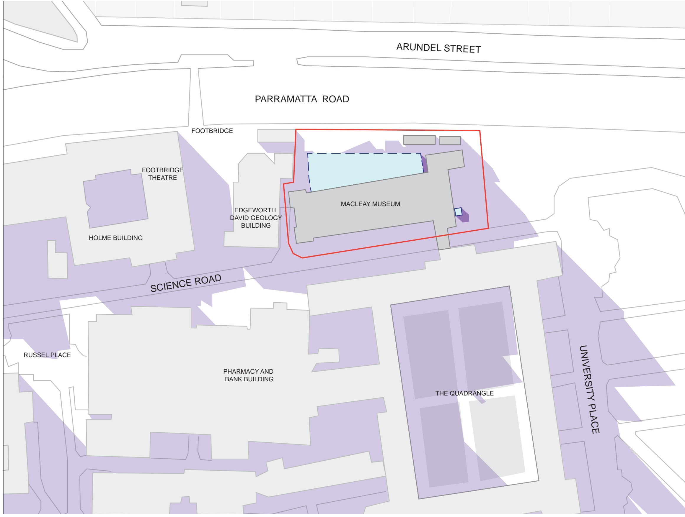
01 MACLEAY - POTENTIAL SHADOWS FROM INDICATIVE BUILT FORM 3pm, 21st OF JUNE
