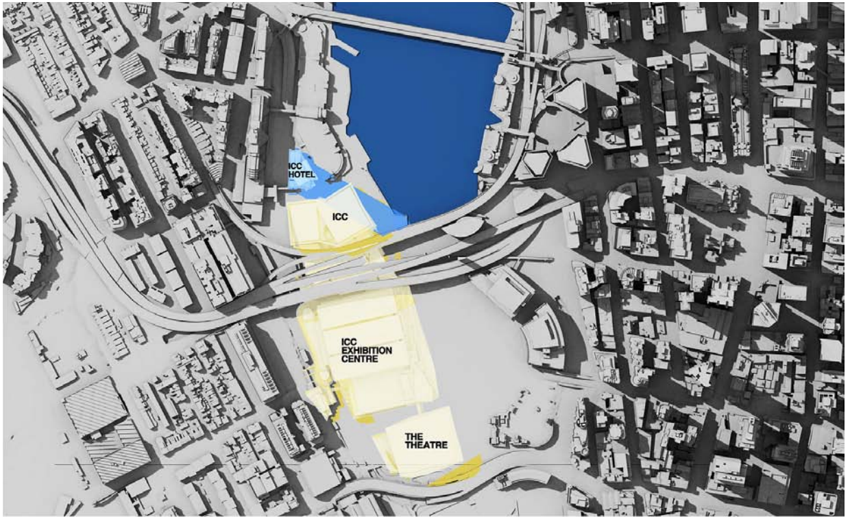
SICEEP - Shadow Study - ICC Hotel 21st March, 4pm
