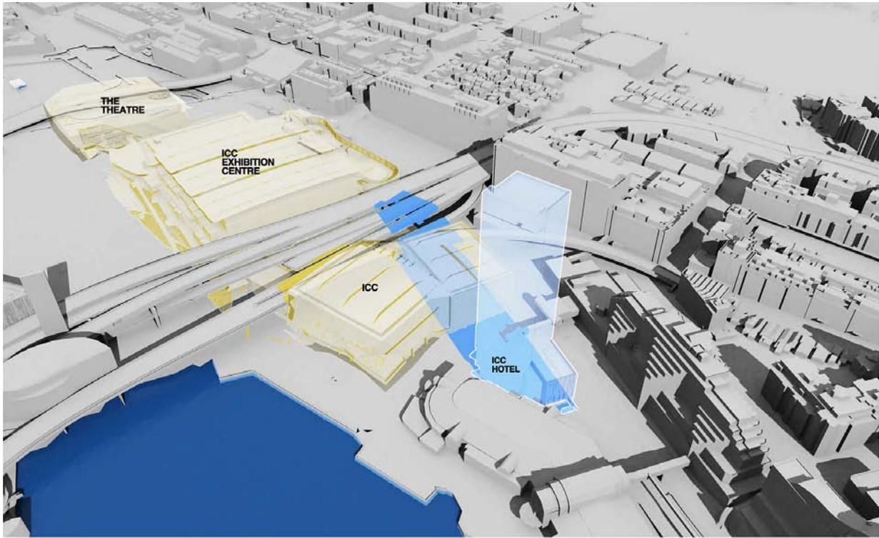
SICEEP - Shadow Study - ICC Hotel 21st June, 12pm Shadows Cast by PPP buildings Shadows cast by ICC Hotel building Shadows cast by Existing City Buildings
