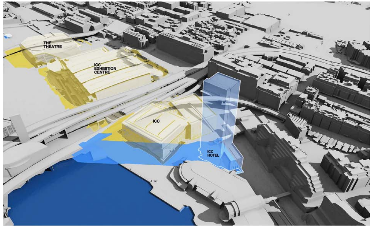
SICEEP - Shadow Study - ICC Hotel 21st September, 3pm
