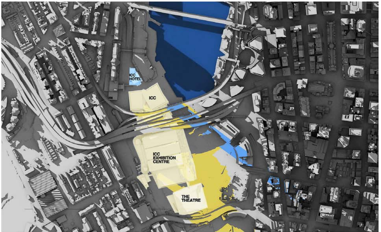
SICEEP - Shadow Study - ICC Hotel 21st June, 4pm
