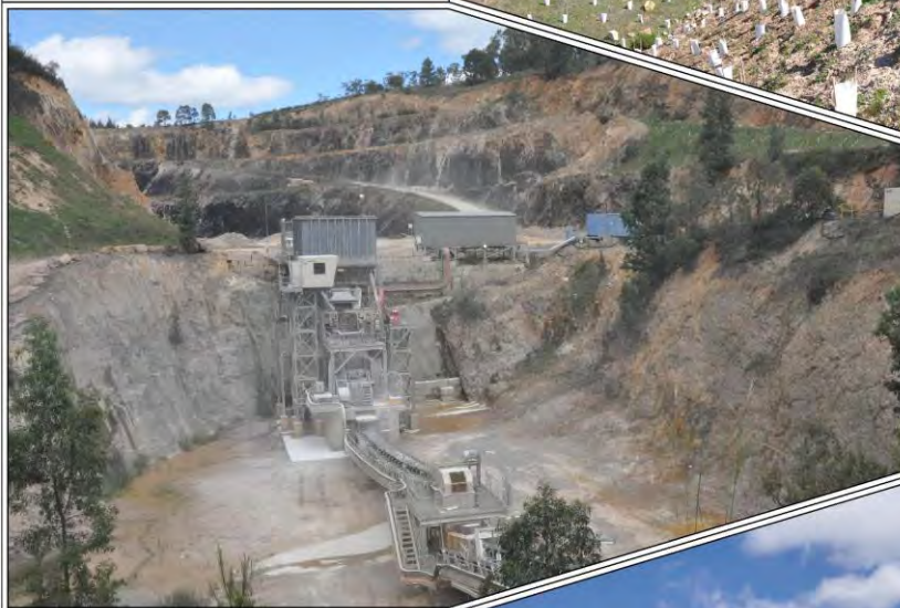
Plate 1.3: View in a southerly direction towards the Primary Crushing Station and Conveyor to the Primary Feed Stockpile (Ref: E652S_033)
