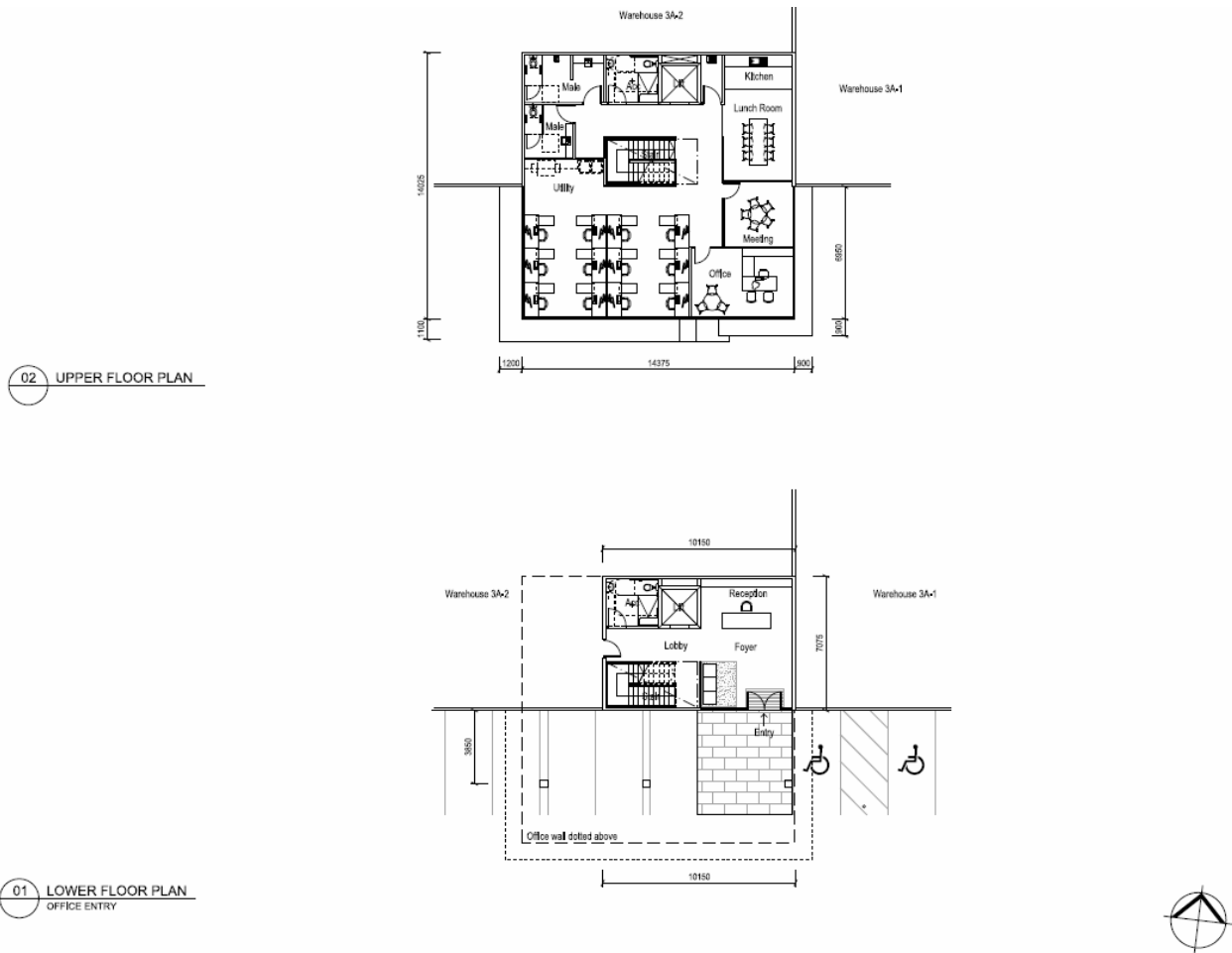
Figure 3-6: 3A-2 Office Floor Plan
