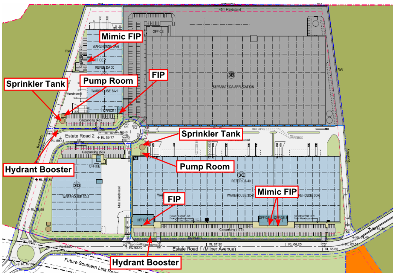
Figure 5-1: Fire Services
