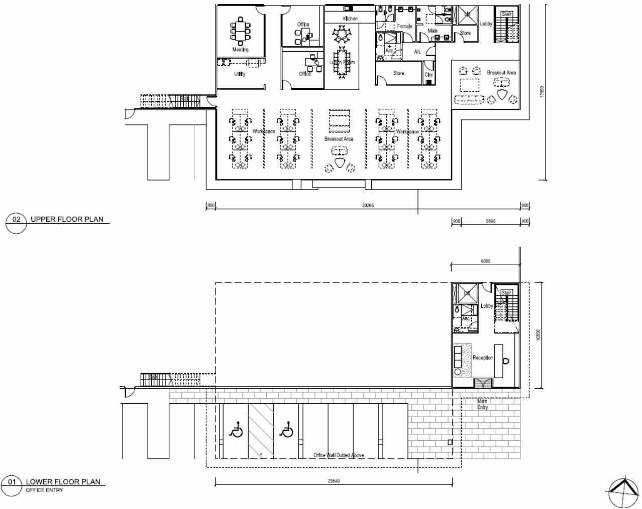
Figure 3-5: 3A-1 Office Floor Plan
