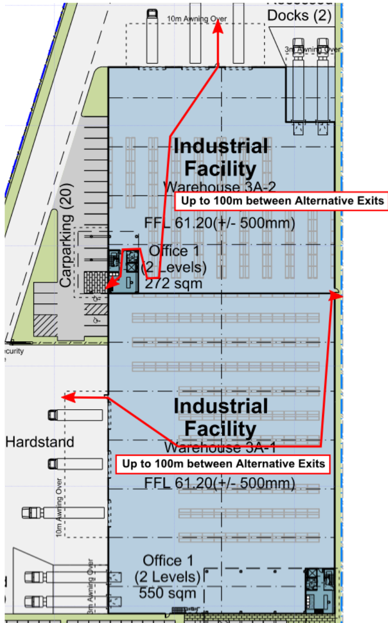
Figure 8-1: DTS Non-Compliant Travel Distances in Warehouse 3A (Tenancies 3A-1 and 3A-2)
