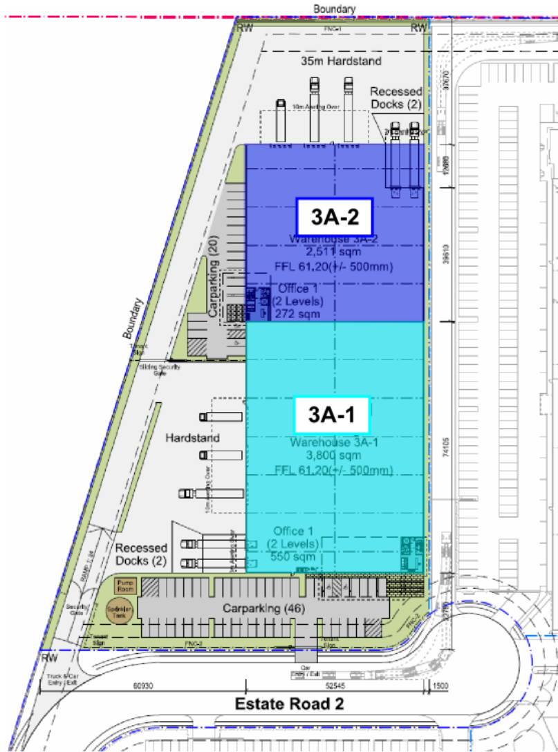
Figure 3-3: Lot 3A Warehouse
