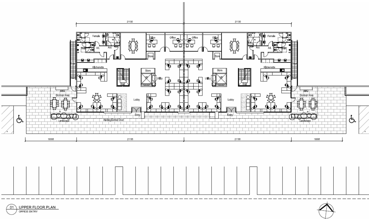
Figure 3-8: 3C-2 and 3C-3 Office Upper Floor Plan
