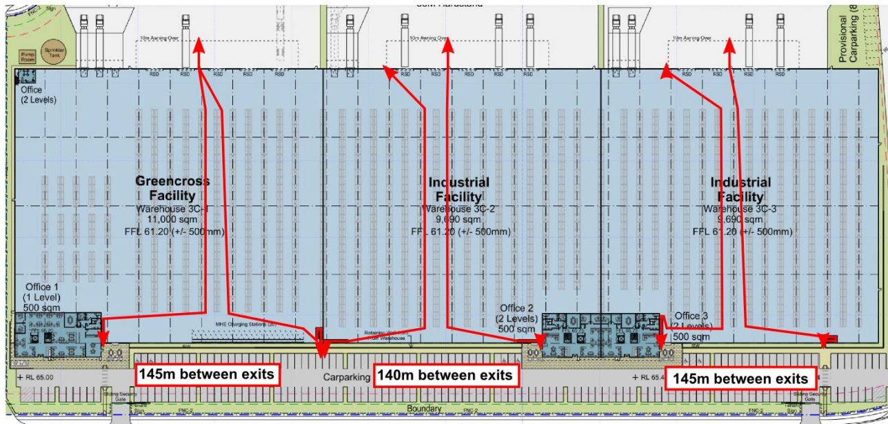
Figure 8-2: DTS Non-Compliant Travel Distances in Building 3C (Warehouses 3C-1, 3C-2 and 3C-3)
