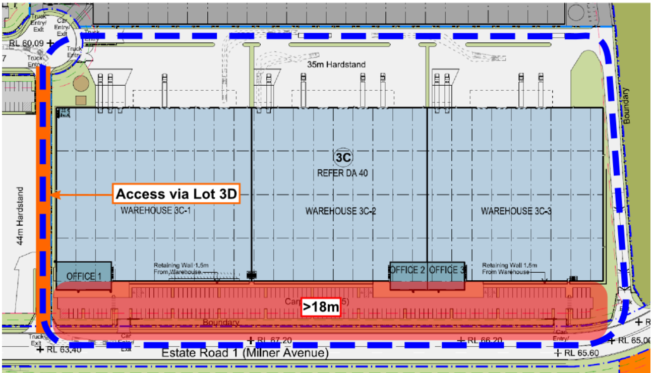
Figure 8-3: Perimeter Access Non-Compliances on Lot 3C
