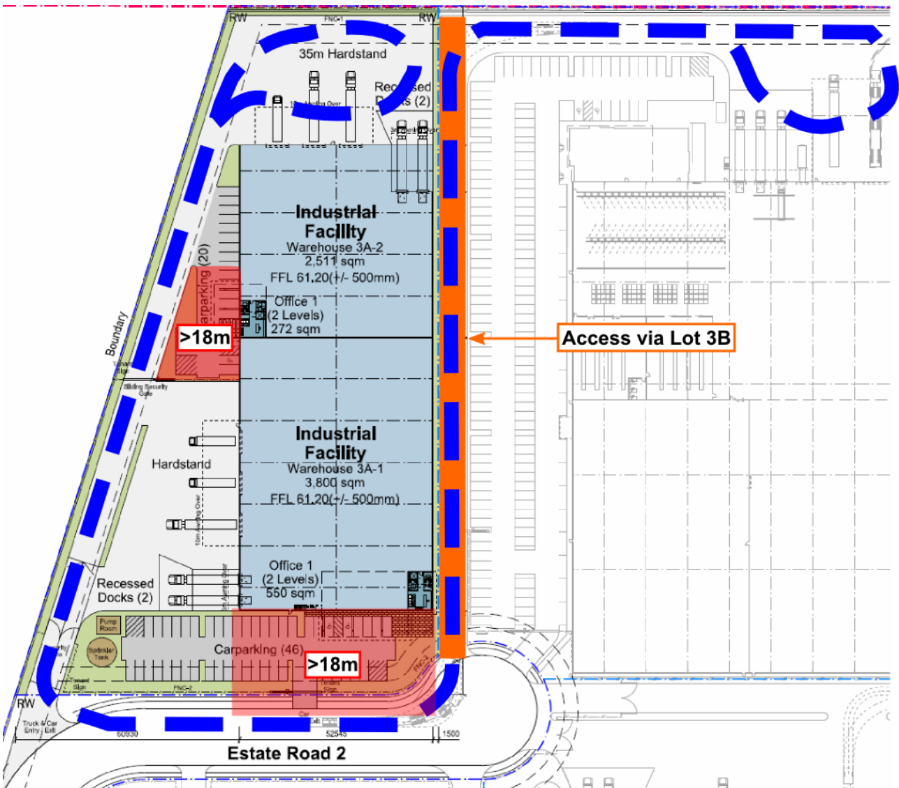
Figure 8-4: Perimeter Access Non-Compliances on Lot 3A
