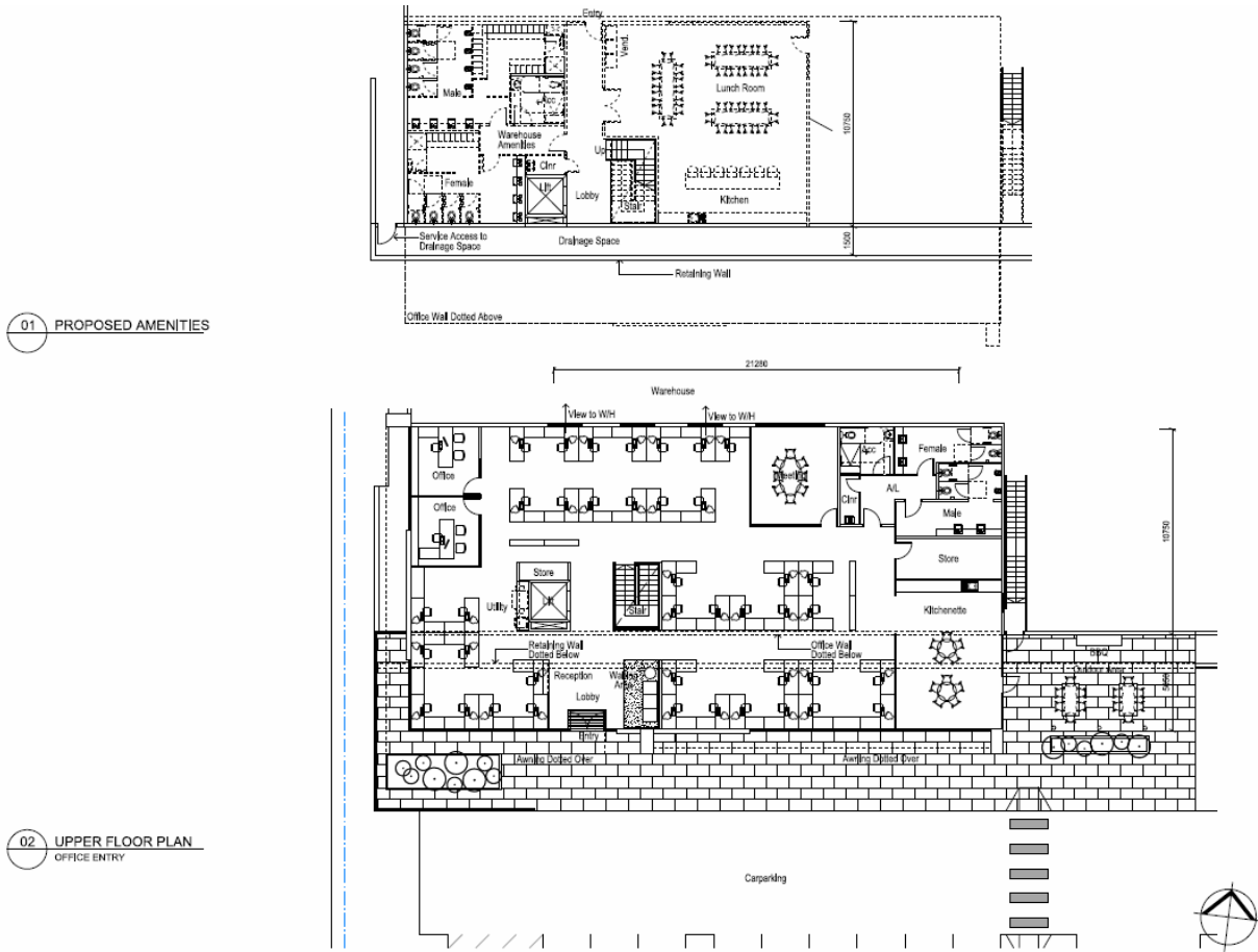
Figure 3-7: 3C-1 Office Floor Plan
