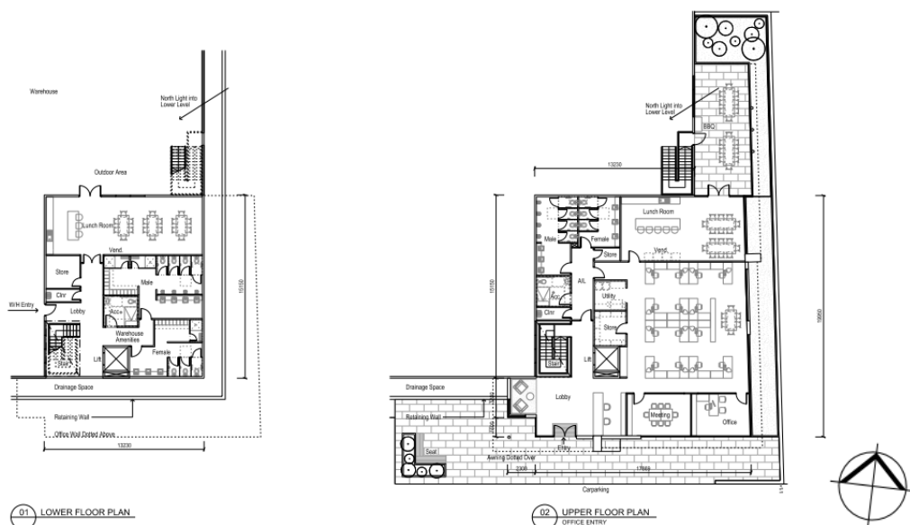
Figure 3-5: 3C Office Floor Plan
