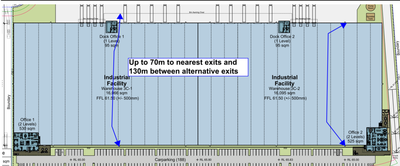
Figure 7-2: DTS Non-compliant Travel Distances in Building 3C-1/2
