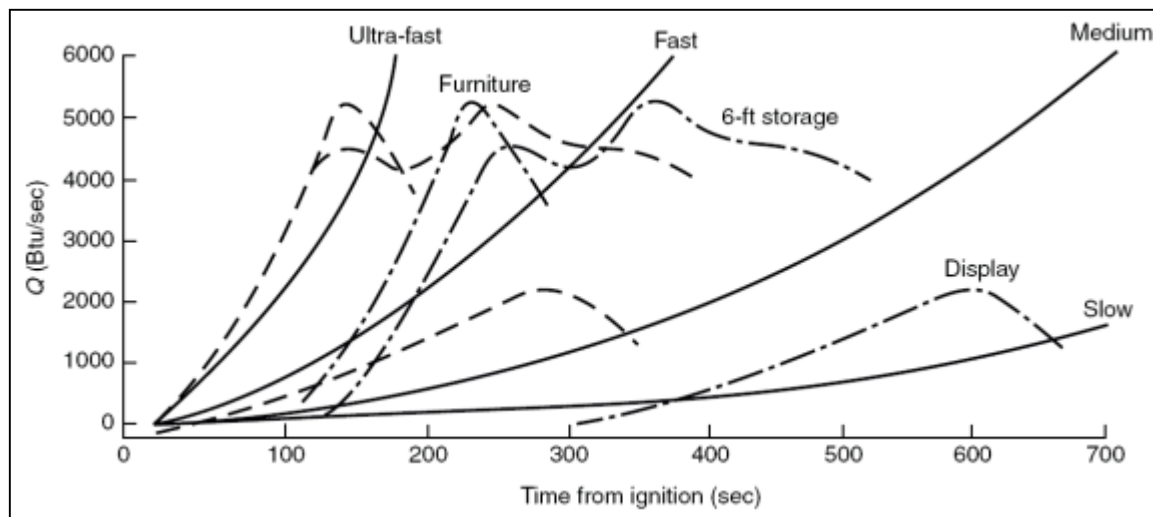
Figure 5-5: NFPA 92B: T-squared fire, rates of energy release
