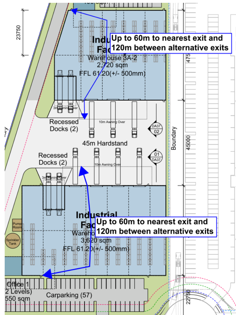
Figure 7-1: DTS Non-compliant Travel Distances in Building 3A-1 and 3A-2
