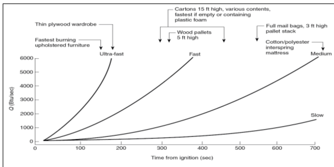
Figure 5-6: NFPA 92B: Relation of t-squared fires to some fire tests
