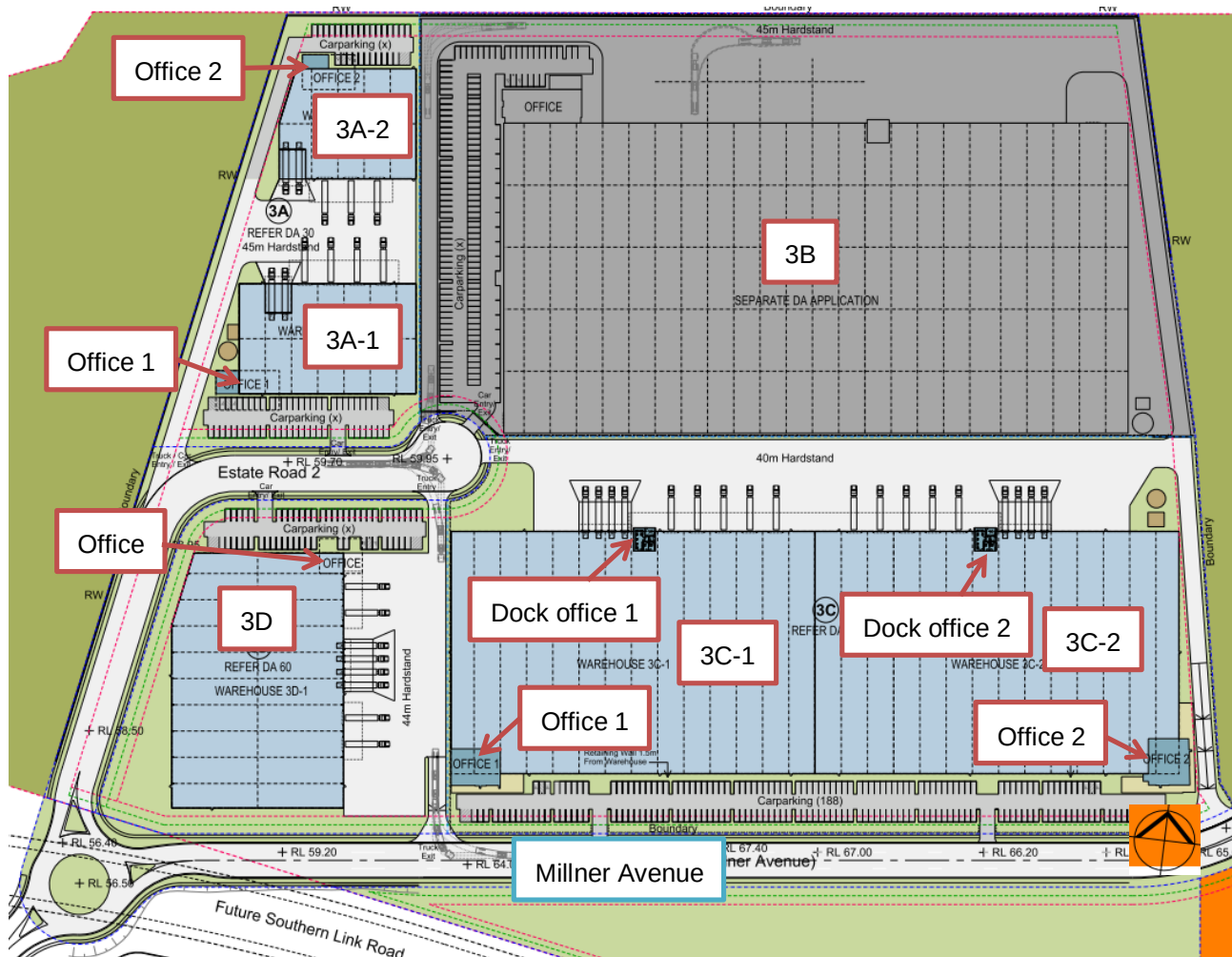
Figure 3-2: Site Layout
