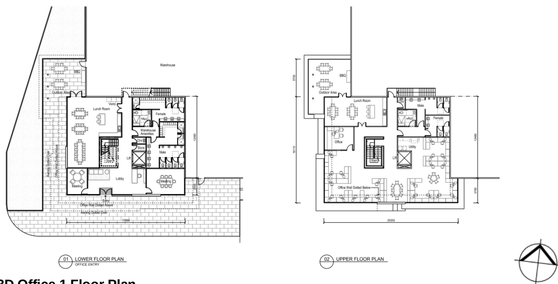
Figure 3-6: 3D Office 1 Floor Plan
