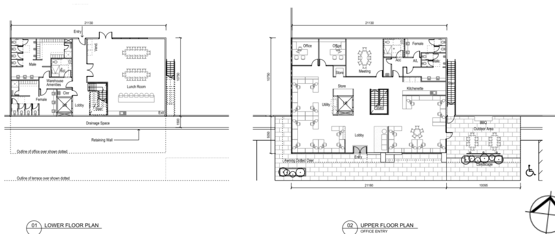
Figure 3-7: 3D Office 2 Floor Plan
