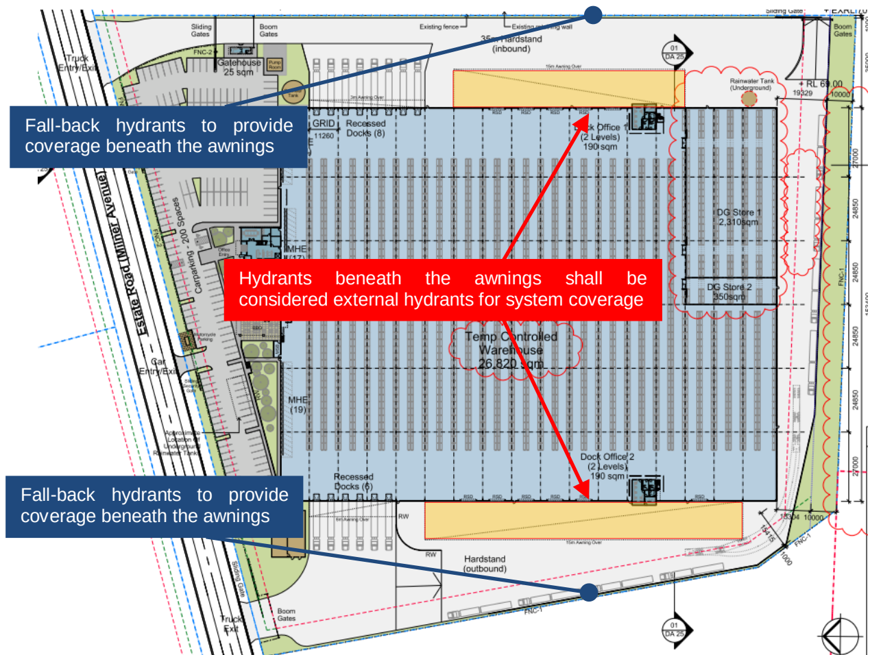
Figure 7-2: Hydrants under the awnings and fall-back hydrant requirements
