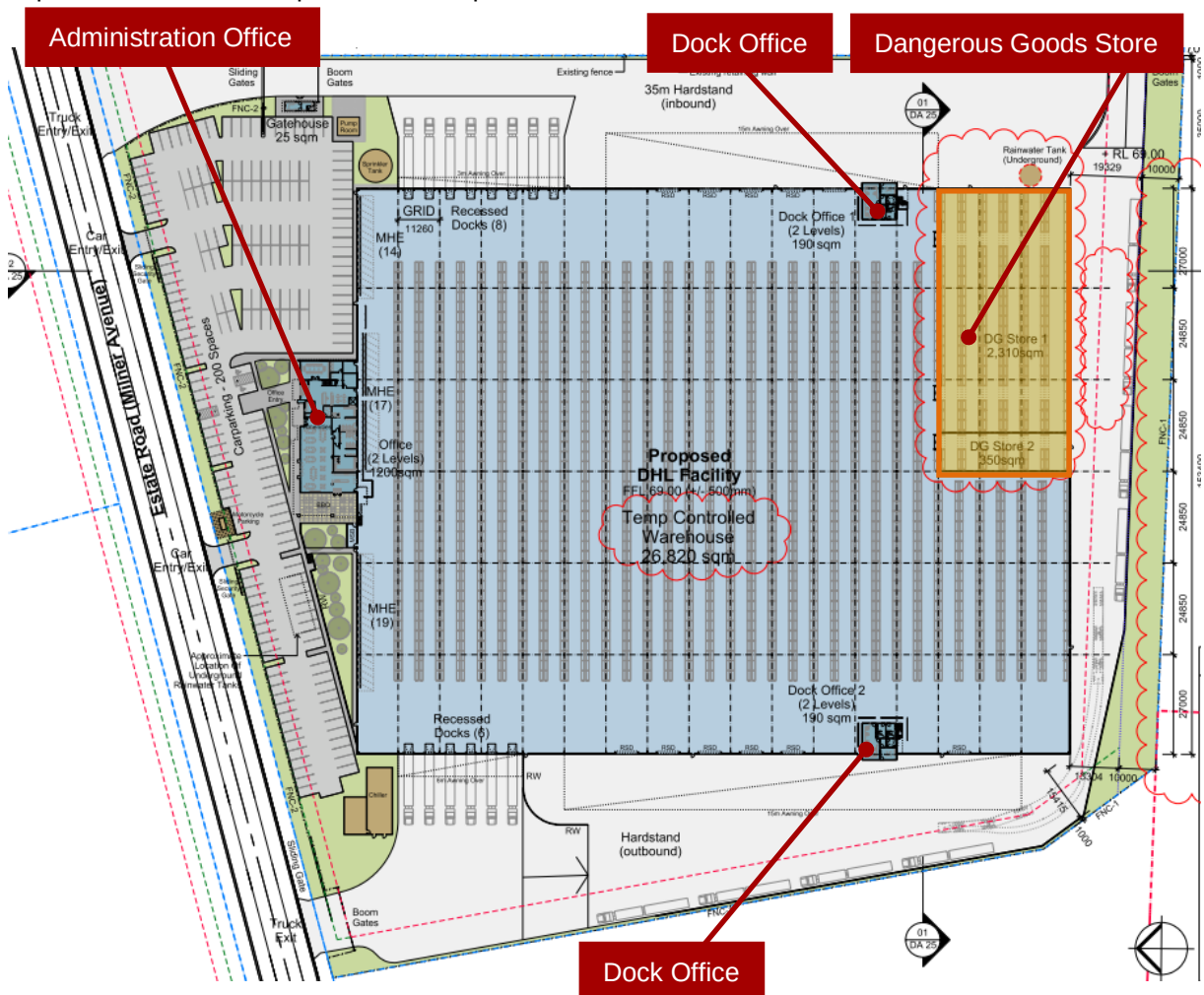
Figure 3-2: Site Plan
