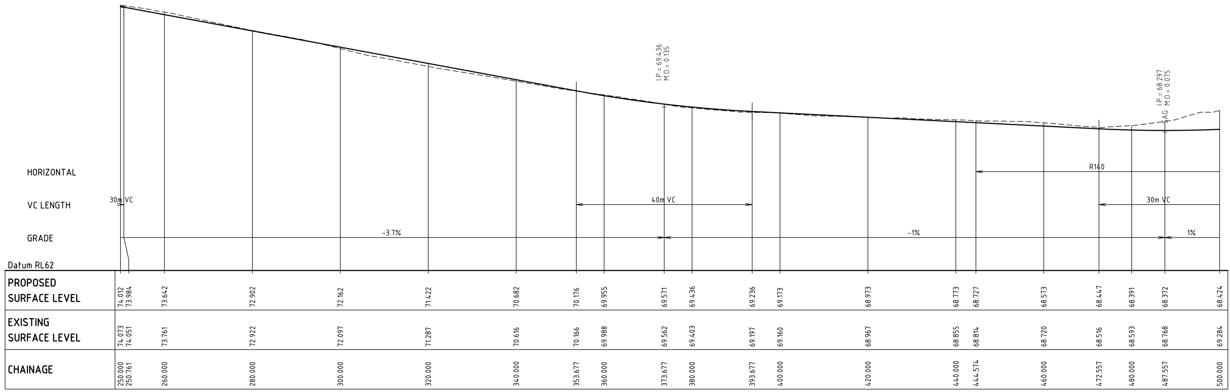
CONTROL LINE MC01 LONGITUDINAL SECTION SCALE 1:500 HORI. 1:250 VERT.
