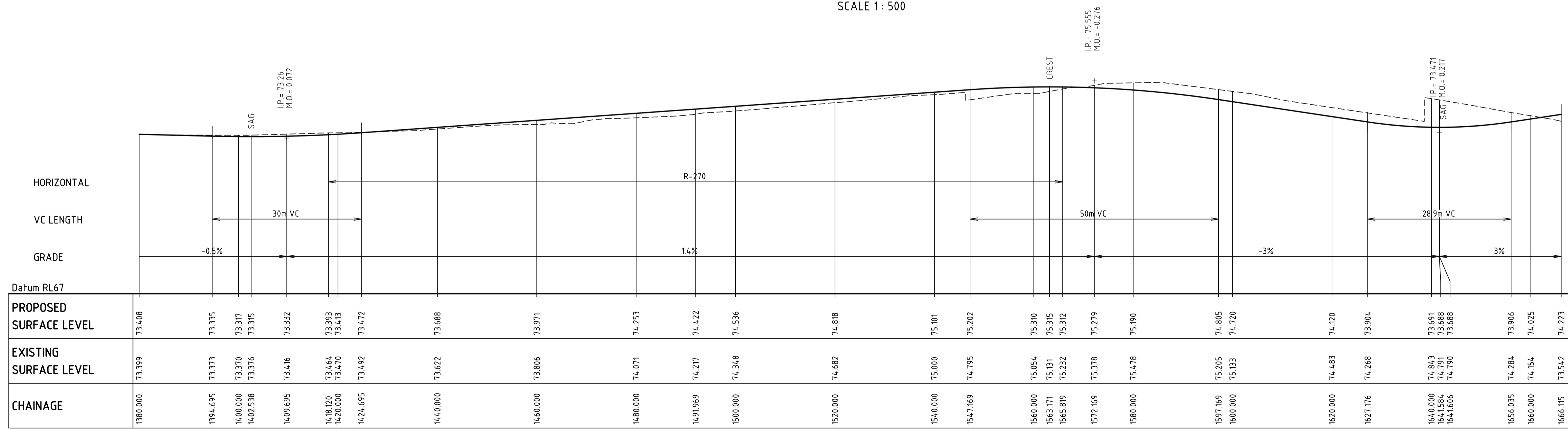
CONTROL LINE MC01 LONGITUDINAL SECTION SCALE 1:500 HORI. 1:250 VERT.
