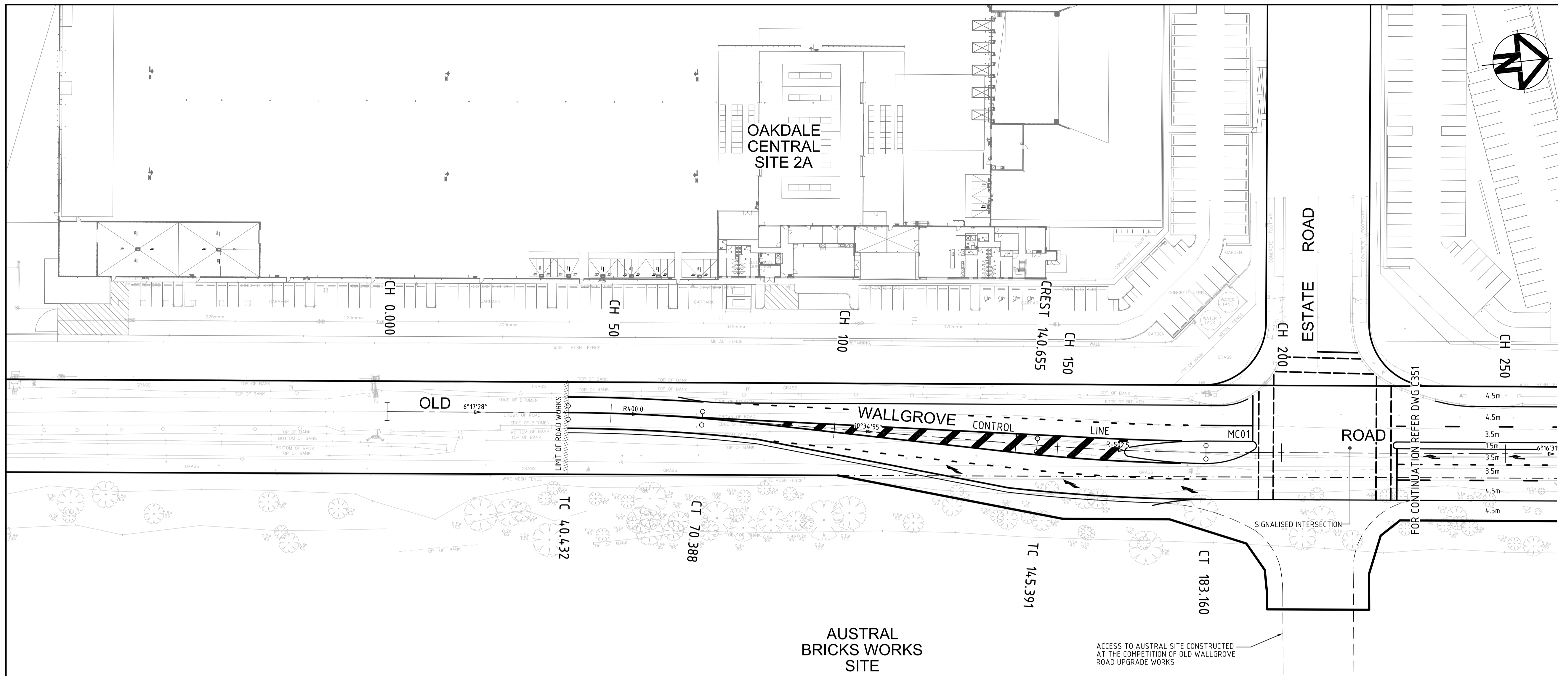
PLAN SCALE 1:500
