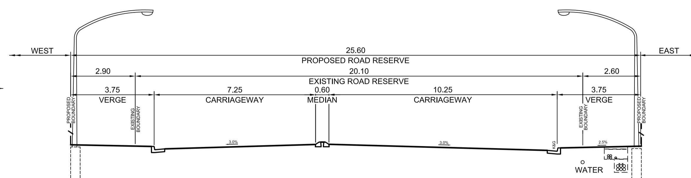
OLD WALLGROVE ROAD TYPICAL SECTION CH 1050 SCALE 1:100
