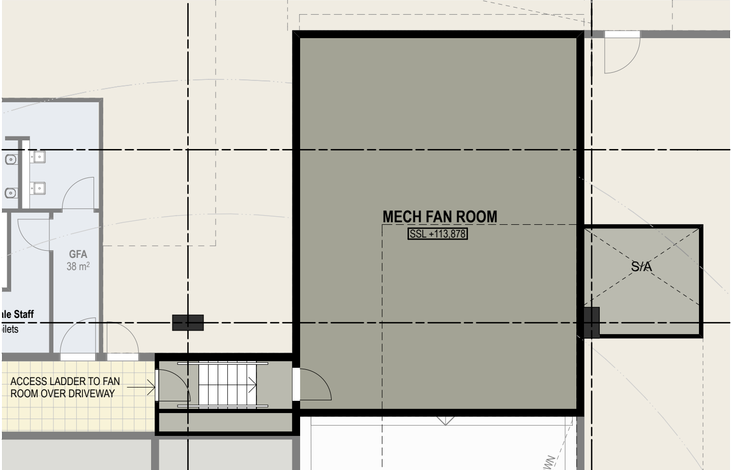
4 Mechanical Fan Room over Entry driveway
