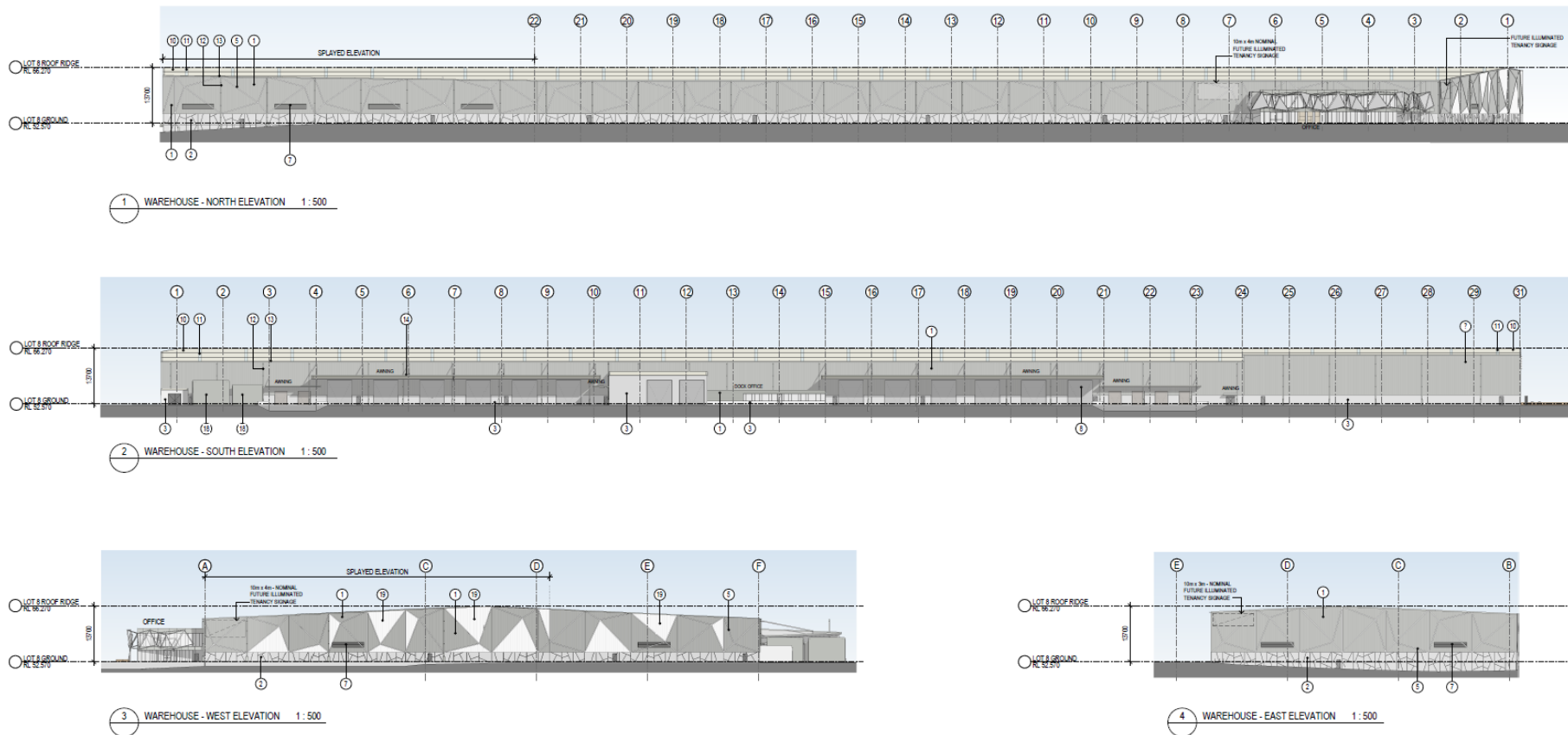
Figure 2: Elevations
