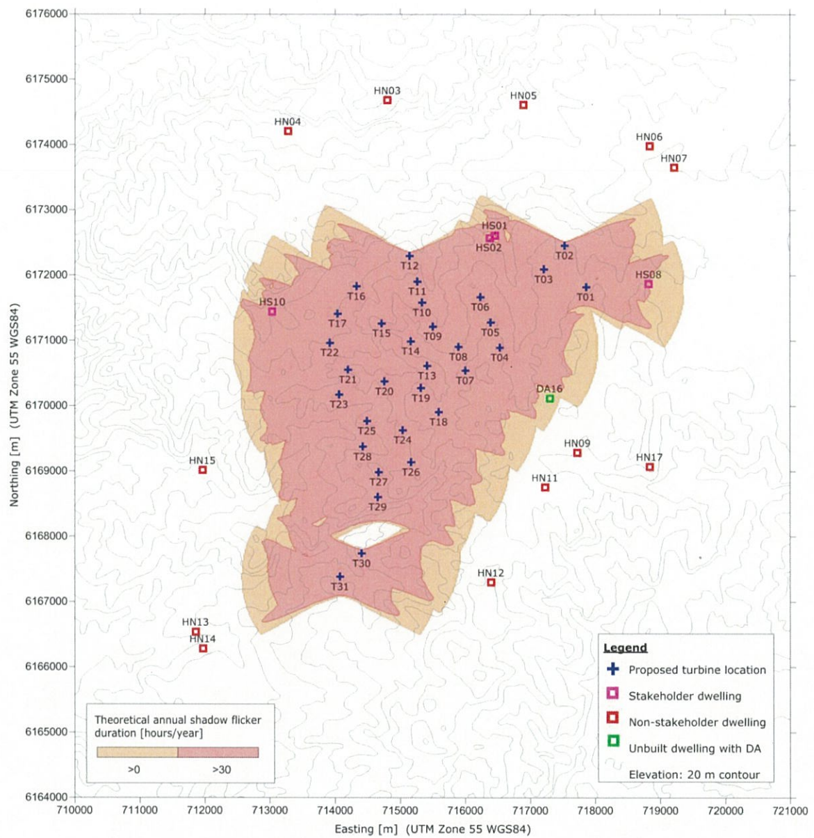
Figure 7: Map of the proposed Biala Wind Farm with turbines, dwelling locations and theoretical annual shadow flicker duration at 6 m above ground level
