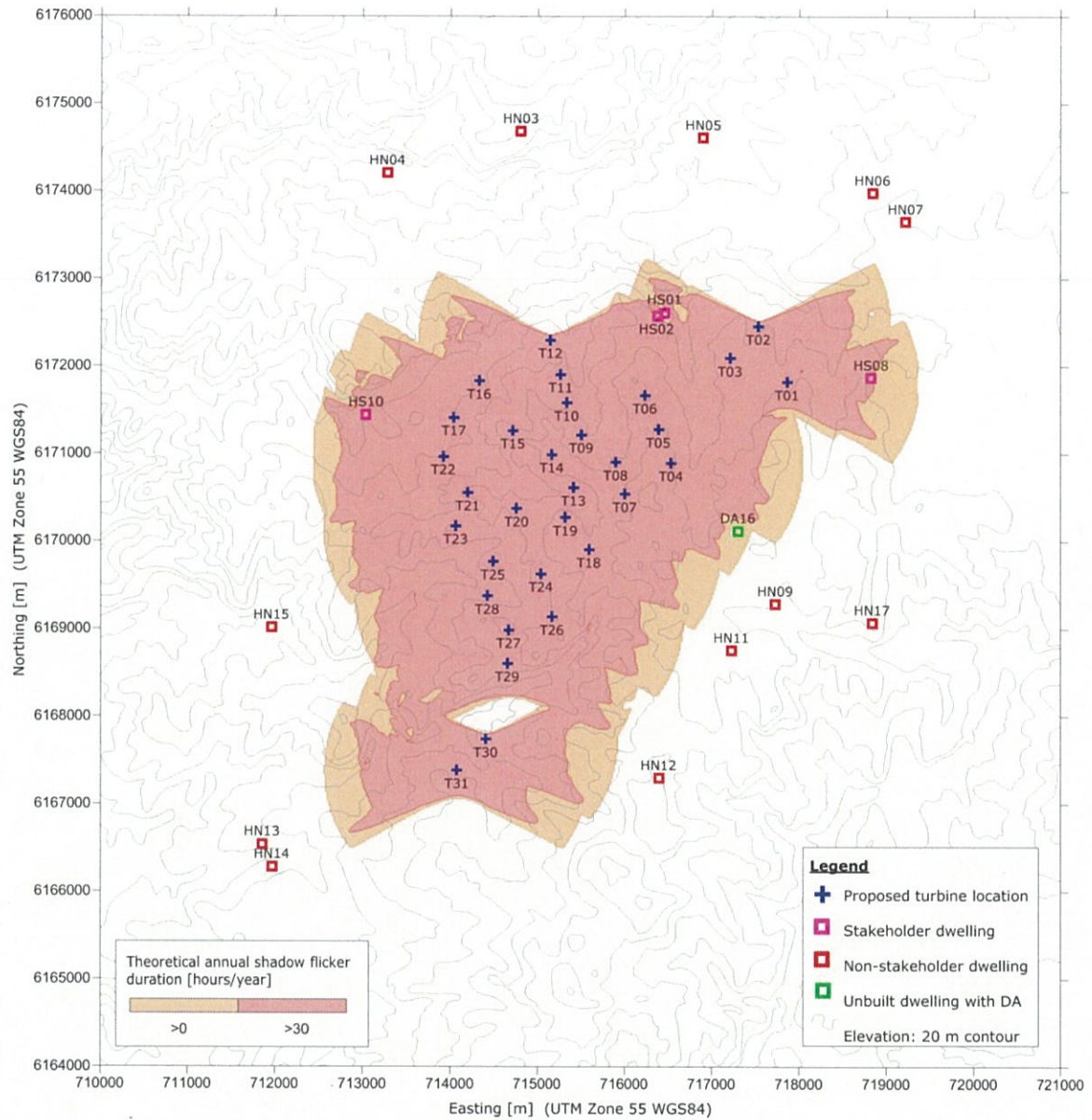
Figure 6: Map of the proposed Biala Wind Farm with turbines, dwelling locations and theoretical annual shadow flicker duration at 2 m above ground level
