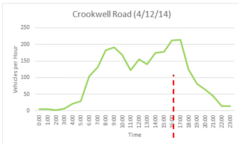
Figure 1 Daily Traffic Count, Crookwell Road 4/12/14
