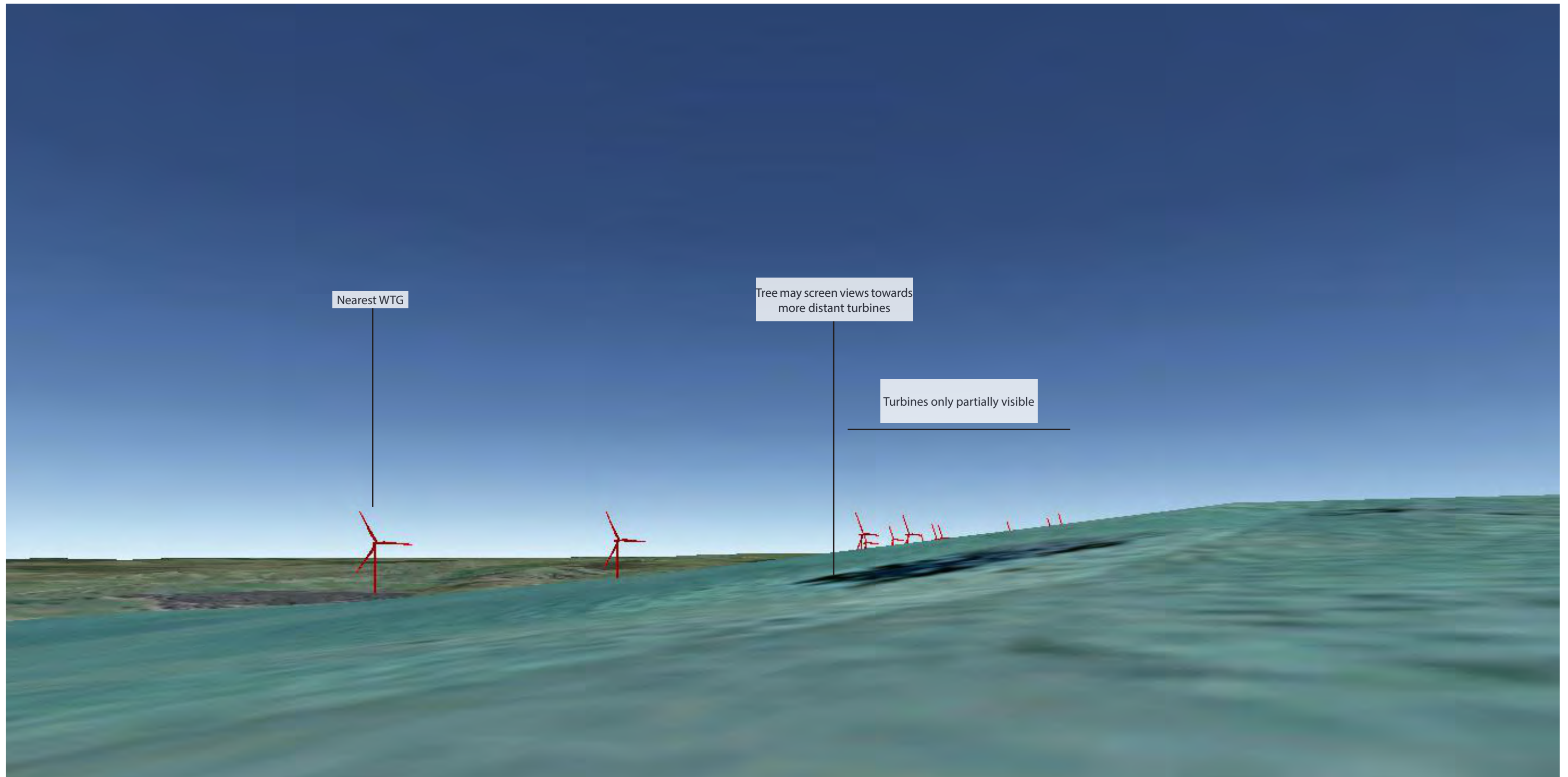
Viewpoint 11 - Photo 11A - Simulated view northwest towards proposed Biala Wind Farm from location of proposed property DA18
