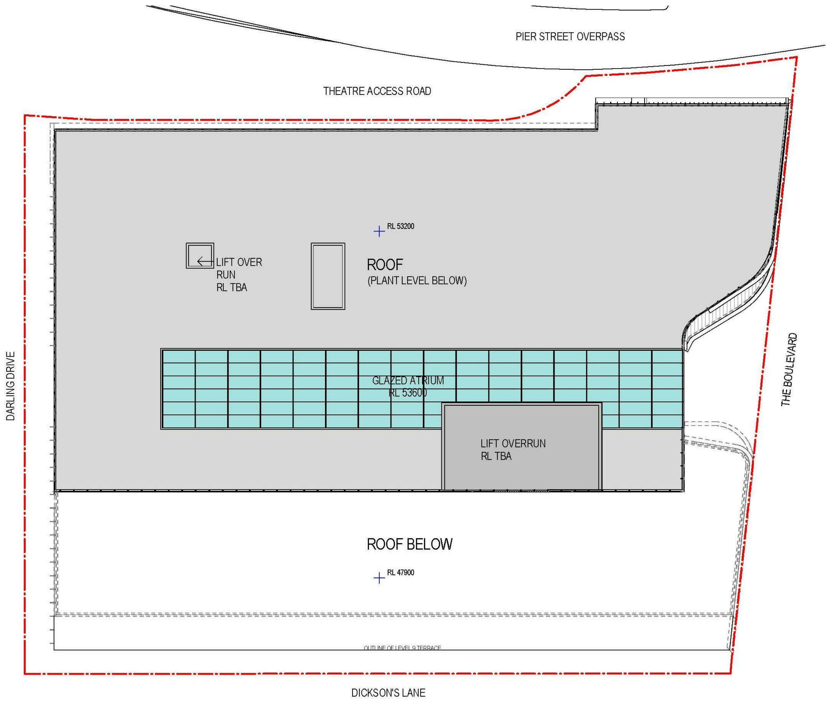
1 Roof Level - Approved SSD 6013 SCALE 1 : 250
