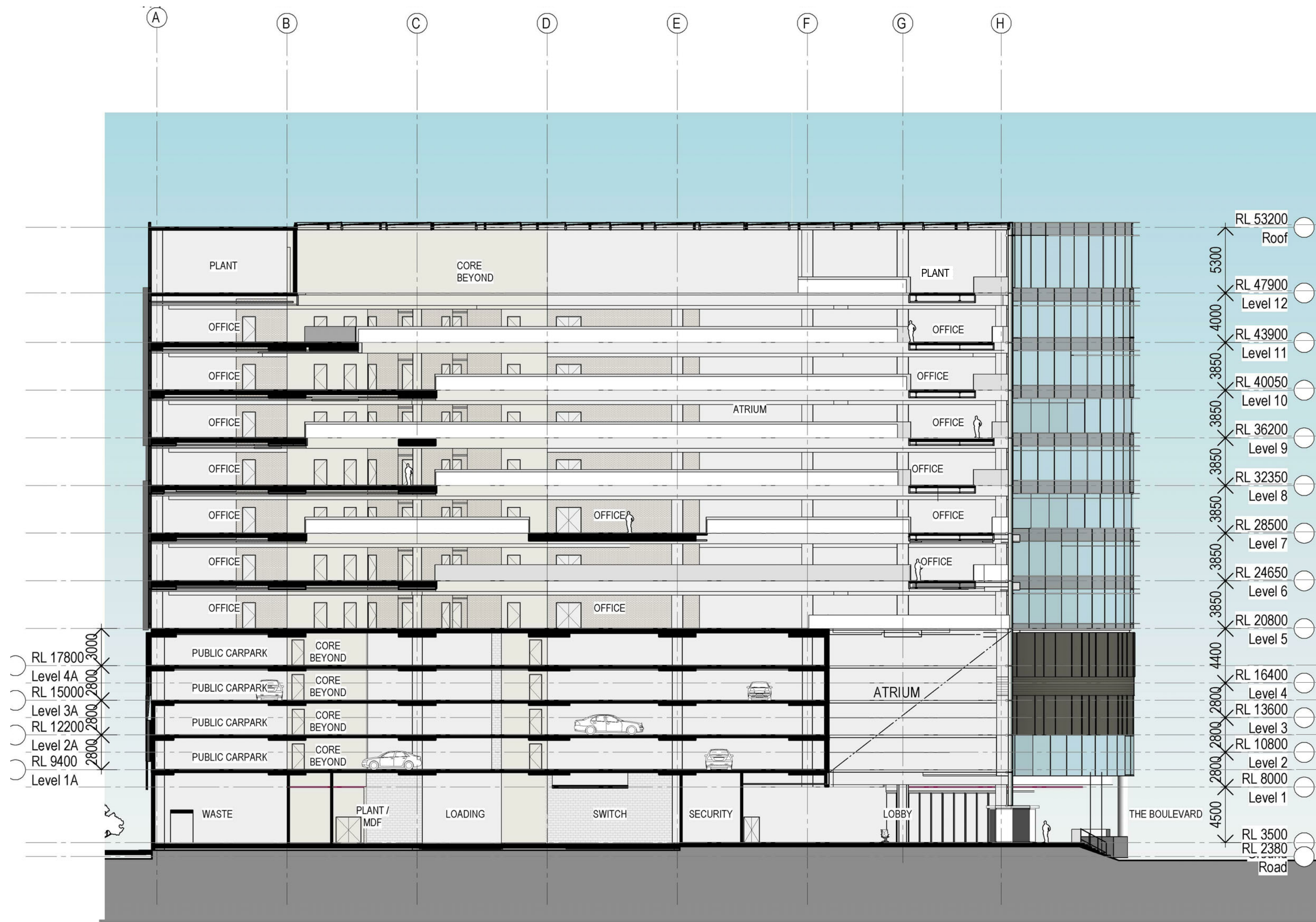
2 Section AA - Approved SSD 6013 SCALE 1 : 250
