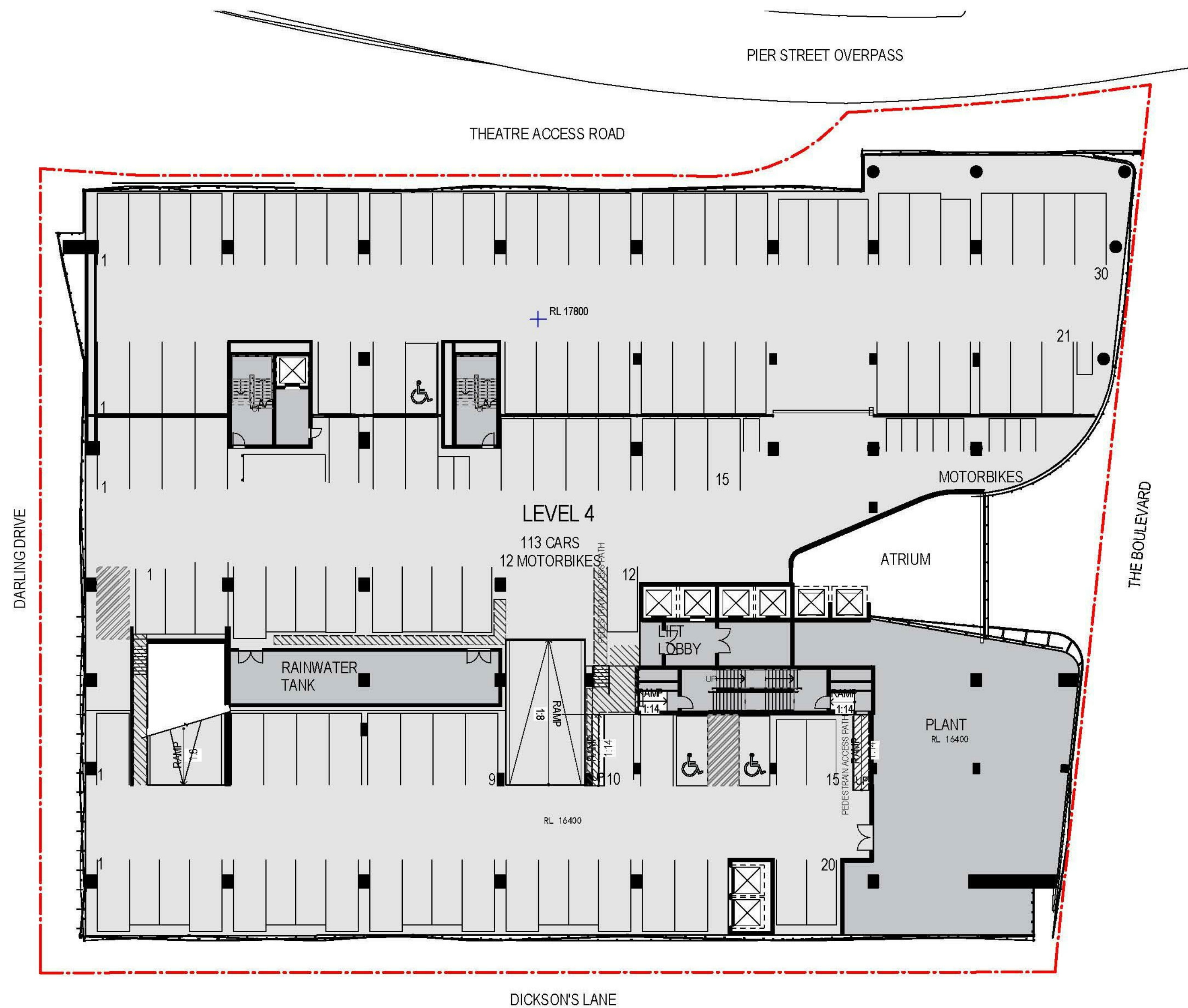
1 Level 4 - Approved SSD 6013 SCALE 1 : 250
