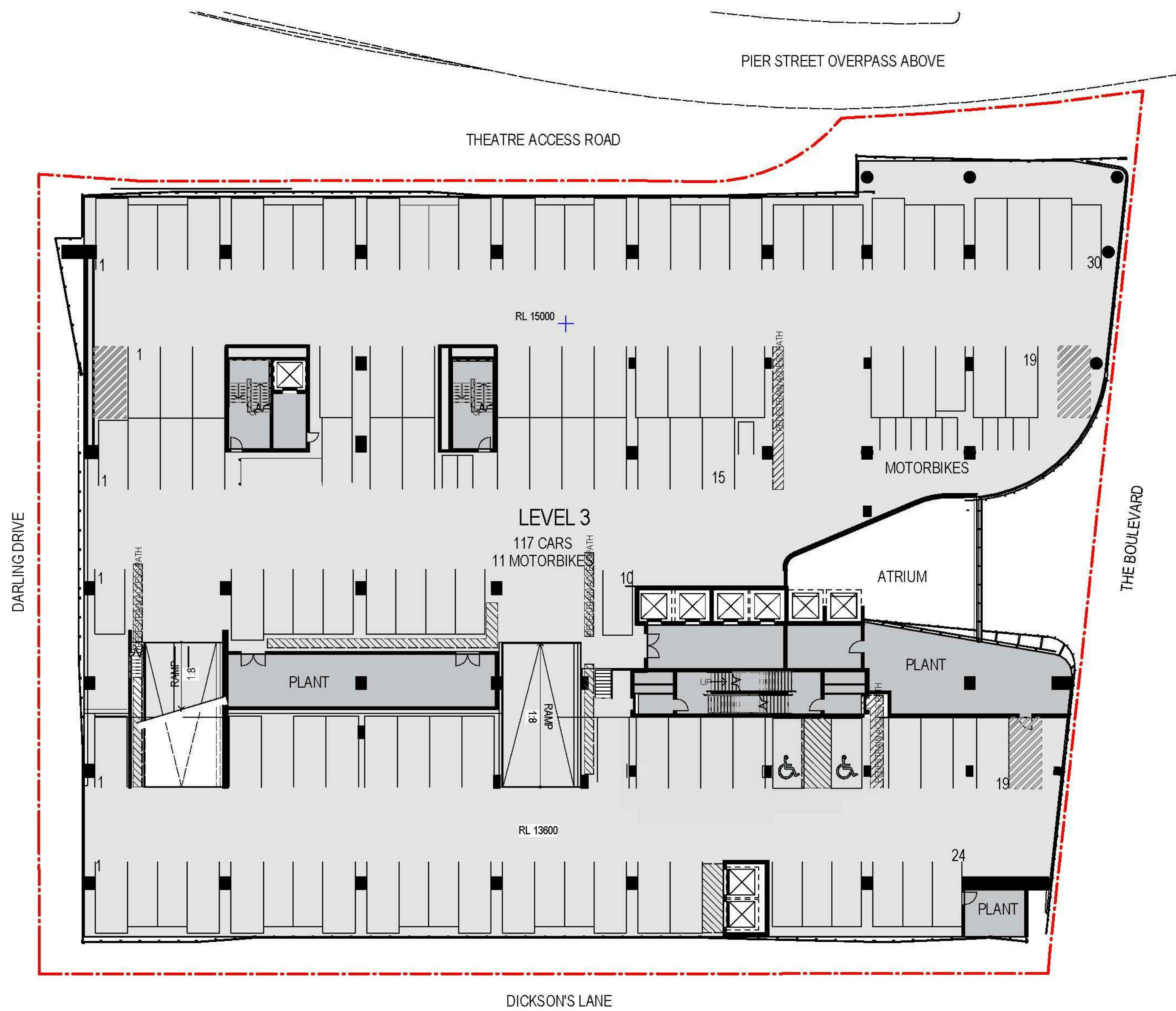
1 Level 3 - Approved SSD 6013 SCALE 1 : 250
