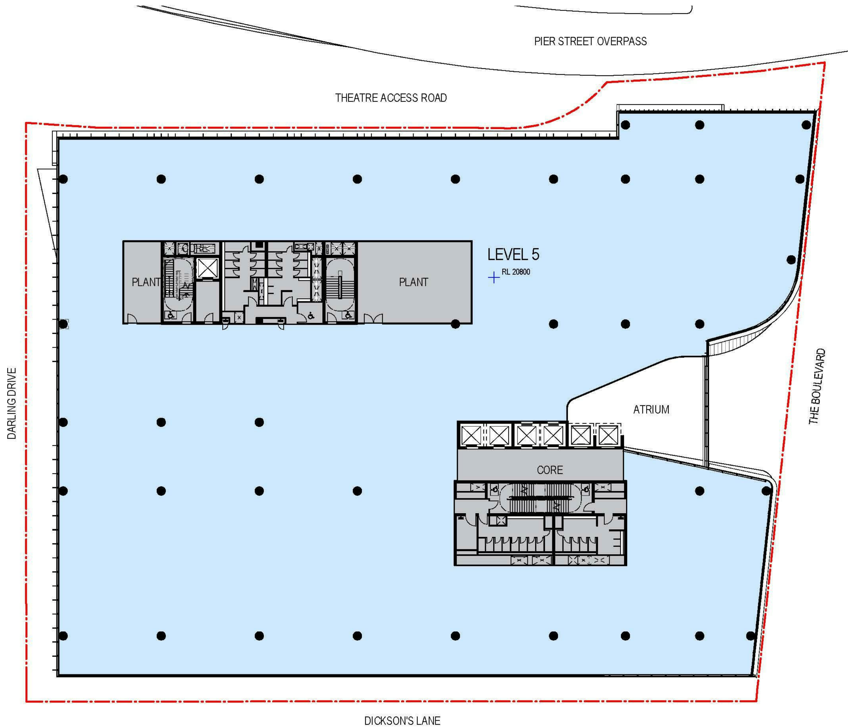
1 Level 5 - Approved SSD 6013 SCALE 1 : 250
