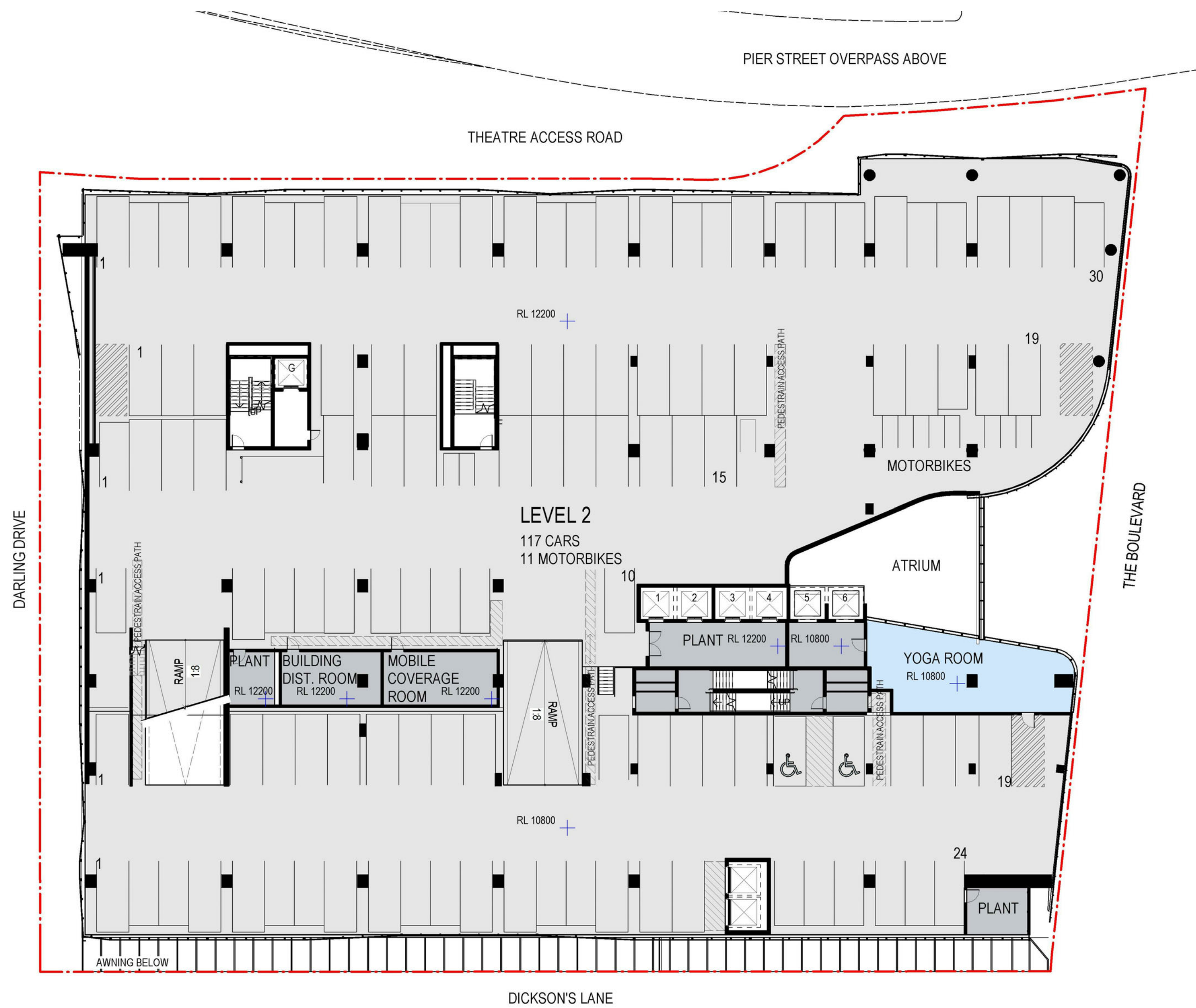
2 Level 2 - Approved SSD 6013 SCALE 1 : 250
