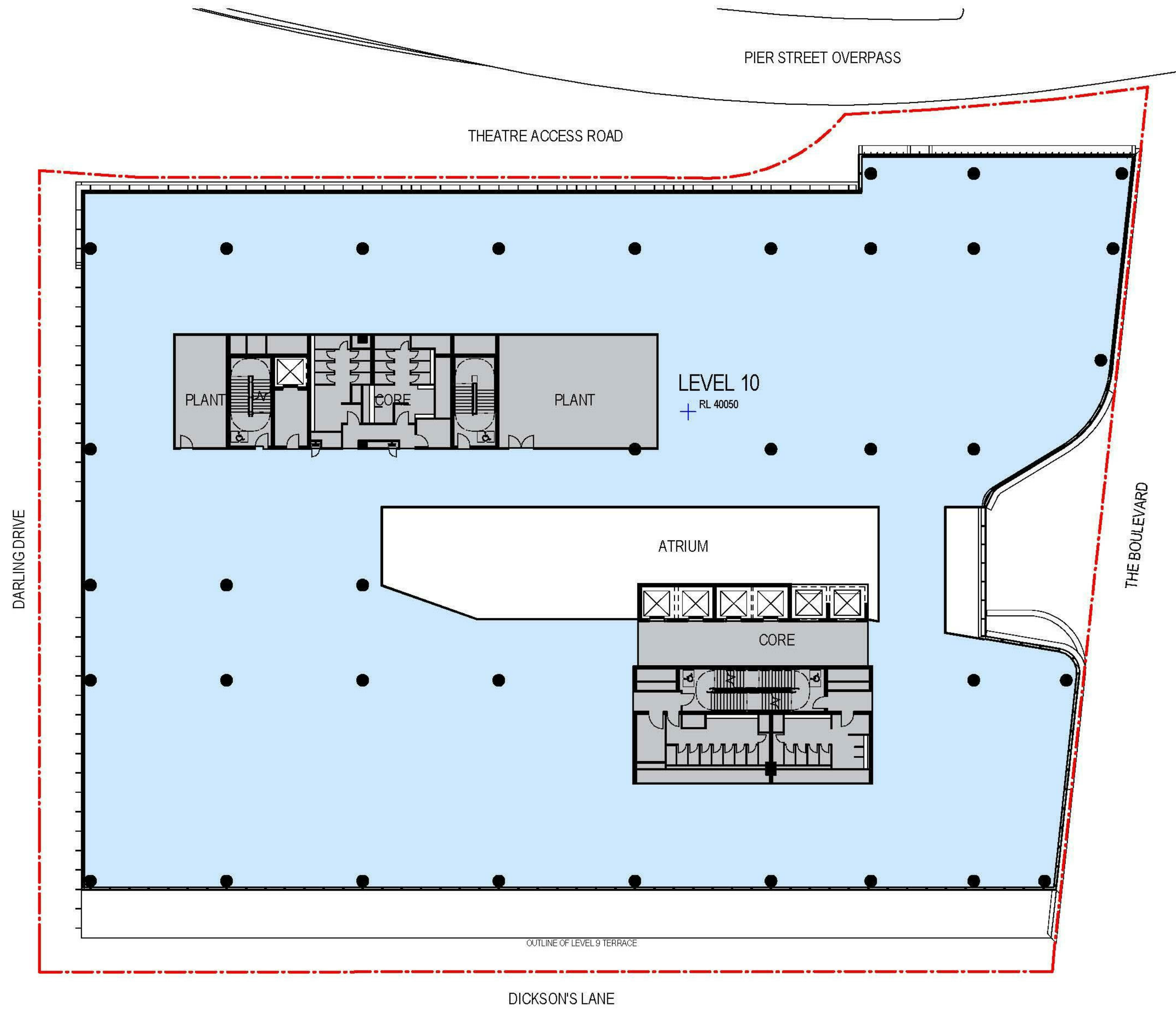
1 Level 10 - Approved SSD 6013 SCALE 1 : 250
