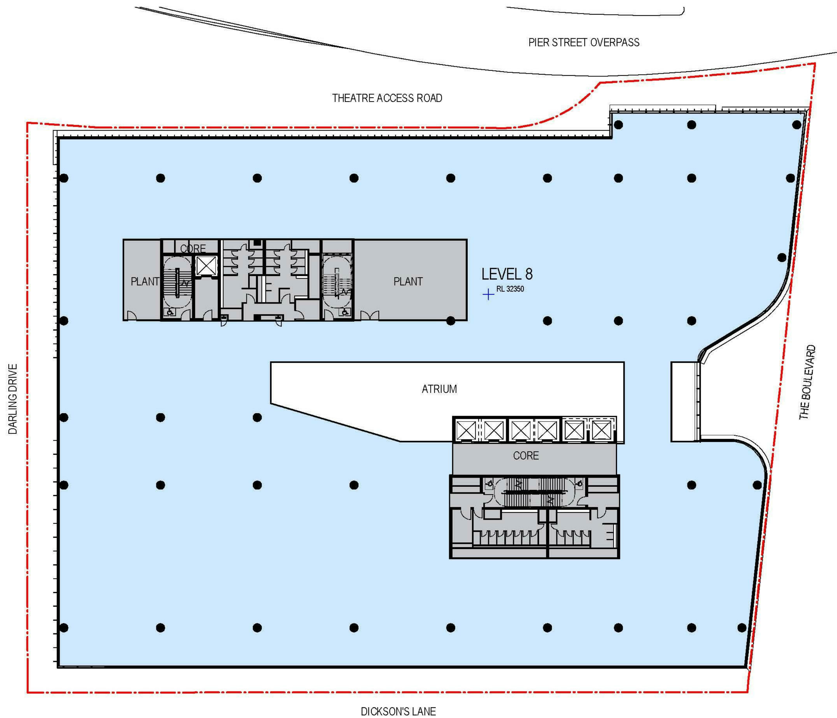
1 Level 8 - Approved SSD 6013 SCALE 1 : 250
