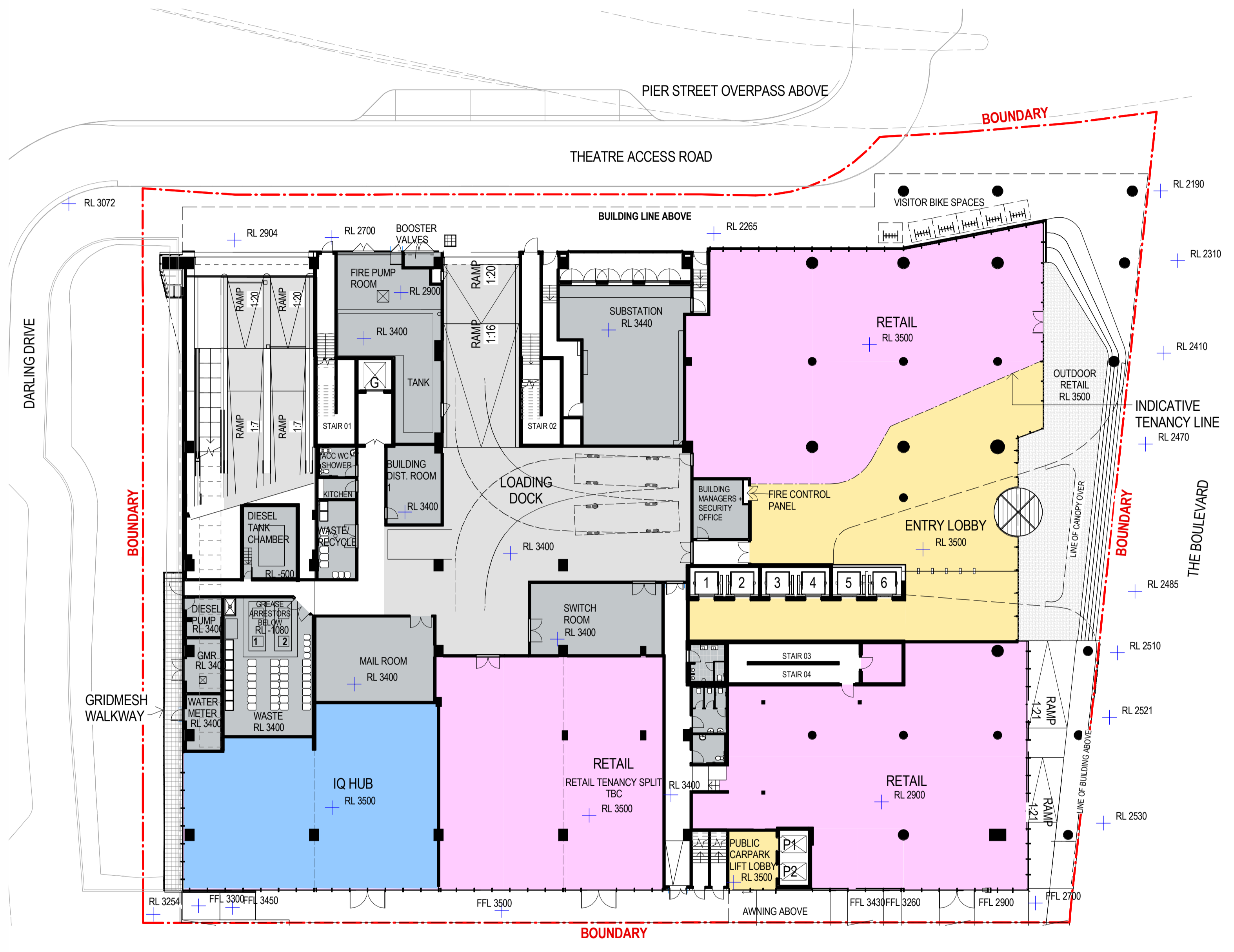
1 Ground Floor - Section 96 SCALE 1 : 250
