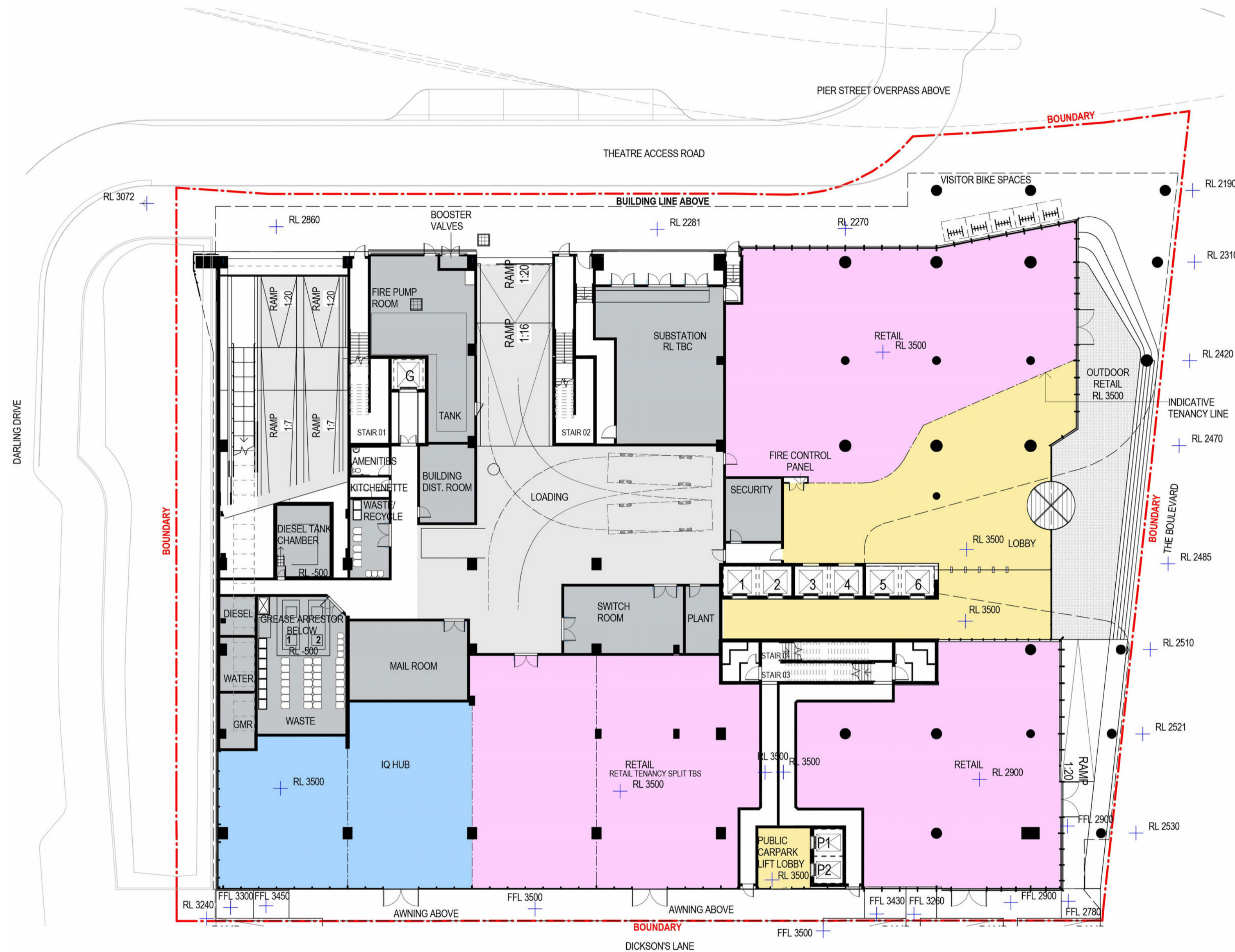
2 Ground Floor - Approved SSD 6013 SCALE 1 : 250
