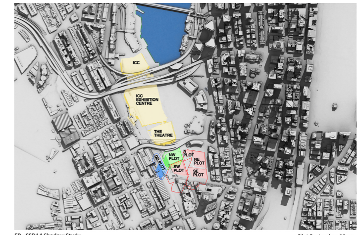
EP - SSDA4 Shadow Study 21st September, 11am ■ Shadows cast by SSDA4 building ↗ Parameter plan shadow NW Plot ■ Shadows cast by SSDA3 building ↘ Parameter plan shadow for DD plot ↖ Concept proposal parameter plan shadows for N, NE, SE + SW plots ■ Shadows cast by other buildings within the SICEEP site (PPP) ■ Shadows cast by Existing City Buildings
