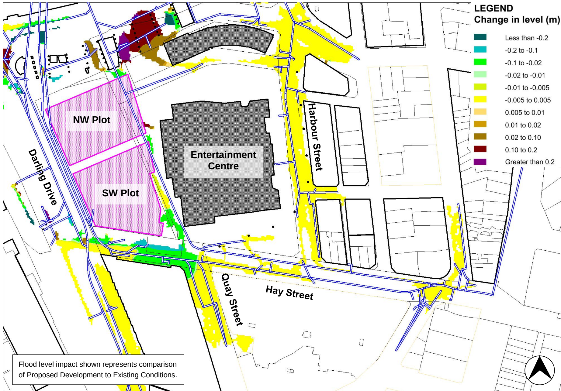
Figure D2 - 5 Year ARI Flood Level Impact 100mm gap under hoarding with 4m 2 inlet pit (50% blockage applied) with amplification and overland flow path
