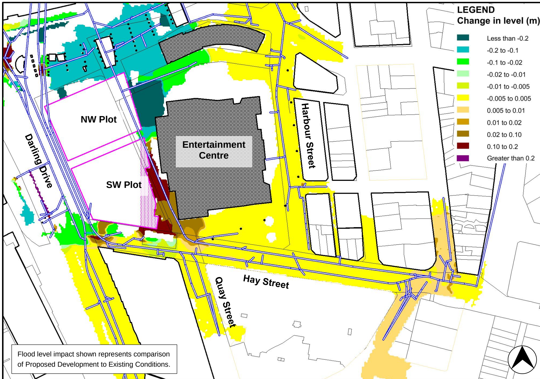
Figure D4 - 100 Year ARI Flood Level Impact 100mm gap under hoarding with 4m 2 inlet pit (50% blockage applied) with amplification and overland flow path
