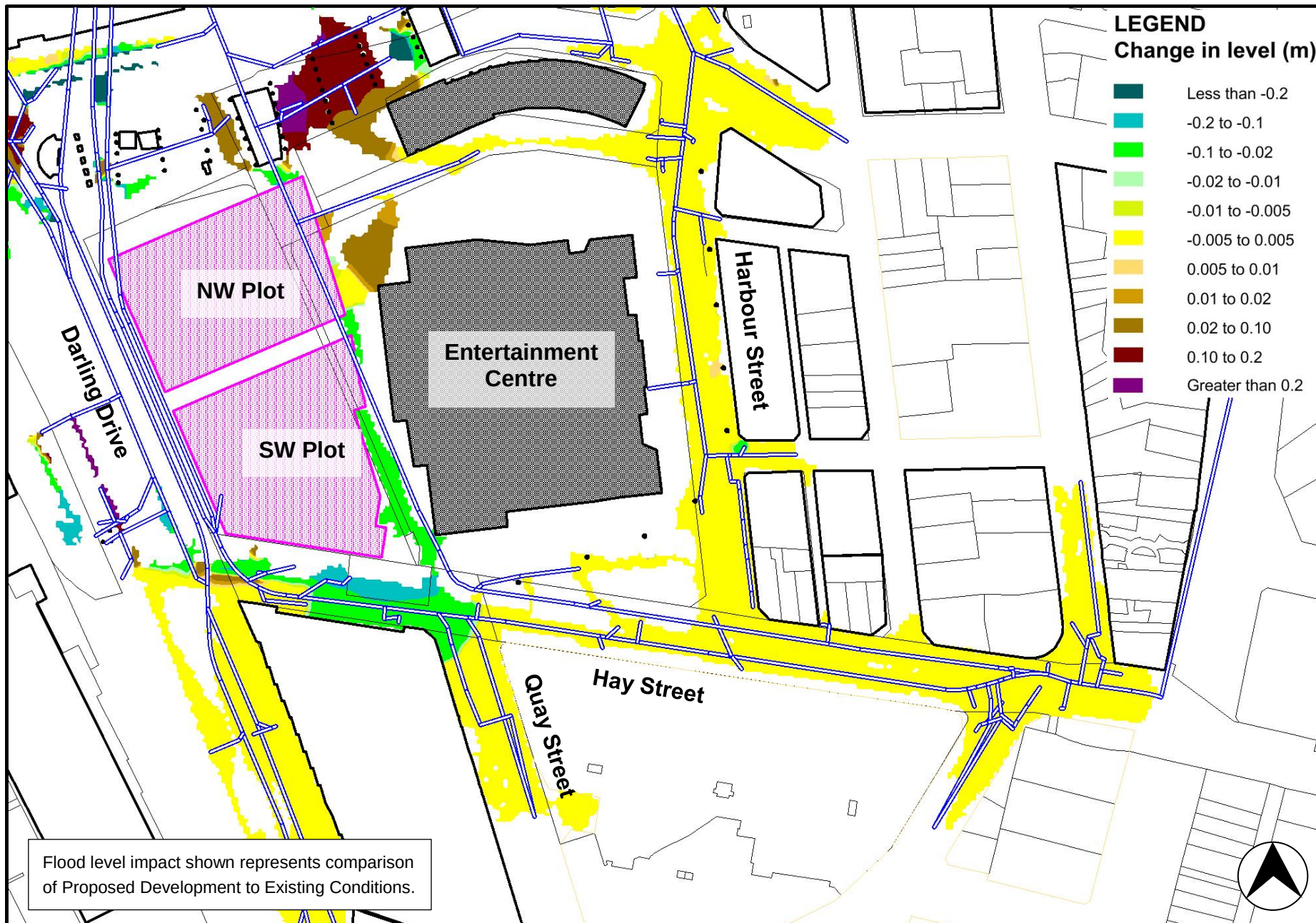
Figure D3 - 20 Year ARI Flood Level Impact 100mm gap under hoarding with 4m 2 inlet pit (50% blockage applied) with amplification and overland flow path
