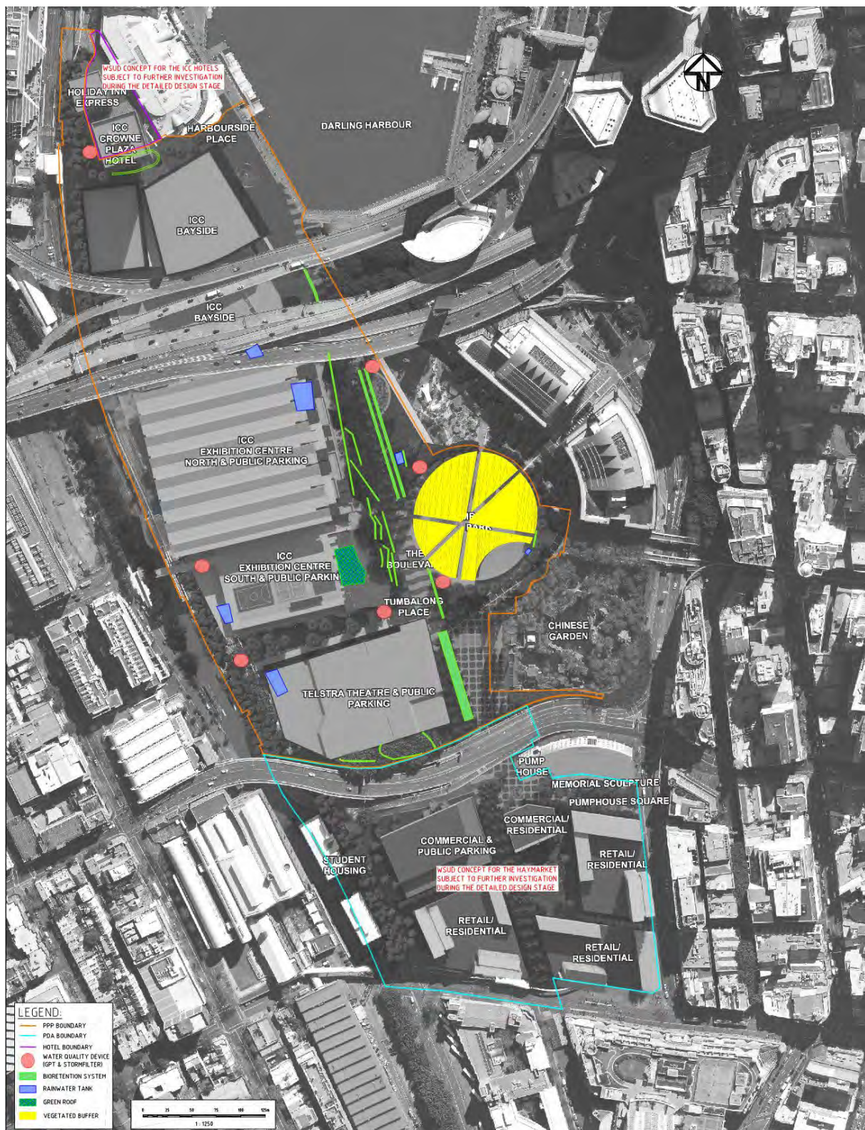
Figure 5-8 Locations of the treatment devices for the proposed Stormwater Quality Management Strategy ('Practical' Scenario) for the PPP development
