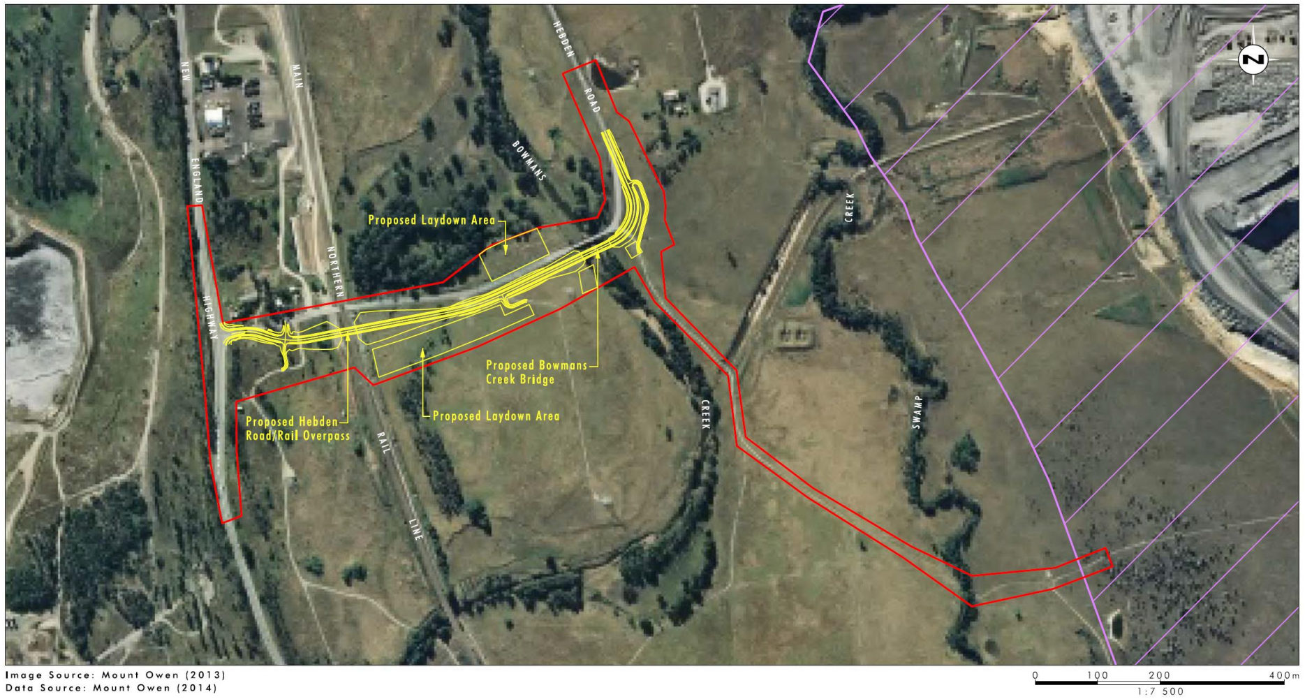
FIGURE 2.15 Hebden Road Upgrade Works Conceptual Design
