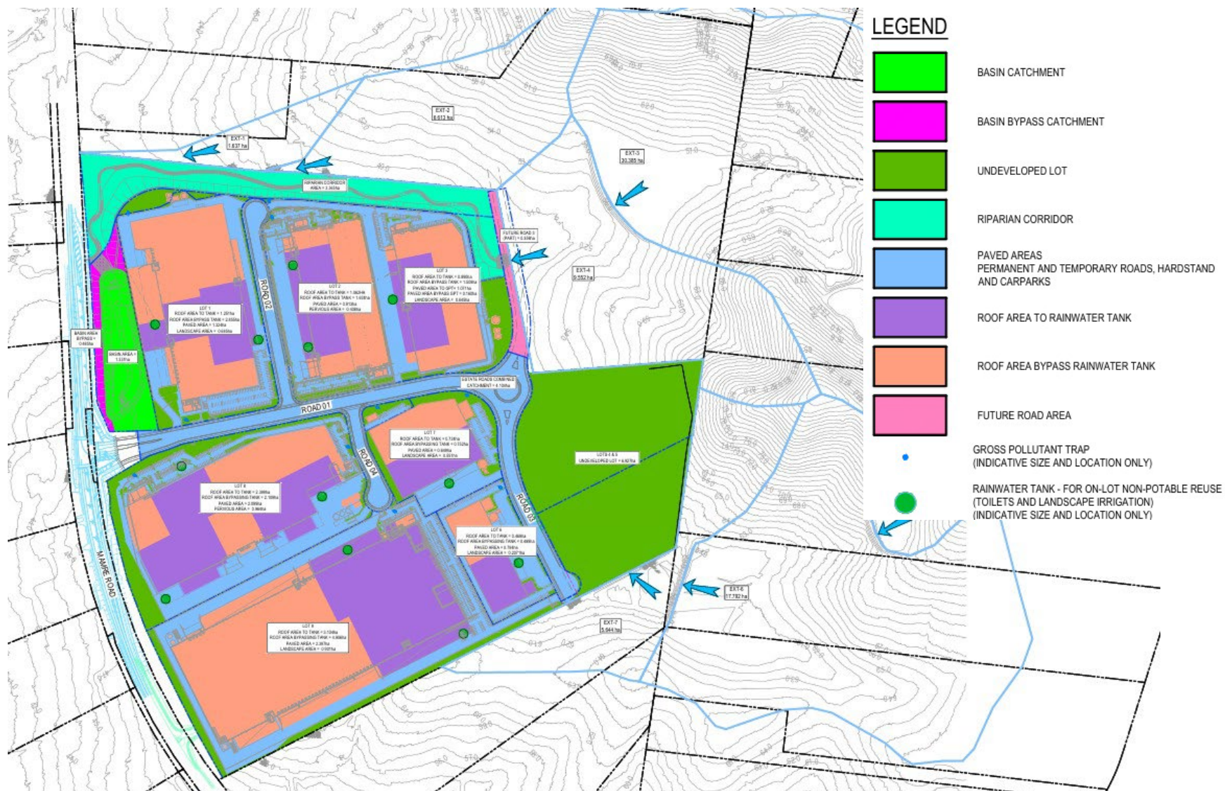
Figure 3: Stormwater Management A/E Site
