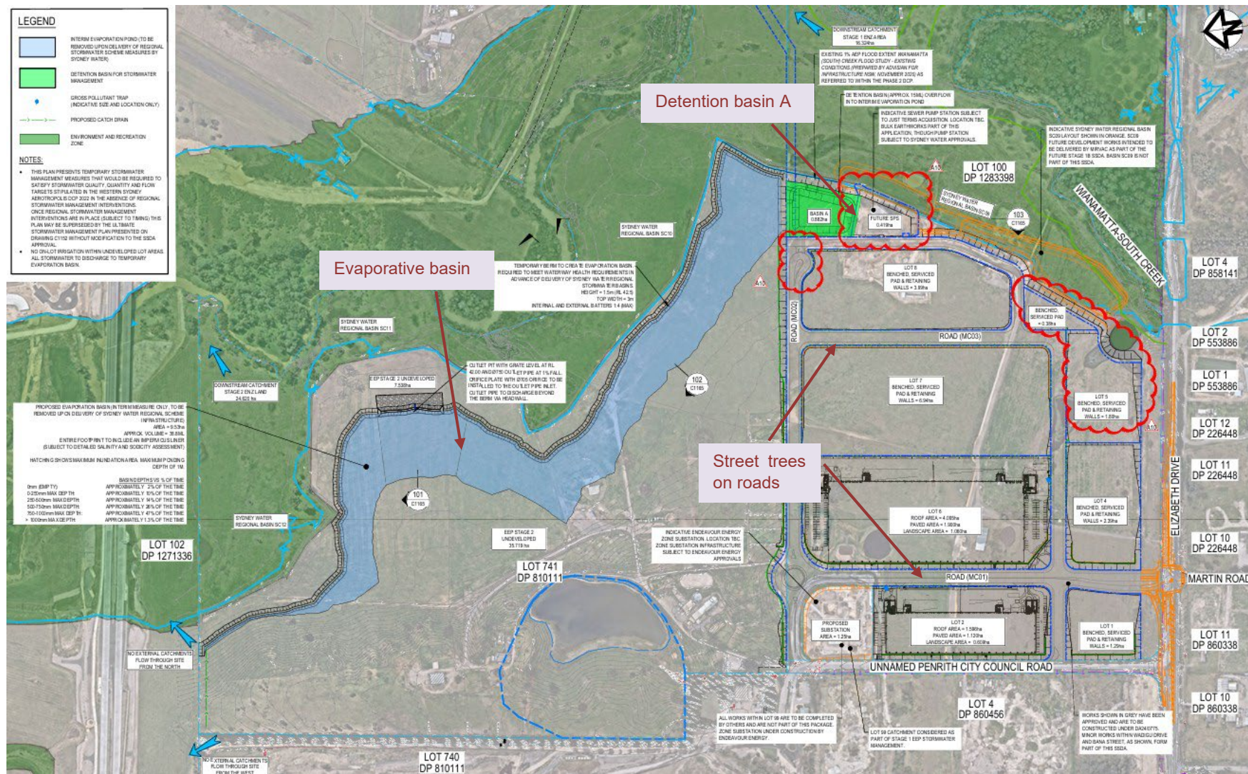
Figure 3A: Stormwater Management Plan EEP Site
