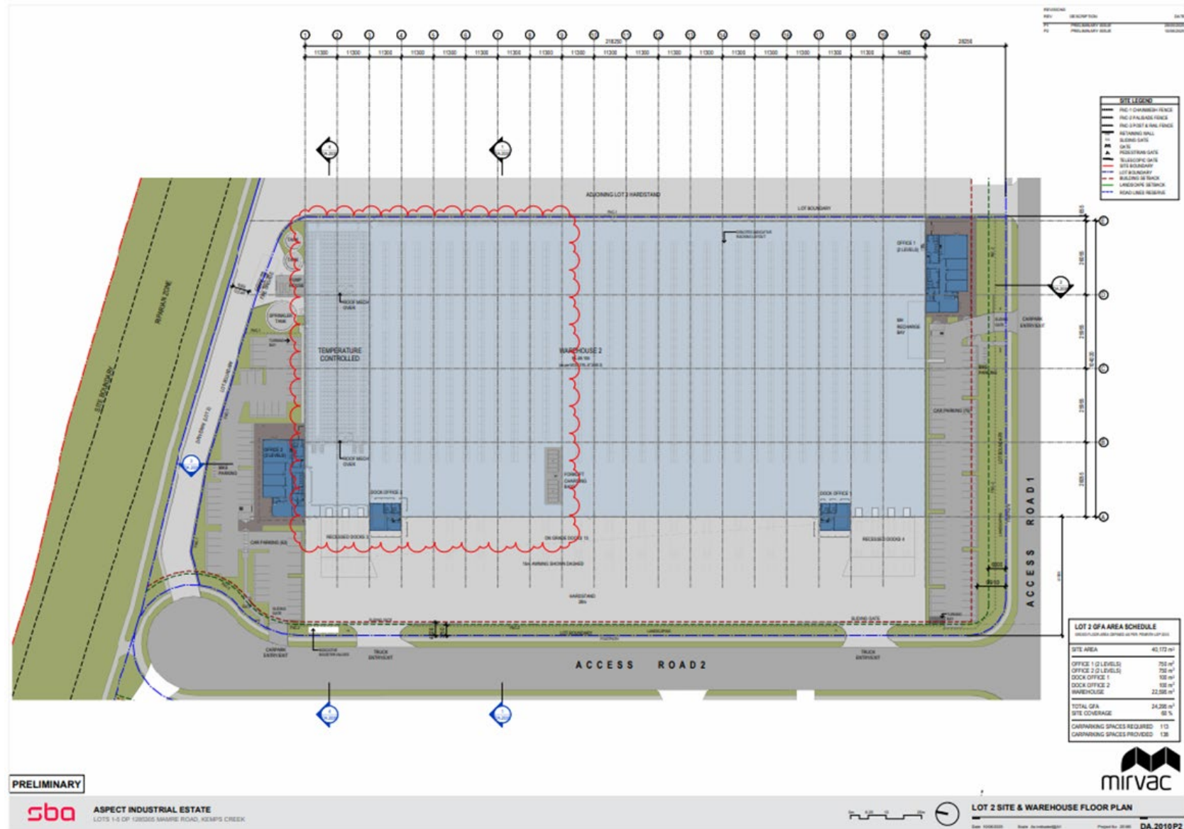
Figure 1: Site Plan
