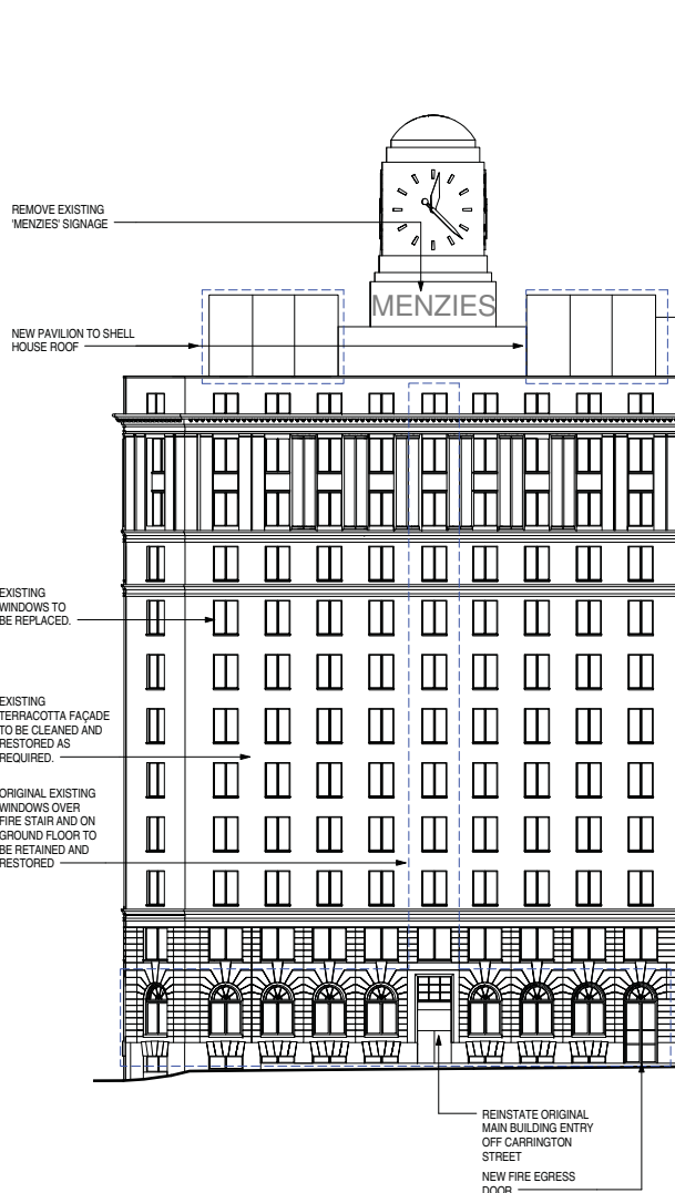
1 Carrington Street Elevation
