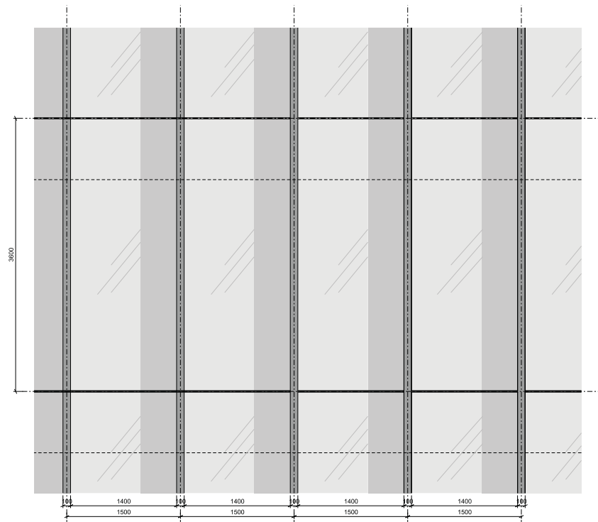
01 Typical Office Elevation
