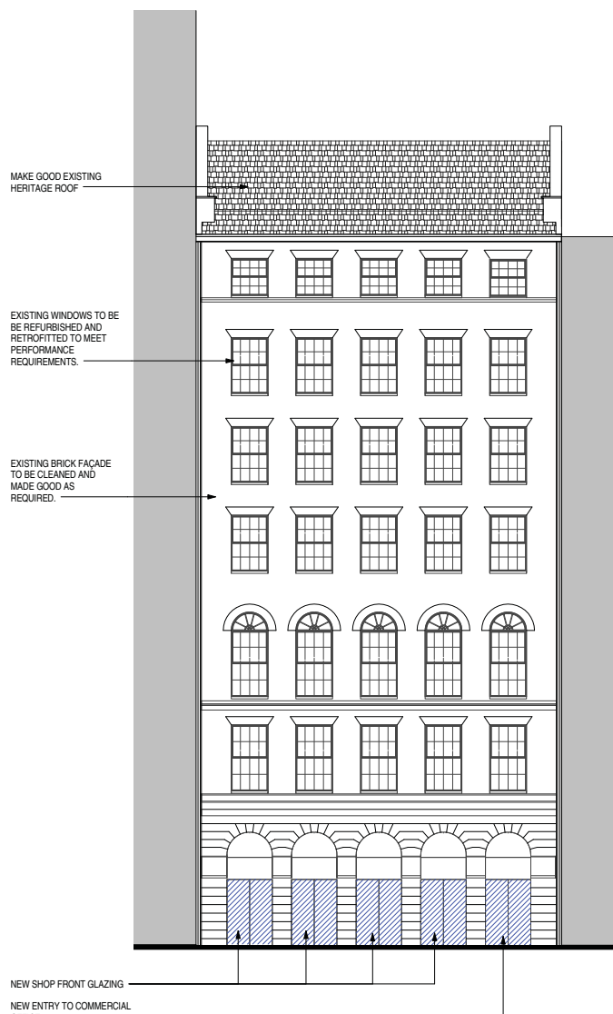
1 George Street Elevation Scale: 1 : 100
