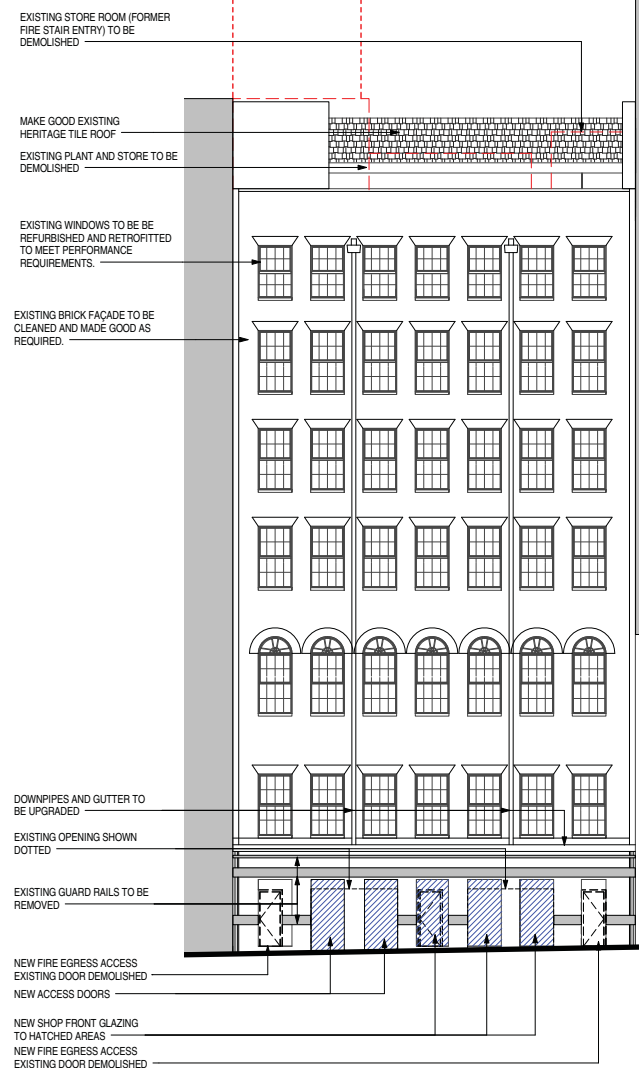
2 Wynyard Lane Elevation Scale: 1 : 100
