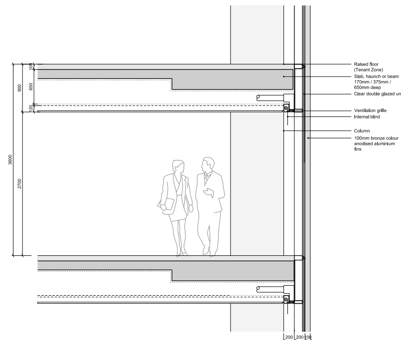
03 Typical office section
