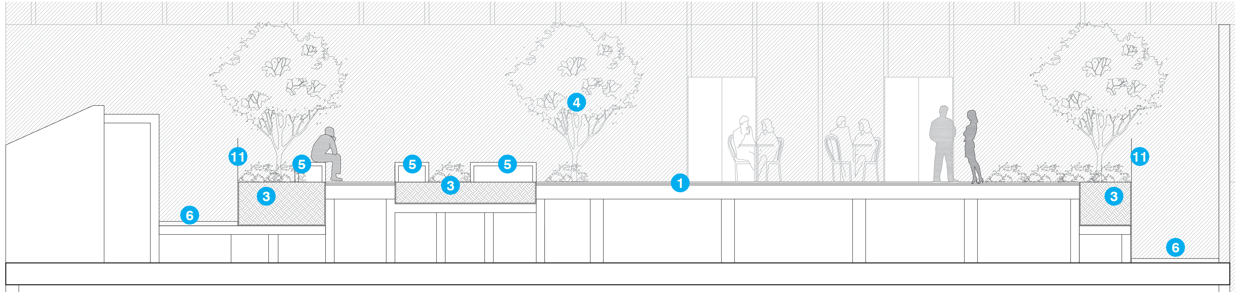
LEVEL 04 SECTION 1:50
