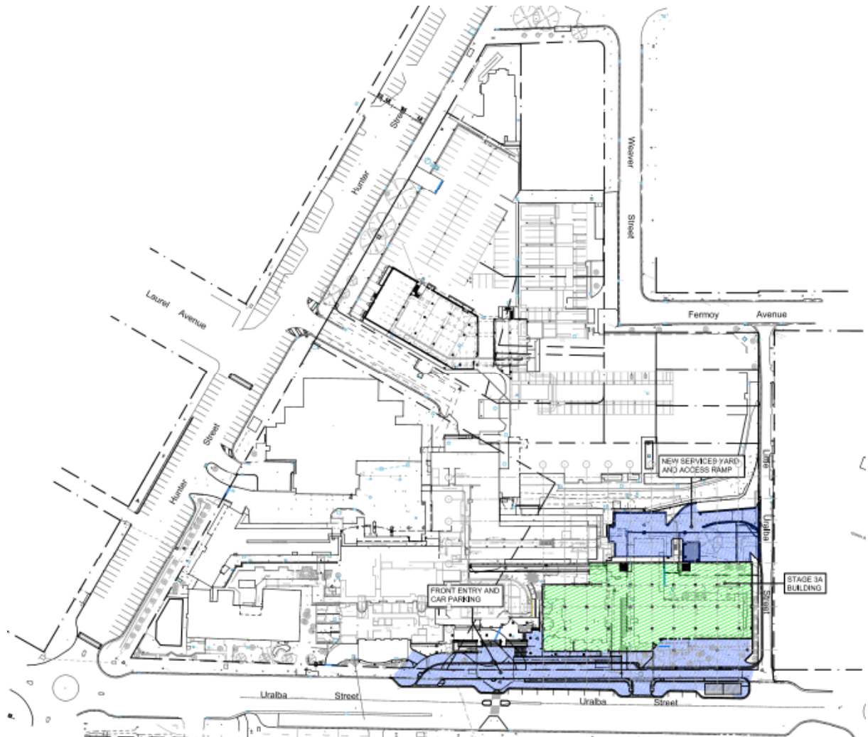
Figure 2 Site Plan
