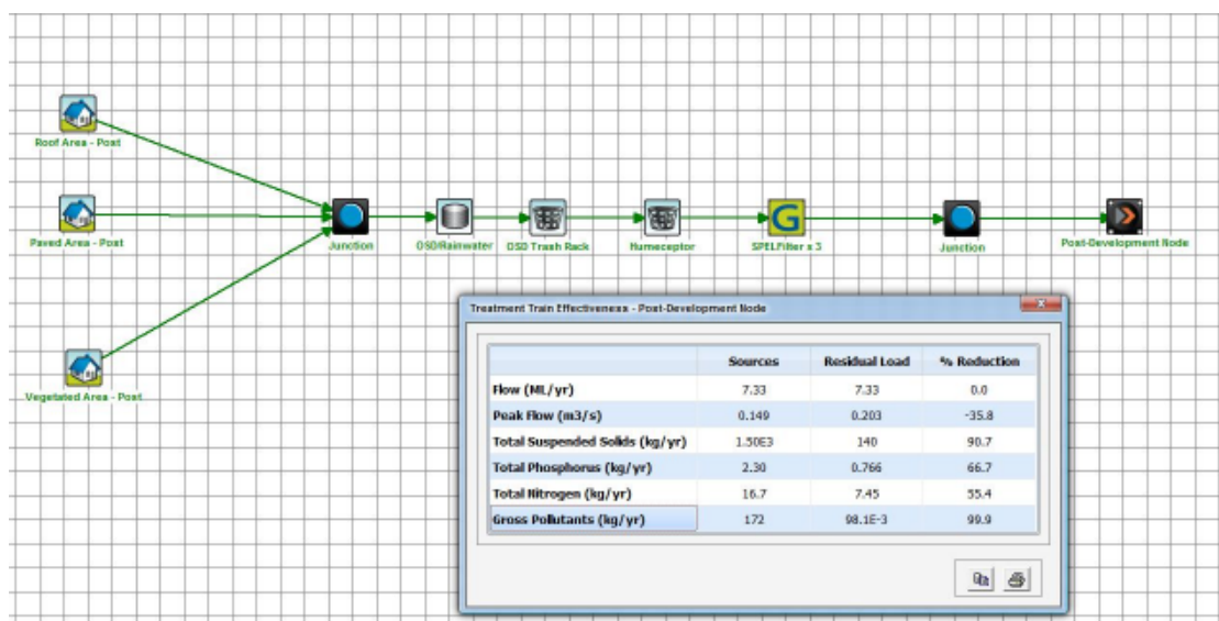
Figure 3 MUSIC Model Results
