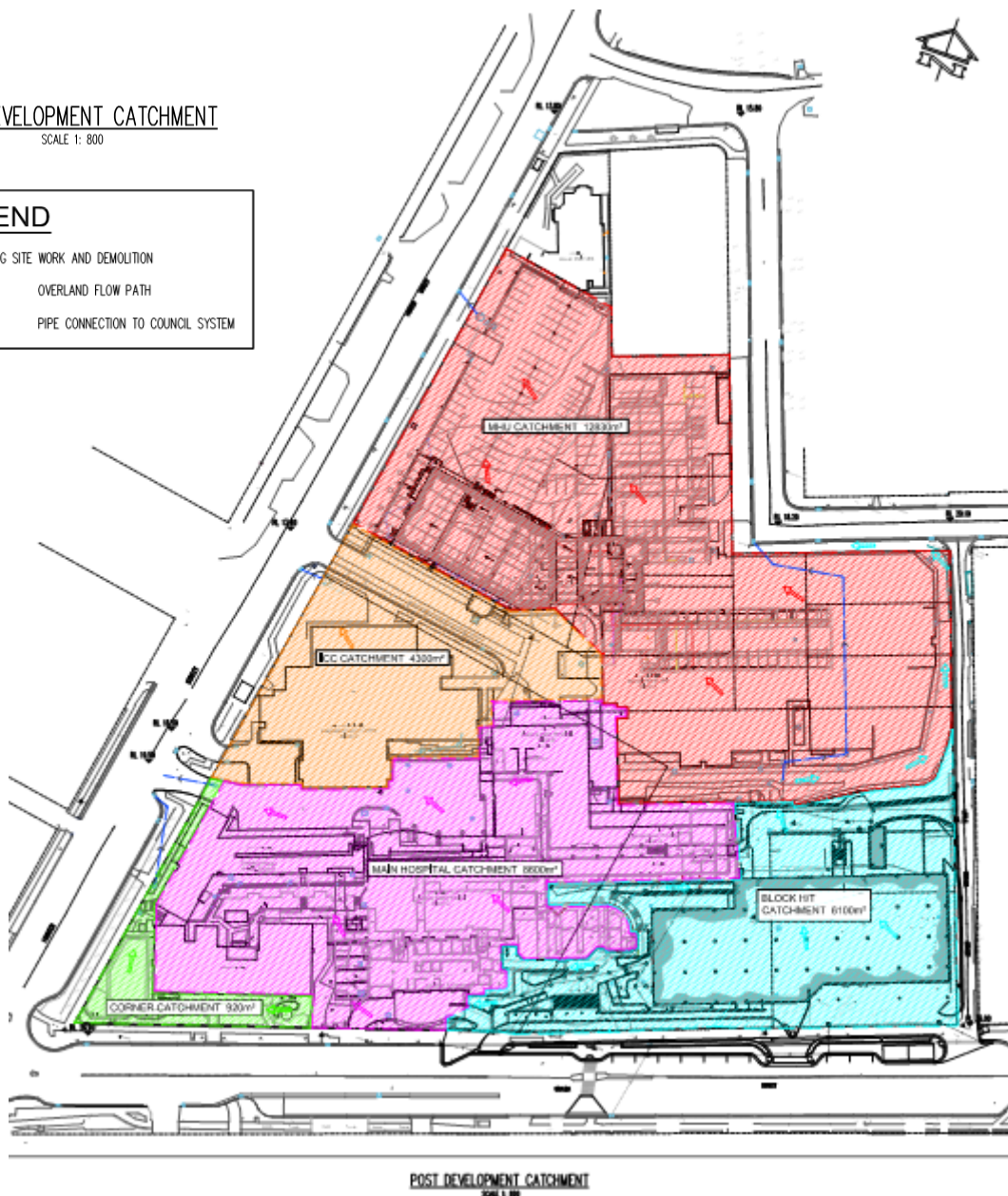
Figure 5 – Post-Development Catchment Plan
