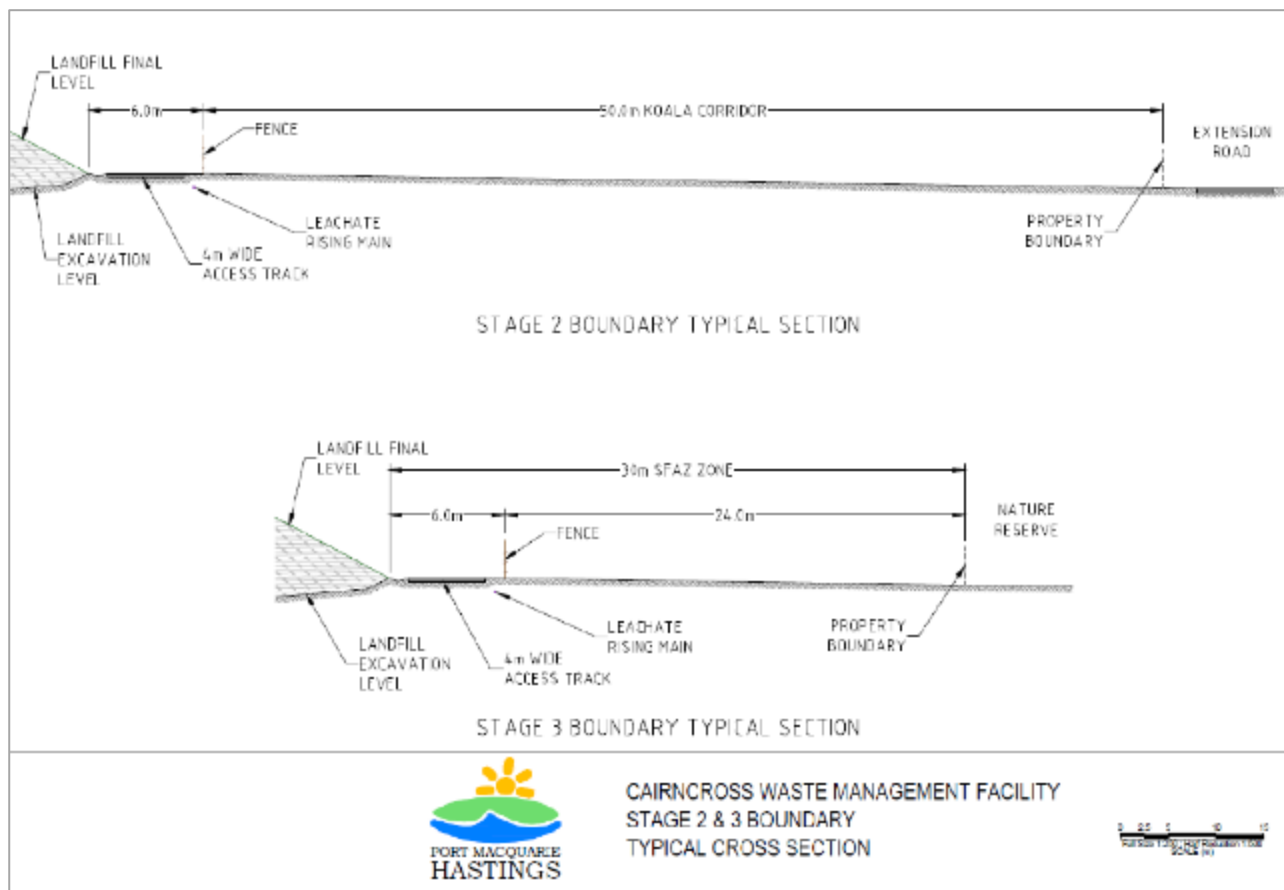
Figure 5-3: Stage 2 and 3 boundary typical cross section
