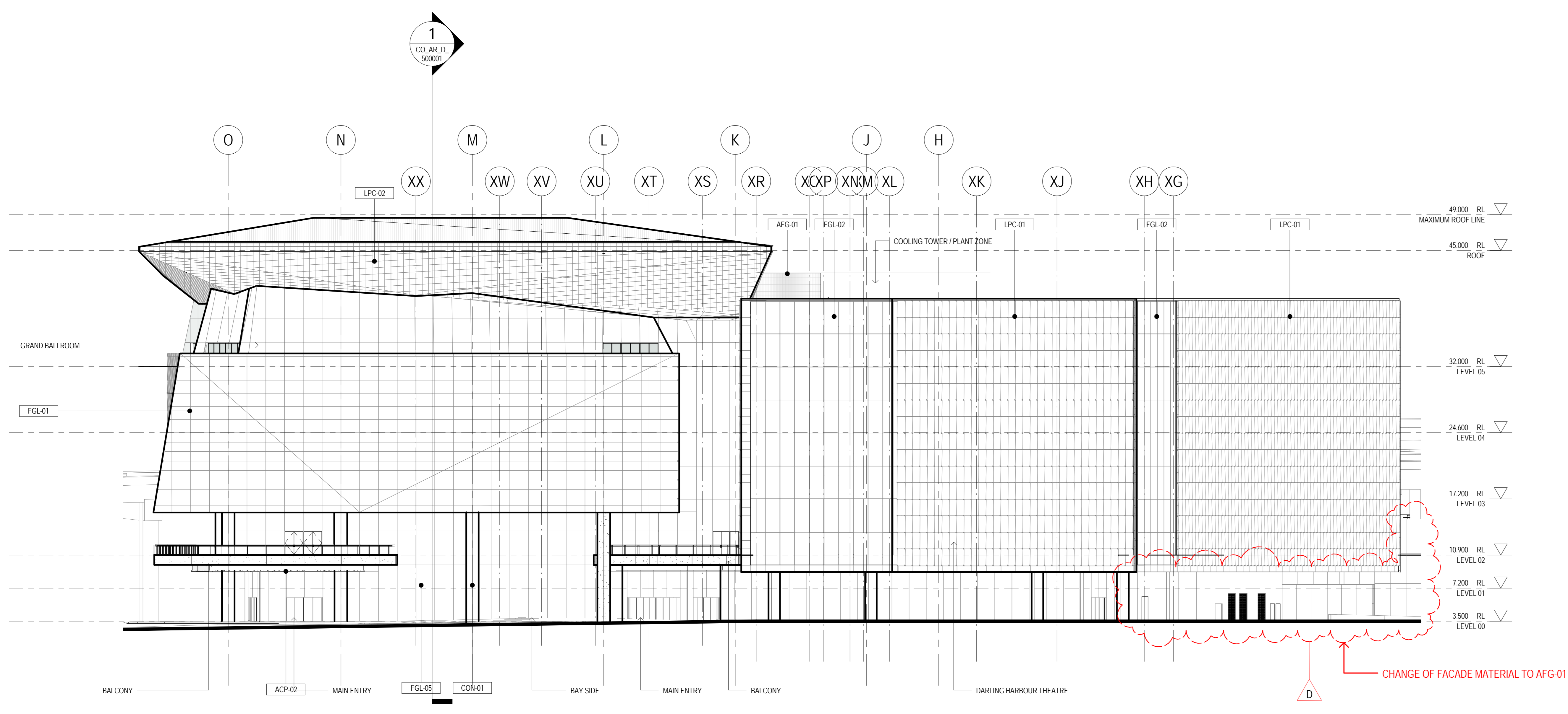
2 NORTHERN ELEVATION 1:250
