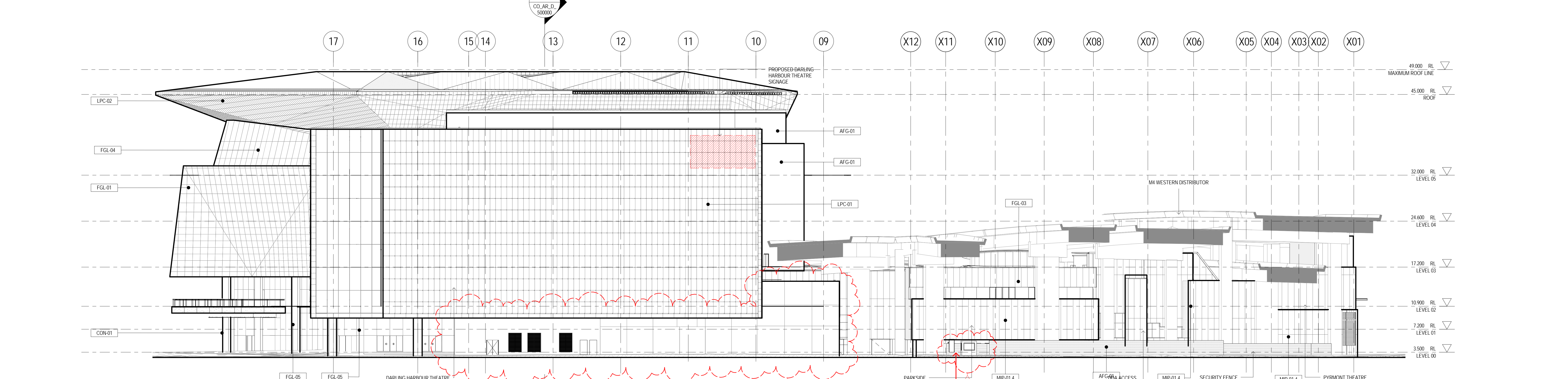
3 WESTERN ELEVATION 1:250
