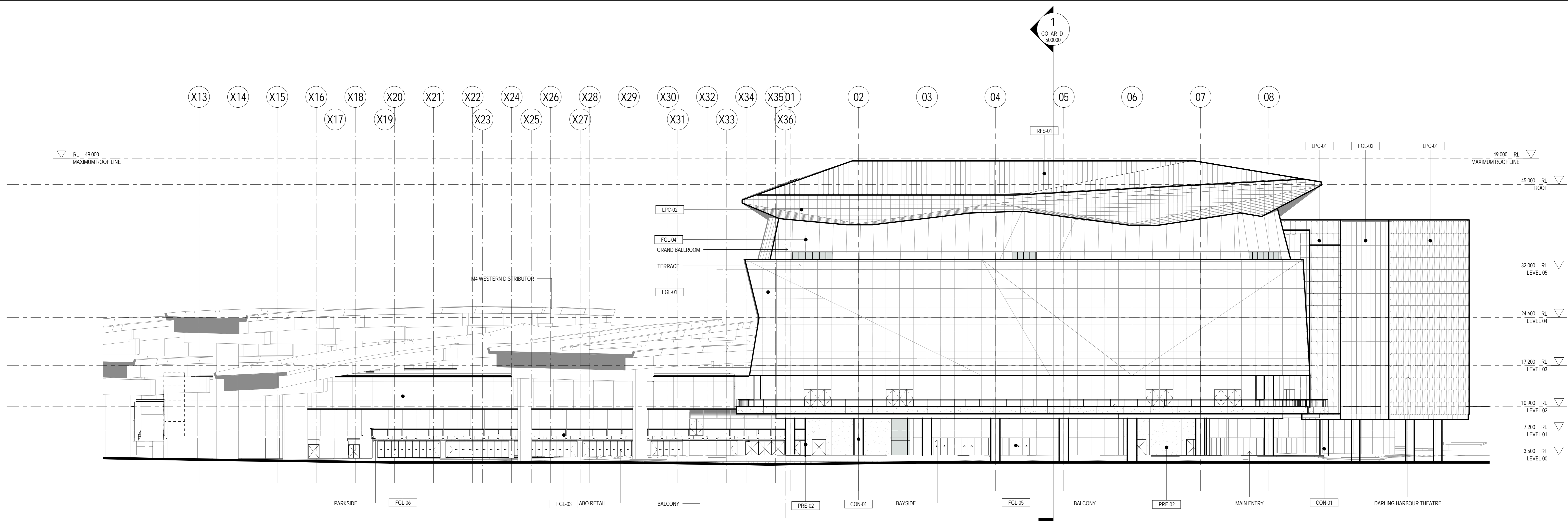
1 EASTERN ELEVATION 1:250
