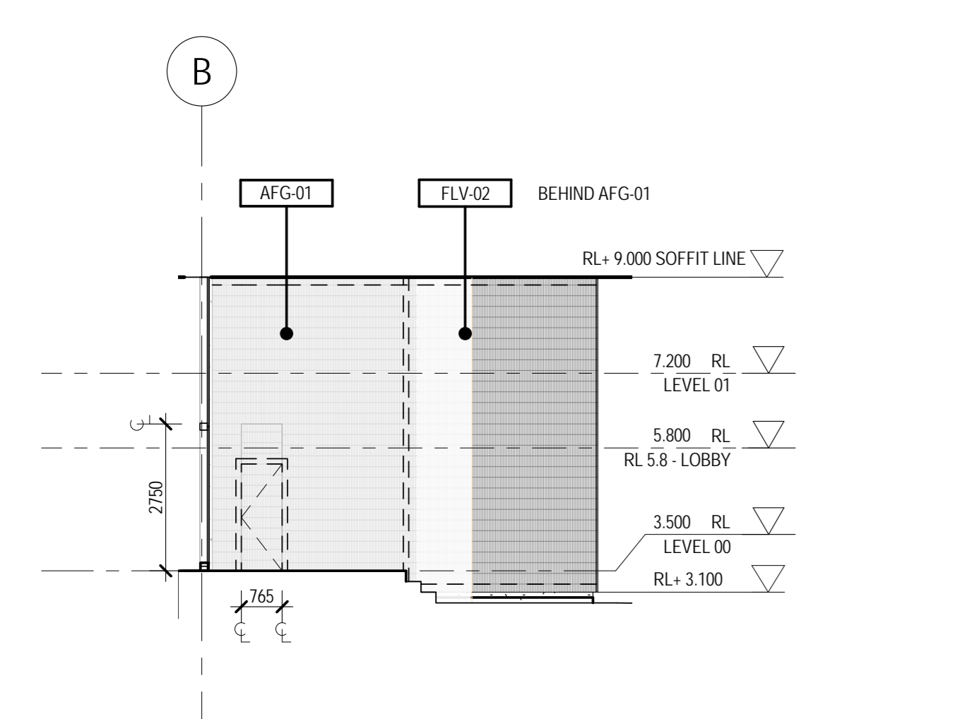
3 (DHT) ELEVATION - NORTH 3 CO.AR.D. 640030 1:100
