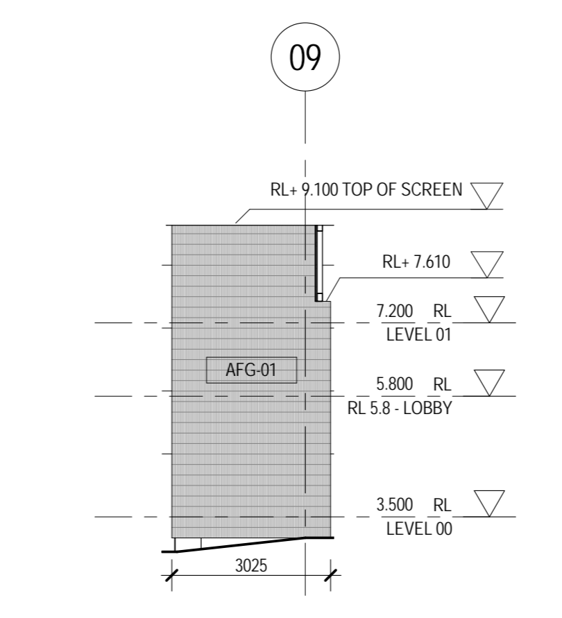
6 (DHT) ELEVATION - SOUTH RETURN CO.AR.D. 640030 1:100
