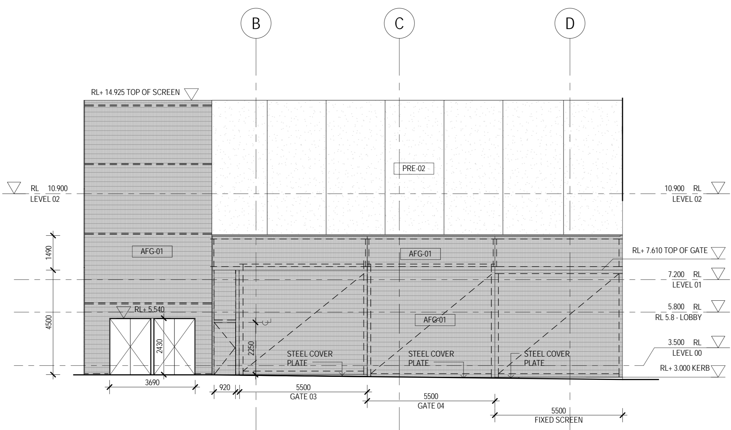
4 (DHT) ELEVATION - SOUTH 2 CO.AR.D. 640030 1:100
