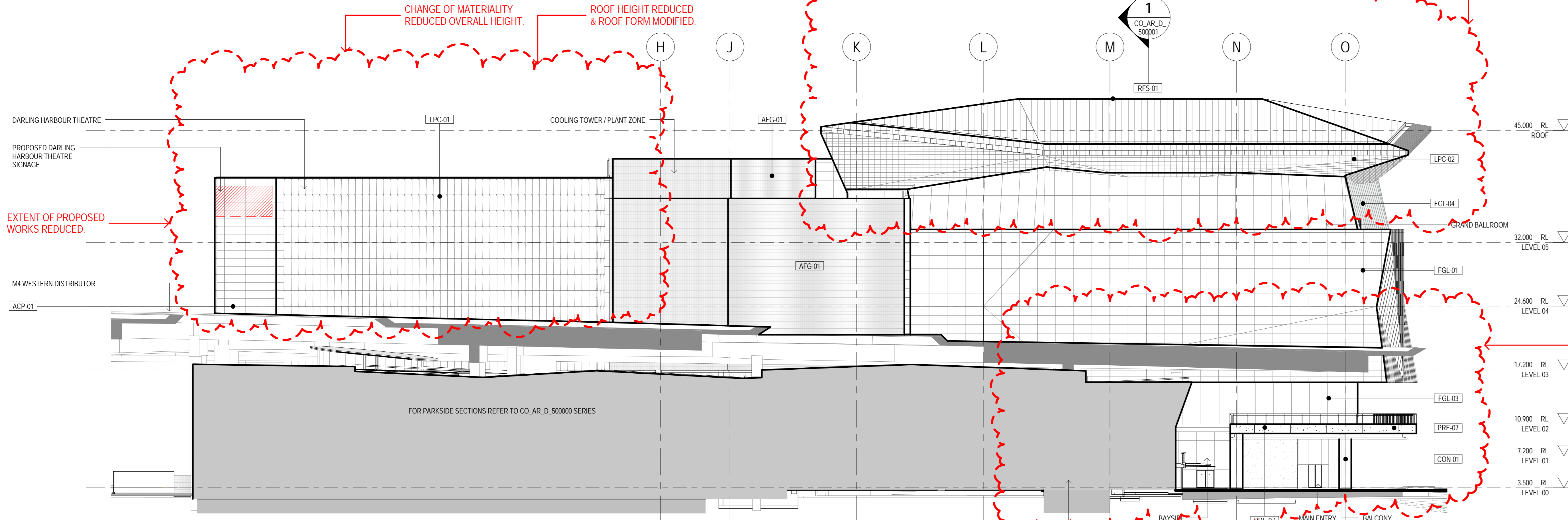
1 SOUTHERN ELEVATION CO_AR_D_400001 1:250
