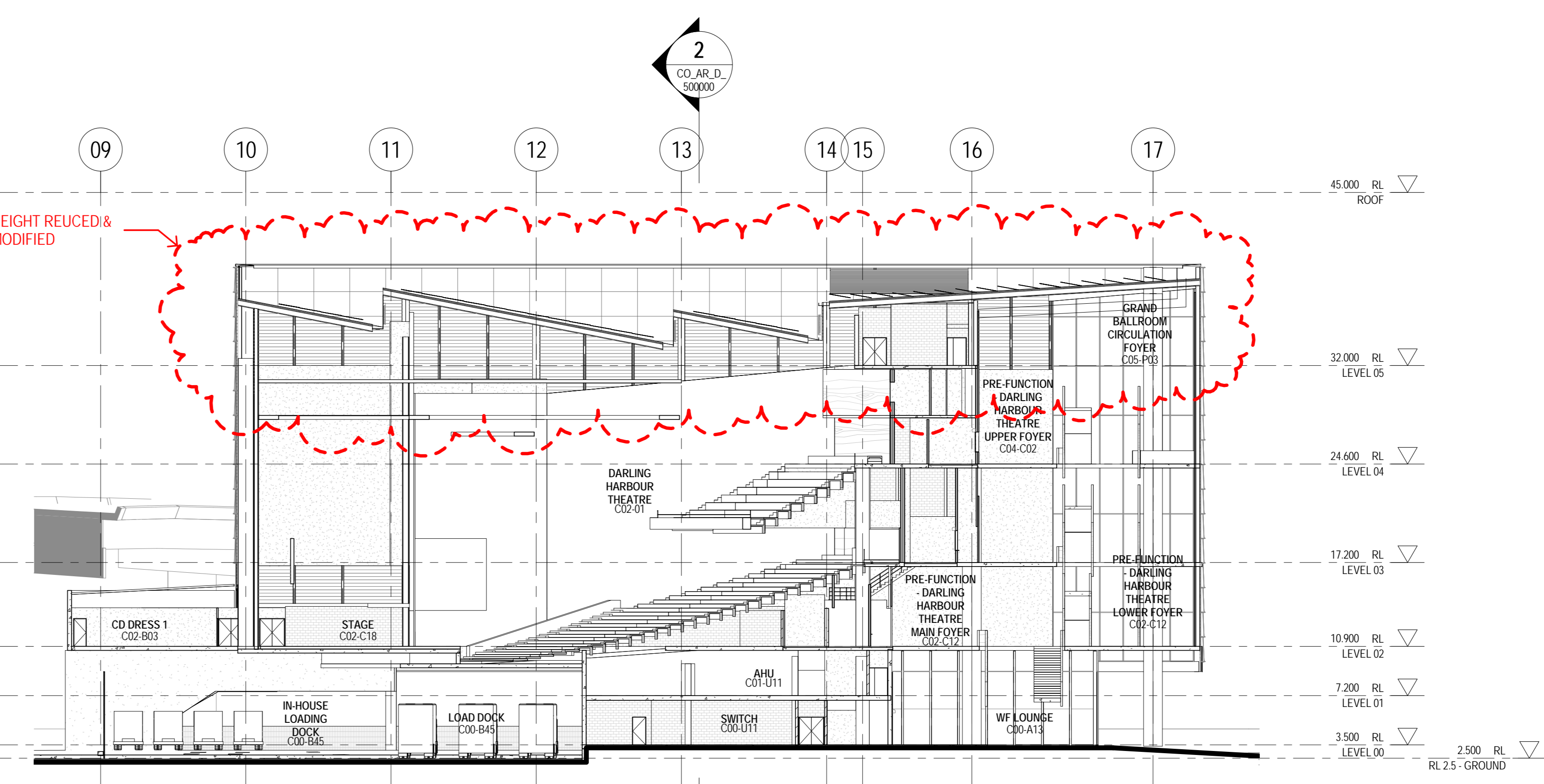
3 SECTION 2 - NORTH-SOUTH - THROUGH PLENIARY CO.AR.D. 1:250
