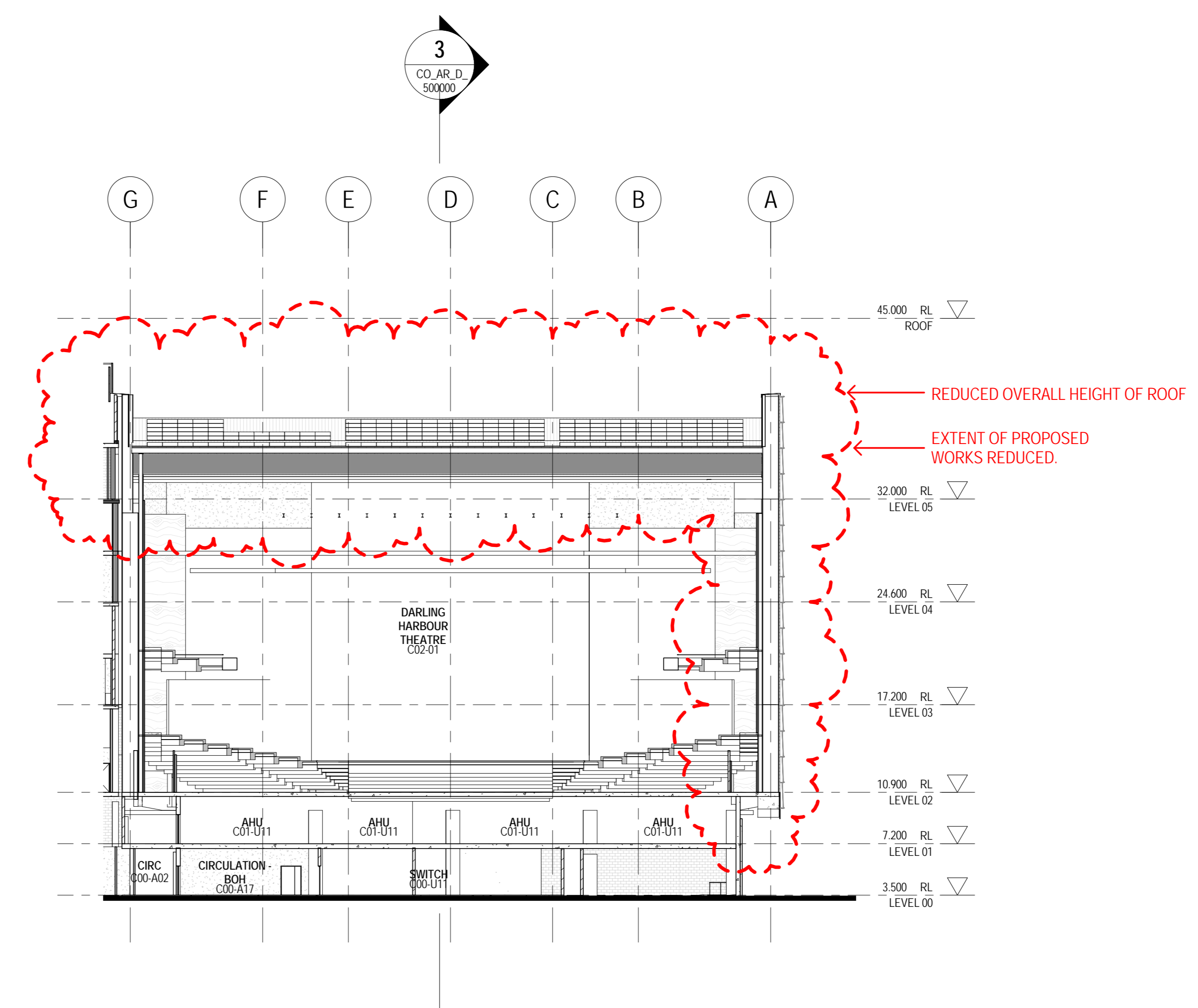
2 SECTION 1 - EAST-WEST - PLENIARY CO.AR.D. 1:250
