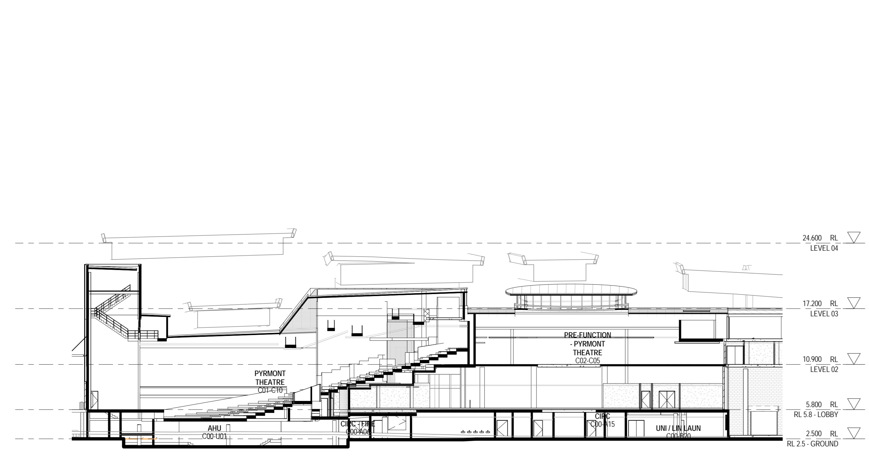
5 SECTION 2 - NORTH SOUTH - THROUGH PARKSIDE CO.AR.D. 1:250
