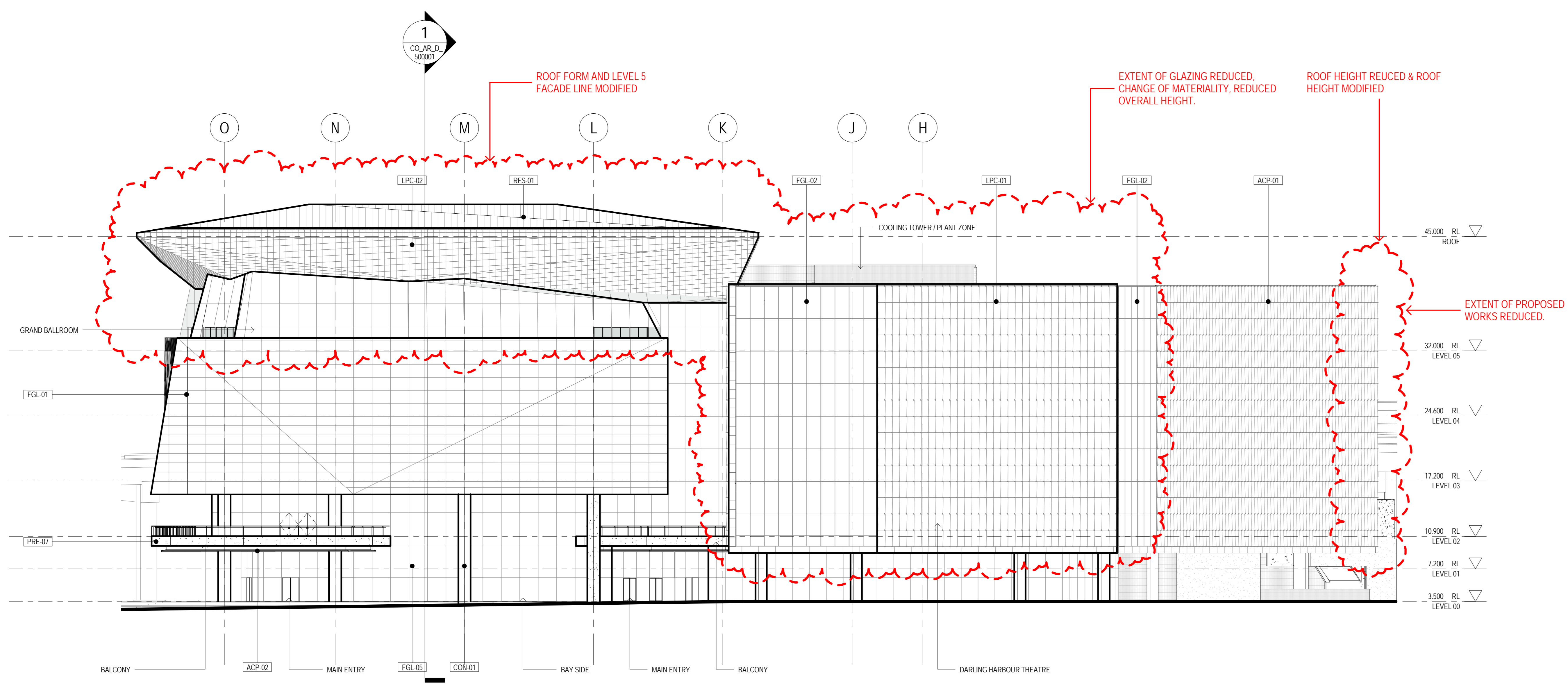
2 NORTHERN ELEVATION CO_AR_D_1:250
