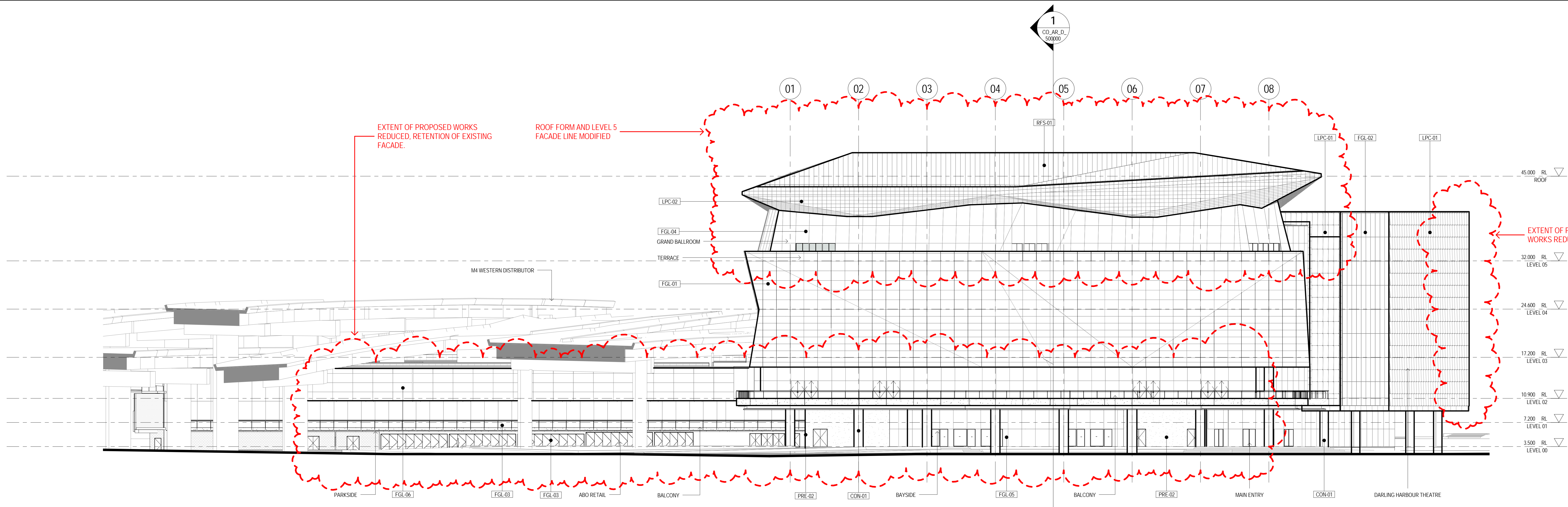
1 EASTERN ELEVATION CO_AR_D_1:250
