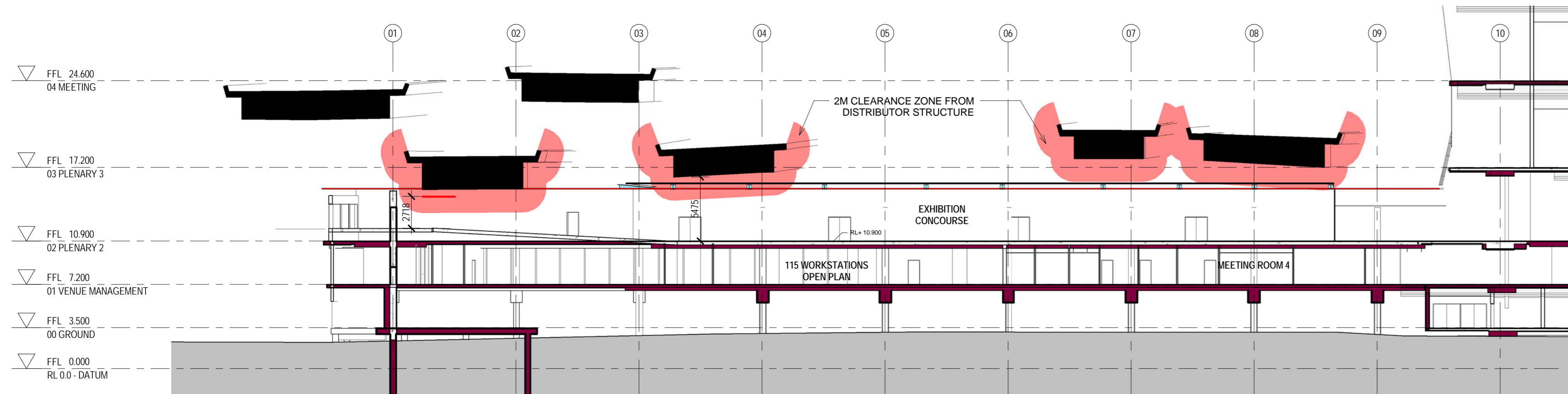
1 SECTION_CONCOURSE ROOF - WESTERN DISTRIBUTOR CONFLICT CO_AR.D / 1:250 CO_AR_SK_2005
