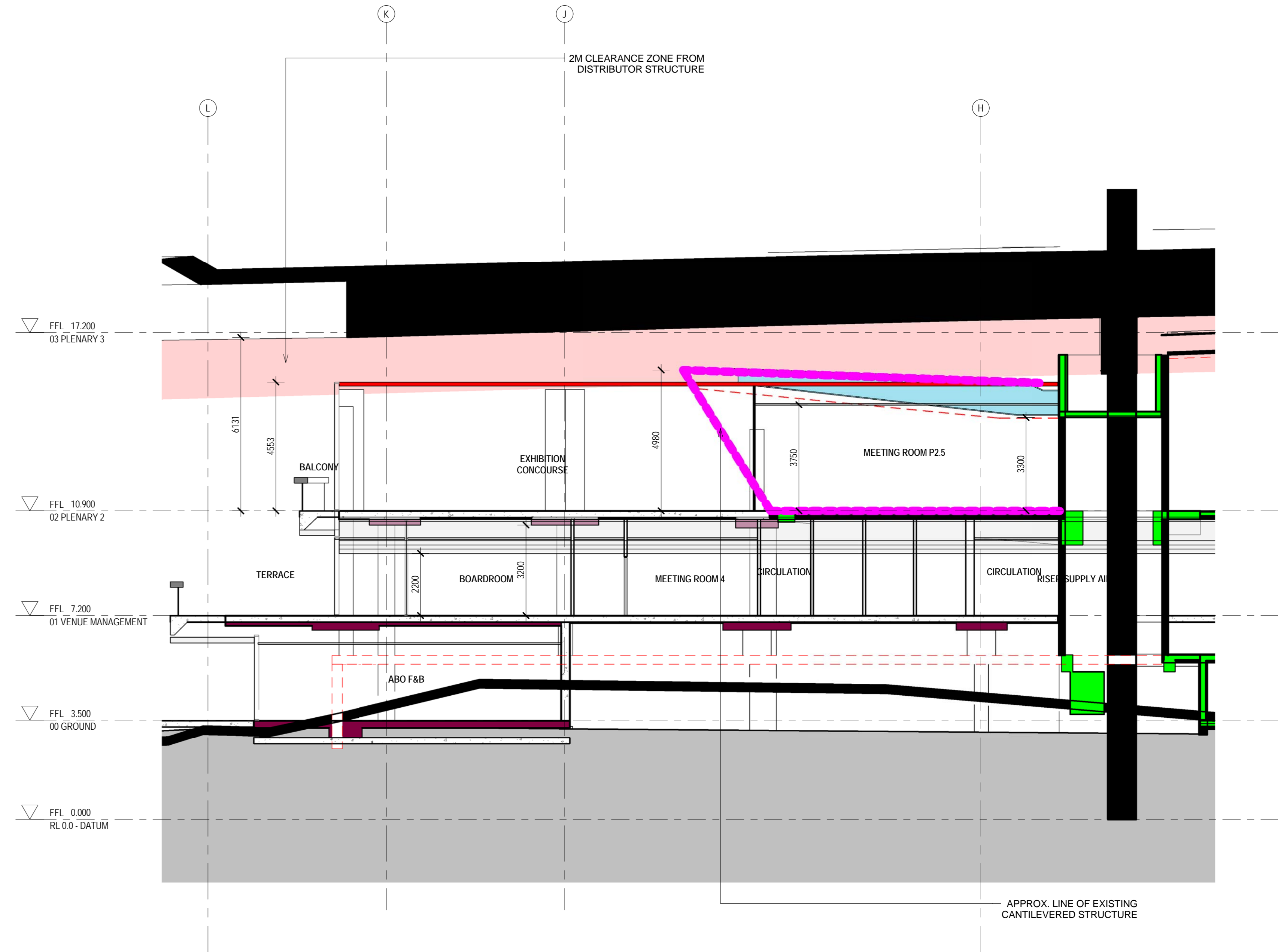
4 SECTION_CONCOURSE ROOF - EAST WEST 02 CO_AR.D / 1:100 CO_AR_SK_2005
