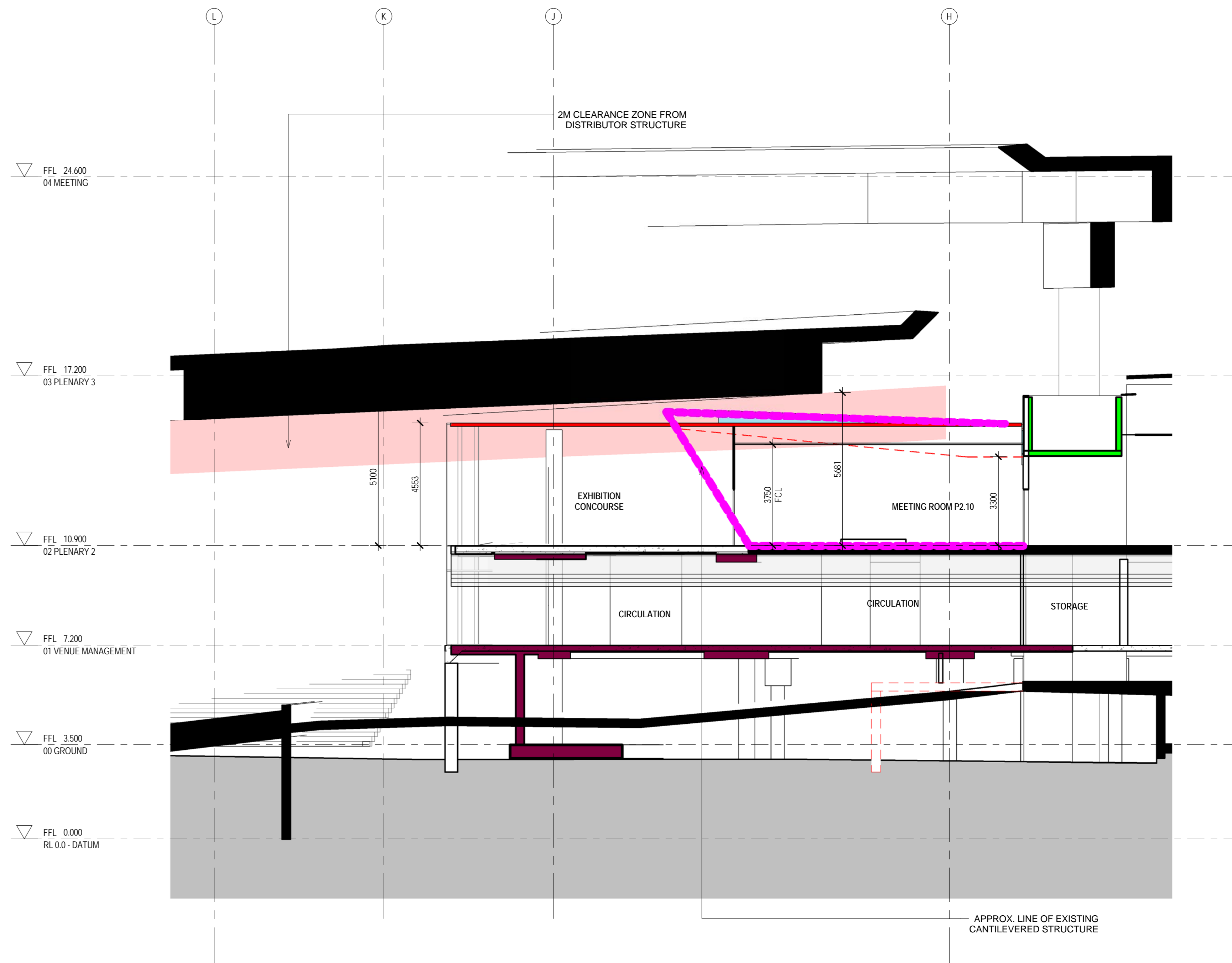
3 SECTION_CONCOURSE ROOF - EAST WEST 01 CO_AR.D / 1:100 CO_AR_SK_2005
