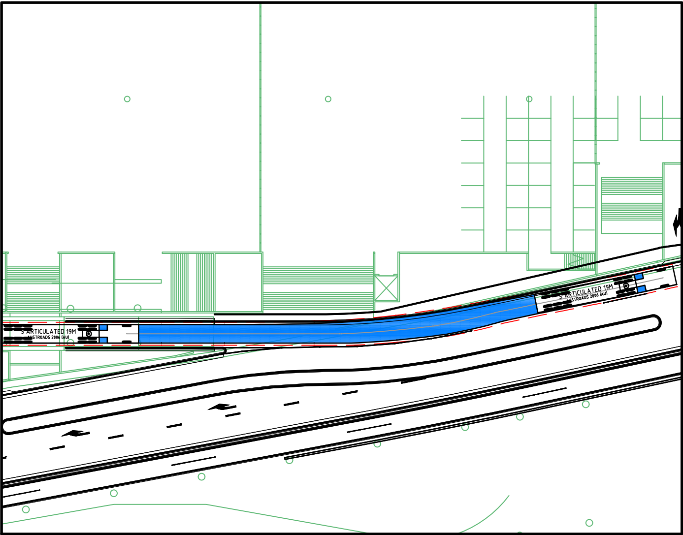
AUSTROADS 2006 19.0m SEMI - 01 ONTO DARLING DRIVE @ 05km/hr 1 : 500
