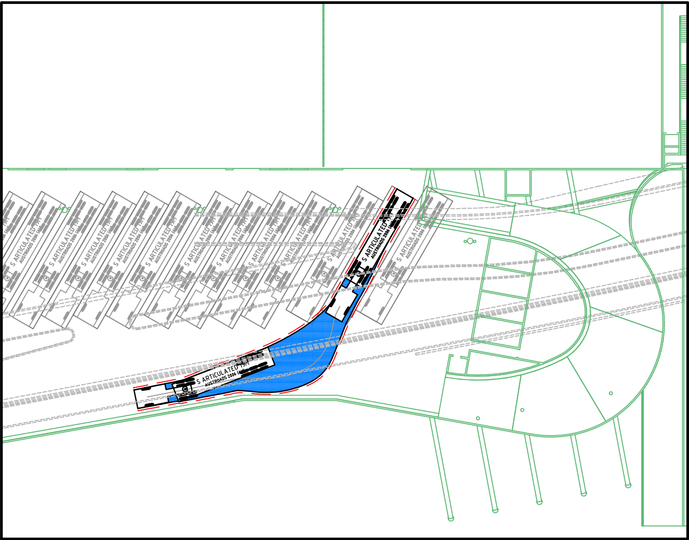
AUSTROADS 2006 19.0m SEMI - 02 IN @ 5km/hr 1 : 500
