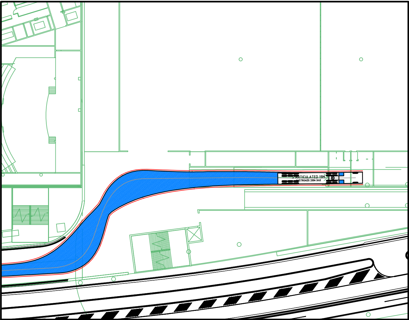
AUSTROADS 2006 19.0m SEMI - 01 IN FROM DARLING DRIVE @ 10km/hr 1 : 500
