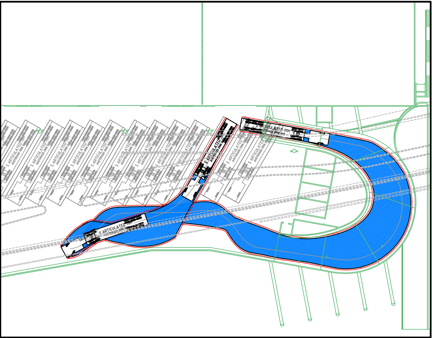
AUSTROADS 2006 19.0m SEMI - 03 IN @ 5km/hr 1 : 500
