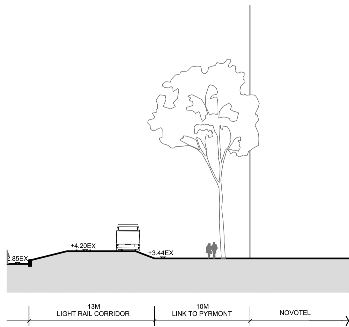
05 HARBOURSIDE PLACE 1:250 @ A1
