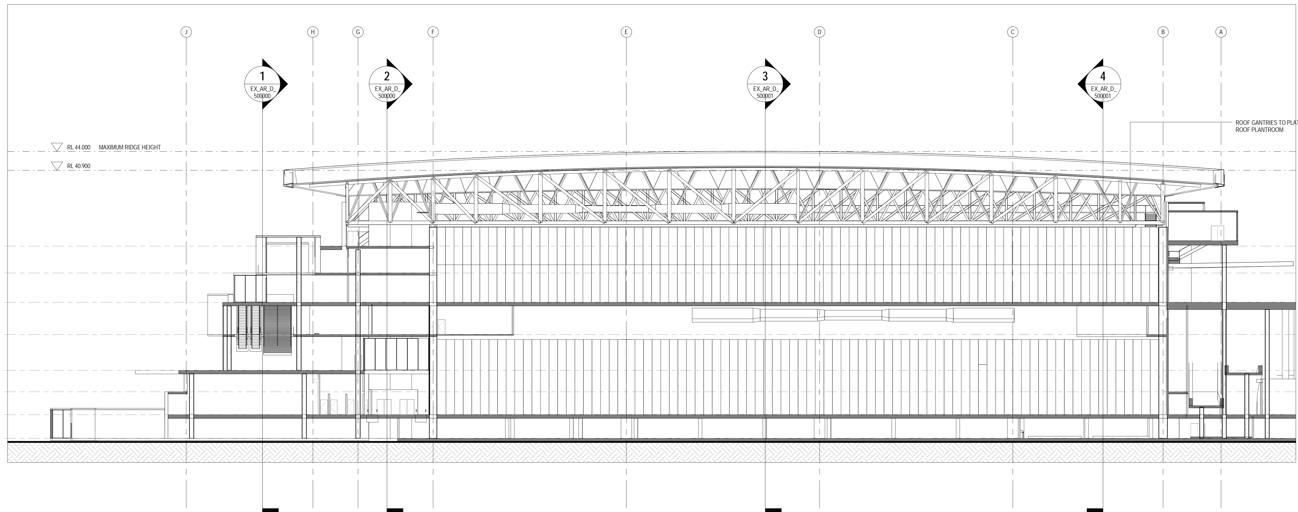
9 SECTION EX_AR_D_500000 1:250
