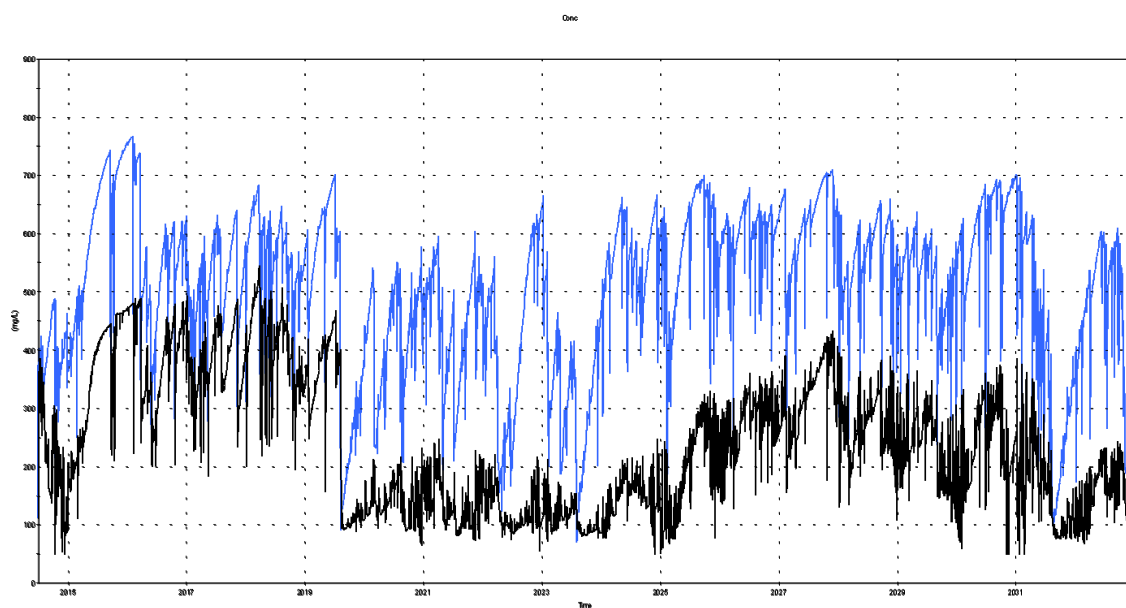
#035: Coxs River above Lake Lyell (Salinity, mg/L; at Energy Australia Monitoring Location, COX5)
