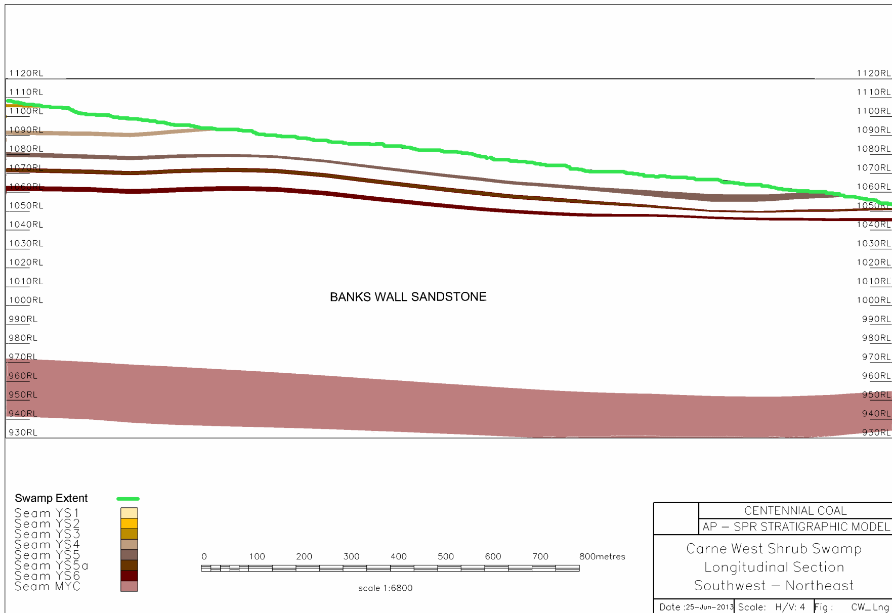
Figure 10 Longitudinal Stratigraphic Section of Carne West Shrub Swamp
